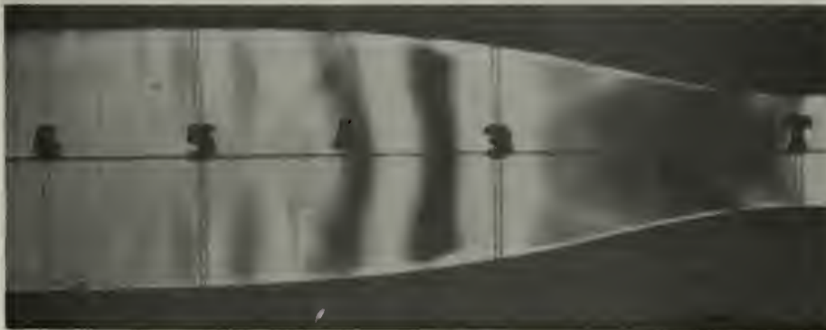
C. Vertical Knife. P_0 = 59.96 in. Hg. a., P_b = 30.73 in. Hg. a., T_n = 61.8^\circ F. Weaker Shock Moving Upstream as P_n is Reduced an Additional Amount.
