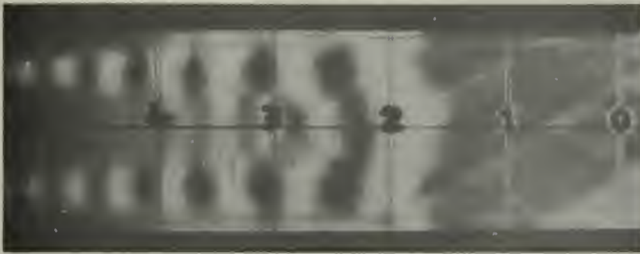
A. Vertical Knife. P_0 = 67.35 in. Hg. a., P_b = 30.45 in. Hg. a., T_0 = 66.3^\circ F. Diffuser Height 1.718 inches. Normal Shock at Station 12.
