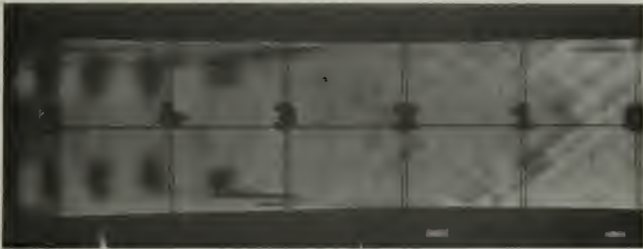
B. Vertical Knife. P_0 = 60.26 in. Hg. a., T_0 = 58.6^\circ F. Diffuser Height = 1.40 in. Area has been Increased 0.005 Square Inches Compared to Figure 16 A, and Shock has been Blown Through Diffuser Nozzle. Pressure Could be Reduced more to move Shock towards the Throat.
