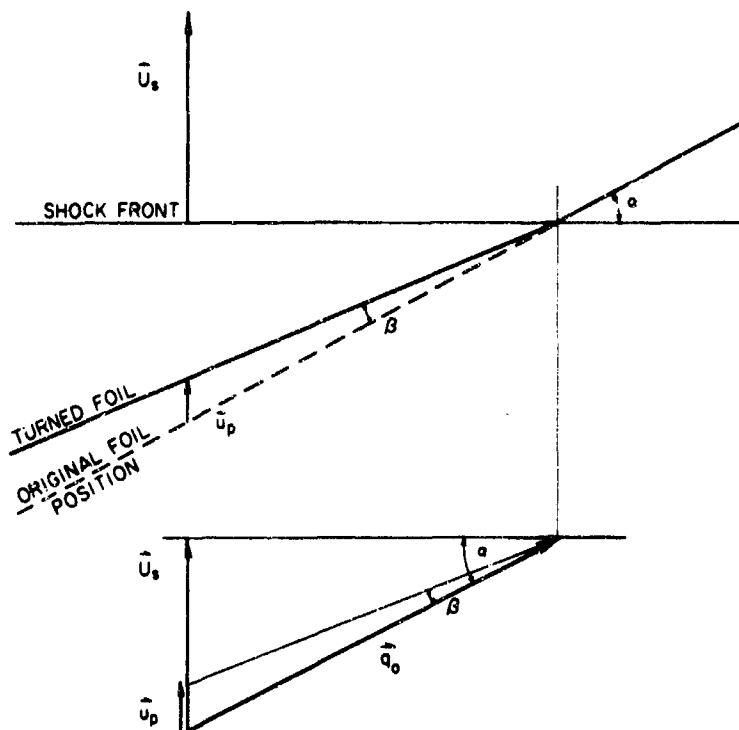
FIG. 24 RELATIONSHIP BETWEEN SHOCK VELOCITY \bar{U}_s , FLUID PARTICLE VELOCITY \bar{u}_p , APPARENT VELOCITY \bar{q}_0 , SHOCK ANGLE \alpha , AND TURNING ANGLE \beta
