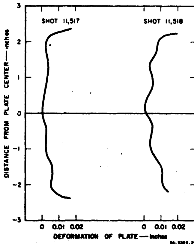
FIG. 7 RESULTS OF TESTS OF FLATNESS OF 0.325 cm/ \mu sec ALUMINUM FLYING PLATES
