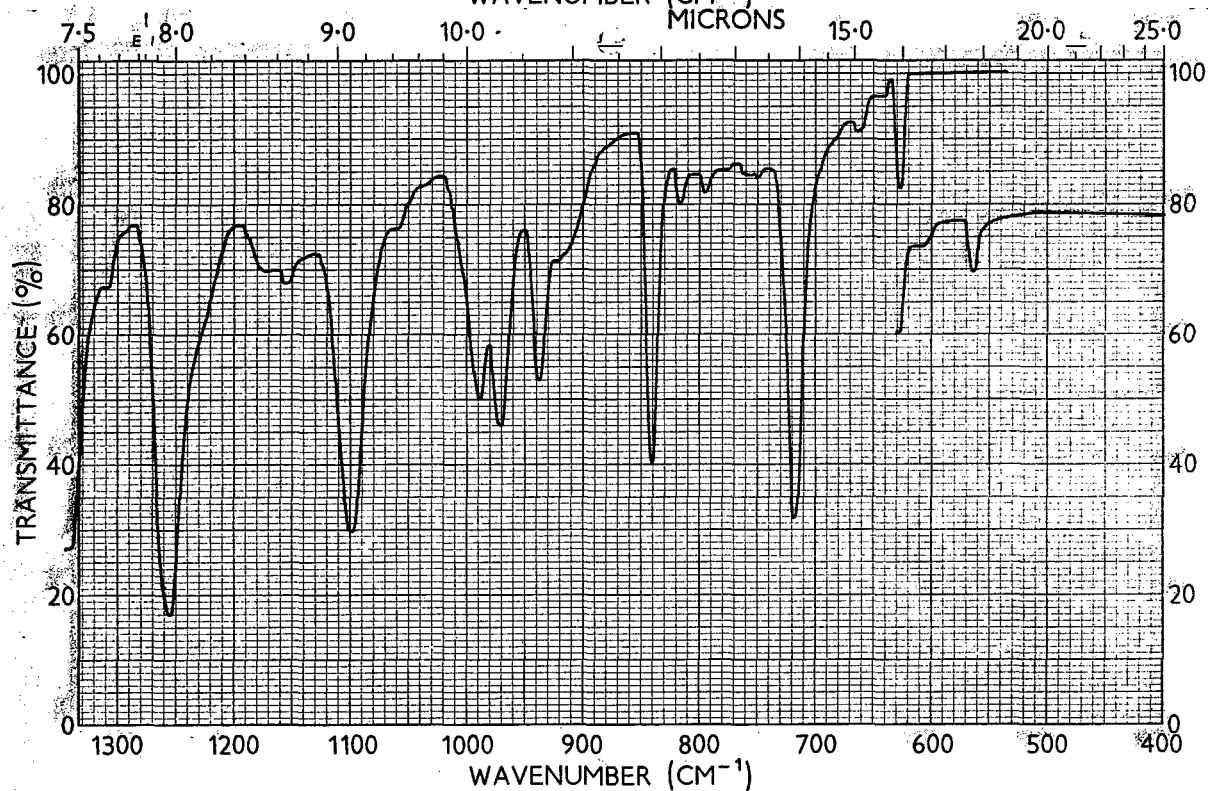
Spectrum No. 1061 Poly[octafluoro-4,4'-biphenylene)-pyromellitimide] (P.I. (9))
