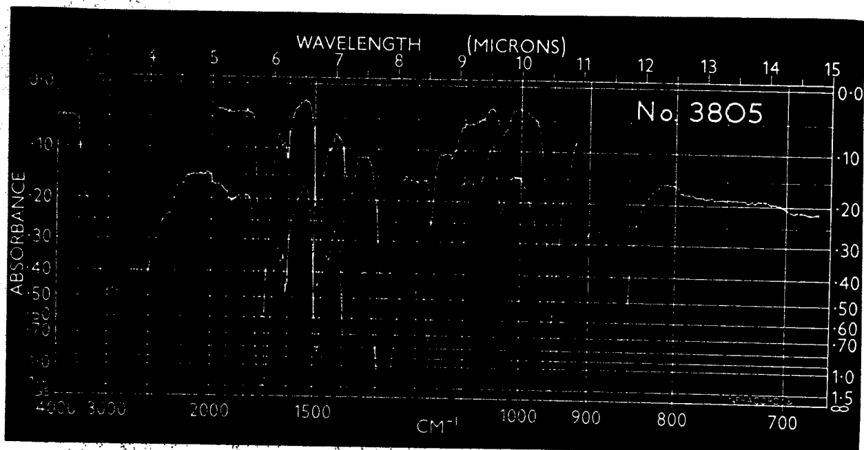
Spectrum No. 3805 2,3,5,6-Tetrafluorobenzoic acid (in \text{CHCl}_3 )
