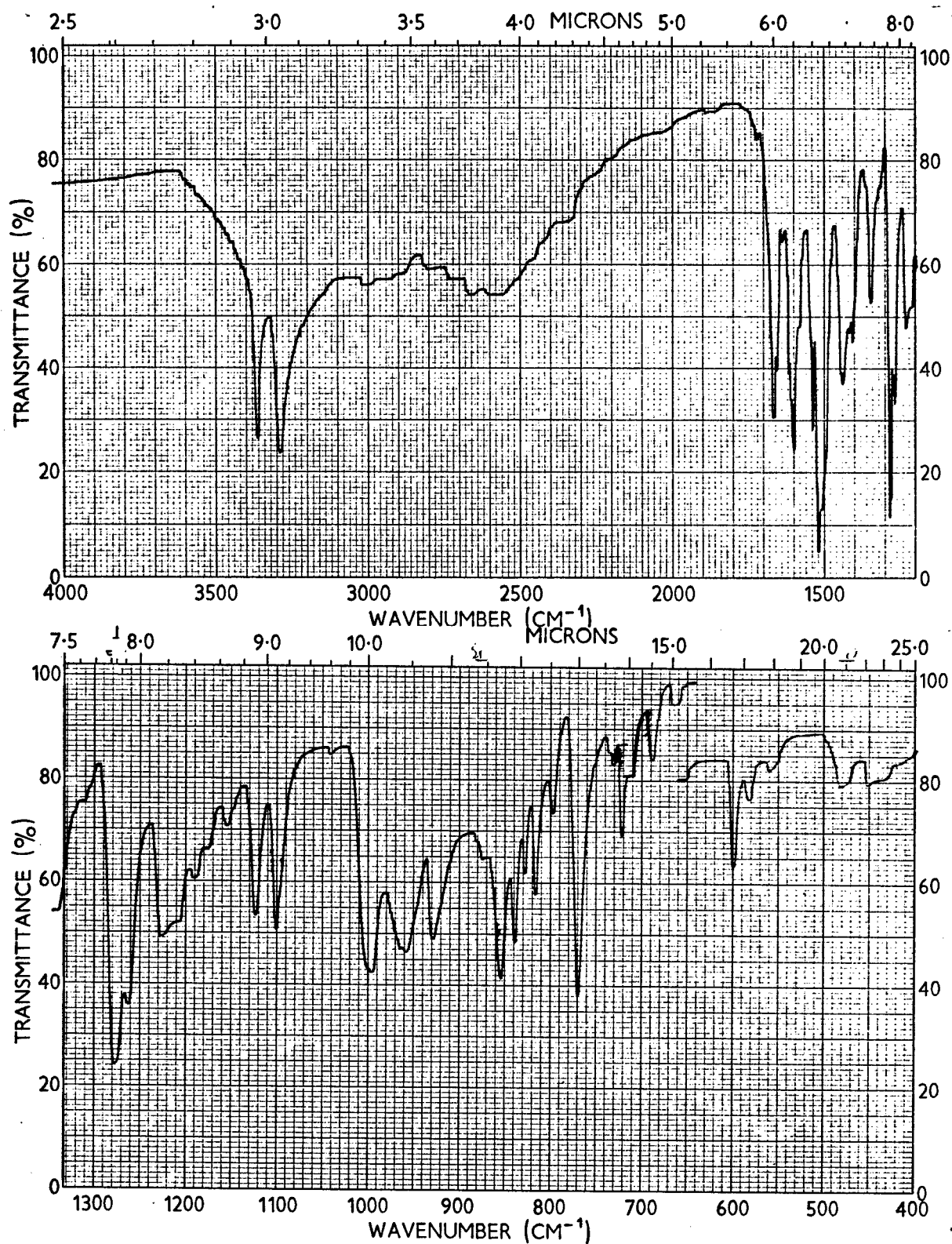
Spectrum No. 1440 Reaction product of pentafluorobenzoyl chloride and 3,3'-dihydroxybenzidine (XI)
