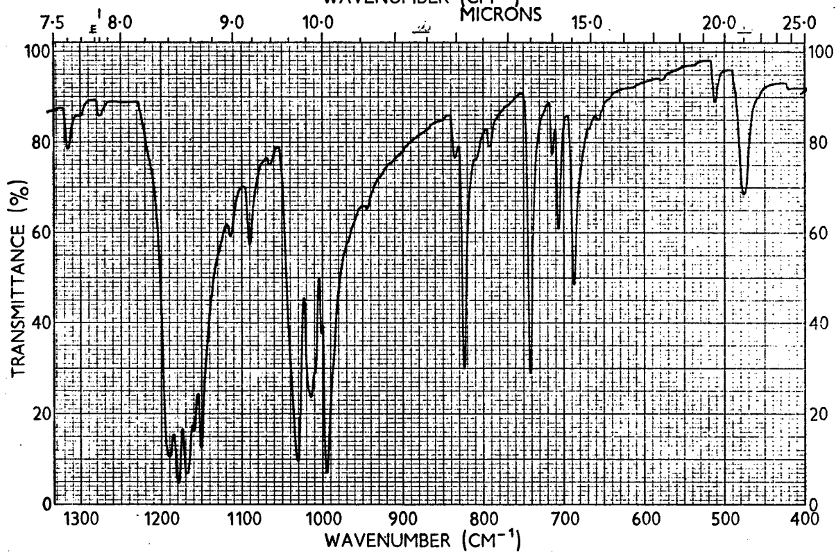
Spectrum No. 1409 0,0-(4,4'-Biphenylene) di(S-phenyl-dithiocarbonate) (XVI)
