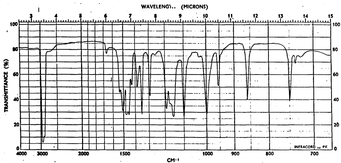
Spectrum No. 4. 3',6'-Bis(trifluoromethyl)decafluoro-p-terphenyl (VI)
