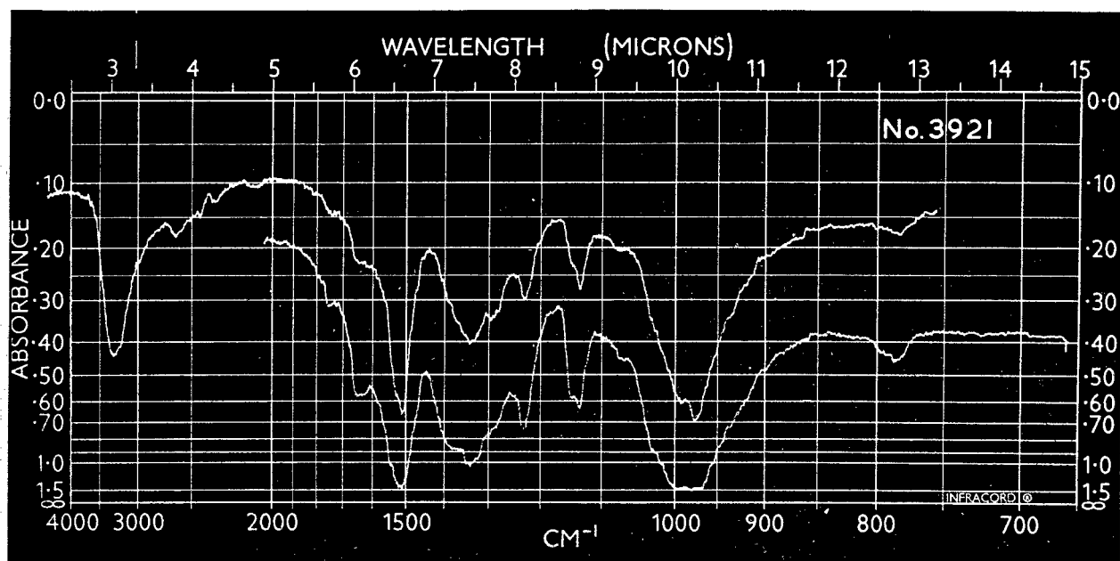
Spectrum No. 3921 Tetrafluororesorcinol (KBr disc)
