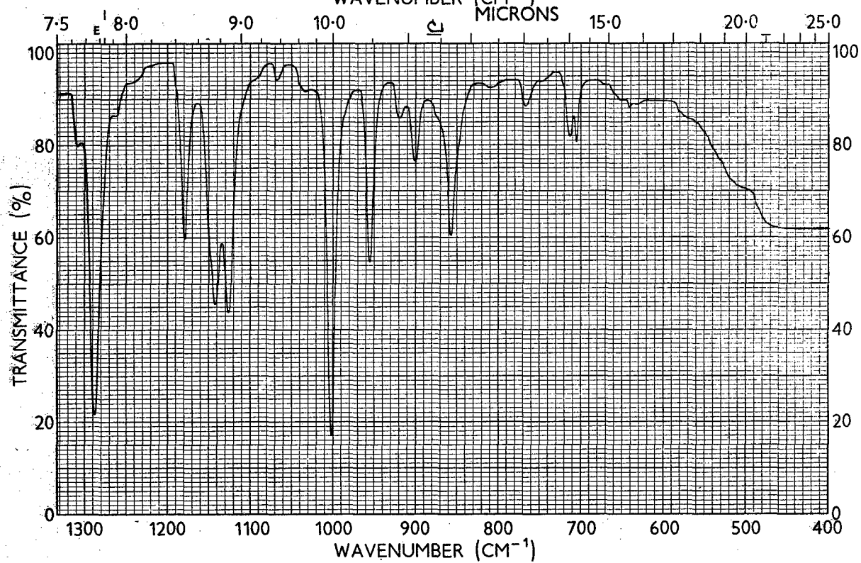
Spectrum No. 1117 1,3-Di(2,3,5,6-Tetrafluorobenzoyloxy)- 2,4,5,6-tetrafluorobenzene (XXII)
