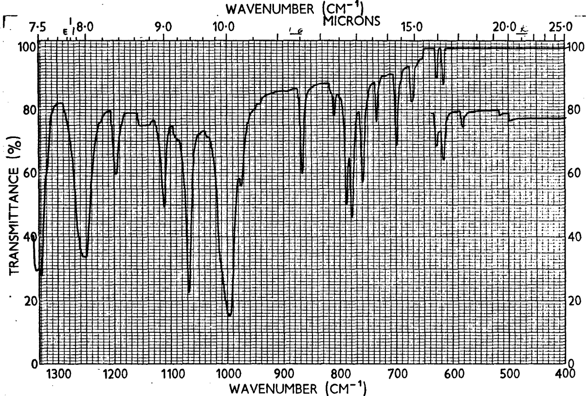
Spectrum No. 1126 Nc1ccc(cc1C(=O)c2cc(F)(F)F)c3cc(F)(F)Fcc3Nc4cc(F)(F)Fcc4C(=O)c5cc(F)(F)F N,N'-Di(pentafluorobenzoyl)-N,N'-di- (pentafluorophenyl)-2,3,5,6-tetra- fluorophenylene diamine (XIX)
