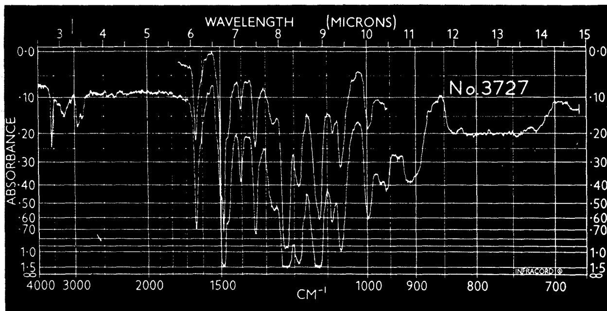
Spectrum No. 3727 Impure 3,3'-bis(1-hydroxy-2,2,3,3,4,4,4-heptafluorobutyl)octafluorobiphenyl (in CCl 4 )
