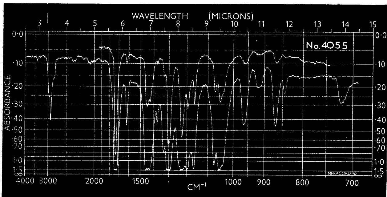
Spectrum No. 4055 Difluoro-bis(methoxycarbonyl)xylene (in CCl 4 )
