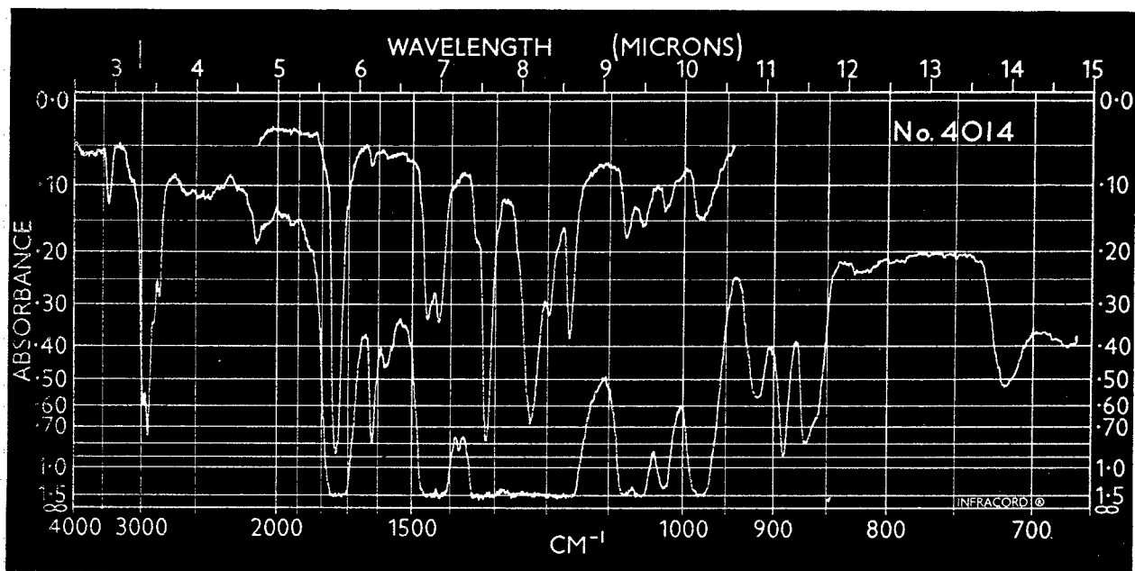
Spectrum No. 4014 2,5-Difluoro-3,4,6-tris(methoxycarbonyl)- toluene (in CCl 4 )
