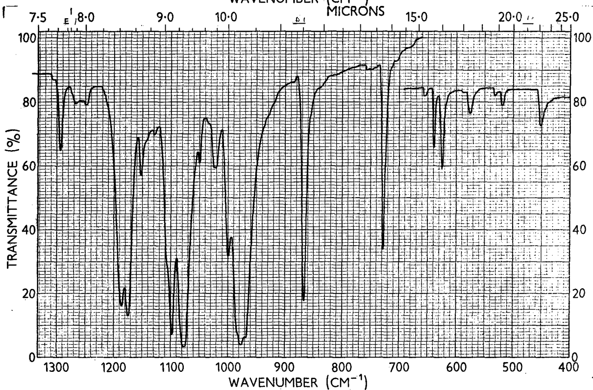
Spectrum No. 1410 0,0-(4,4'-Octafluorobiphenylene) di(S-pentafluorophenyl dithiocarbonate) (XV)
