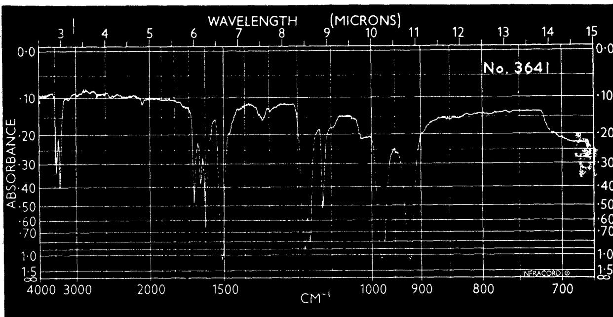
Spectrum No. 3641 Tetrafluoro-m-phenylenediamine (in CCl 4 )
