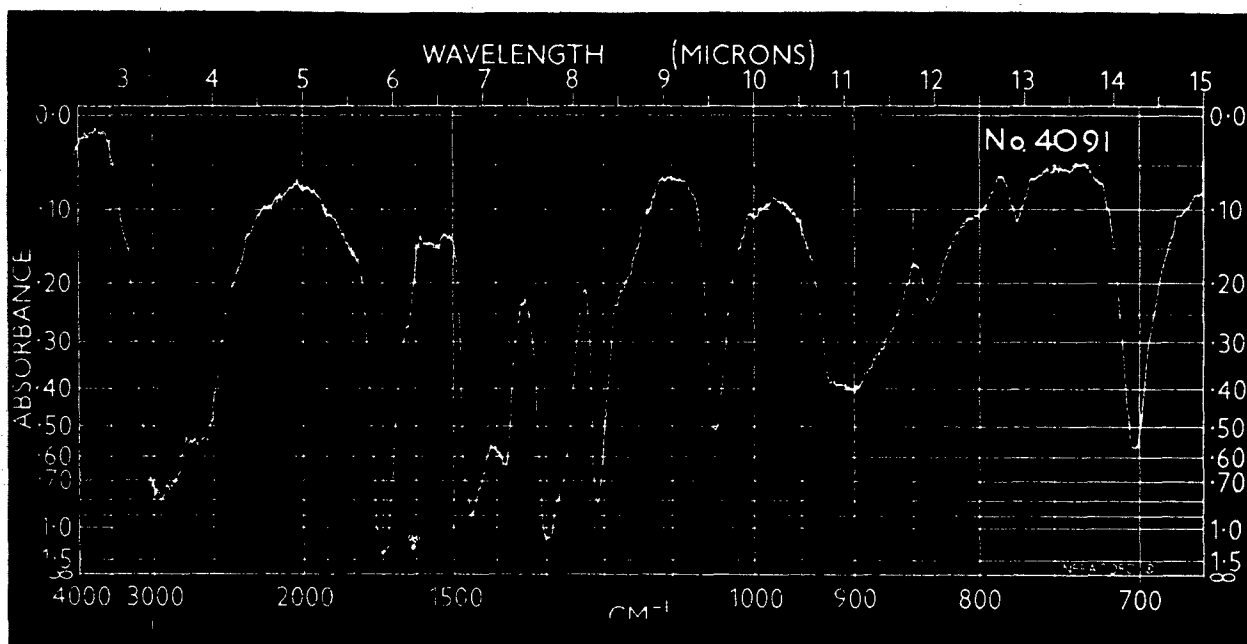
Spectrum No. 4091 Difluoroxylene dicarboxylic acid (KBr disc)
