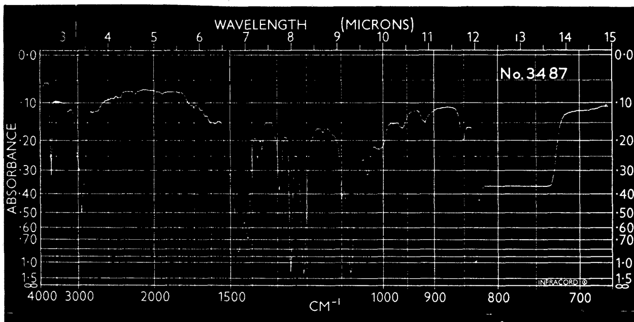
Spectrum No. 3487 3-Fluoro-6-hydroxy durene (in \text{CCl}_4 )
