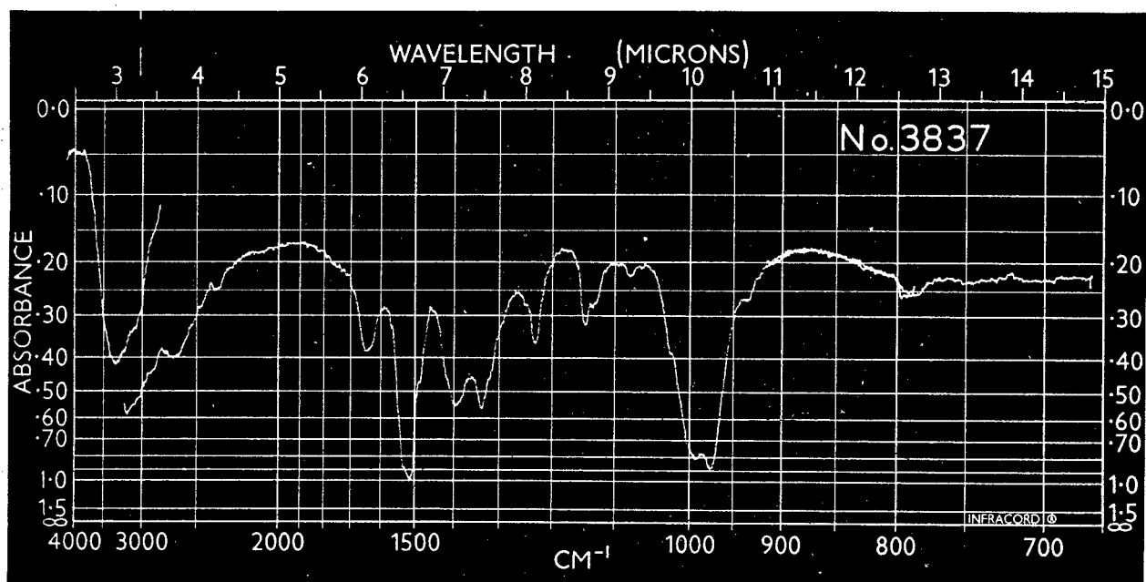
Spectrum No. 3837 Tetrafluororesorcinol (KBr disc)
