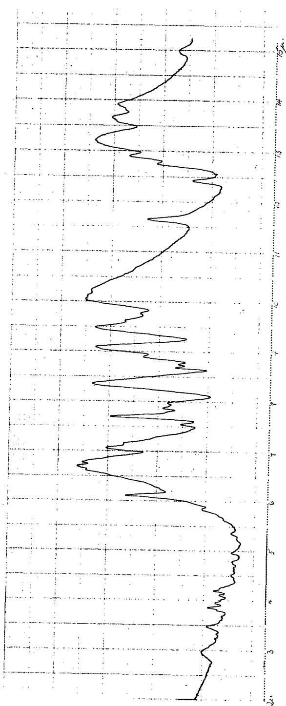
Spectrum No. 594 4,4'-Di(pentafluorophenylsulphonyloxy)biphenyl
