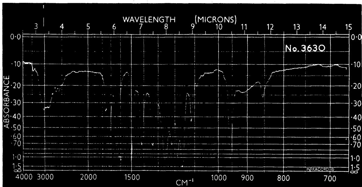
Spectrum No. 3630 Heptafluoro-m-toluic acid (in \text{CCl}_4 )
