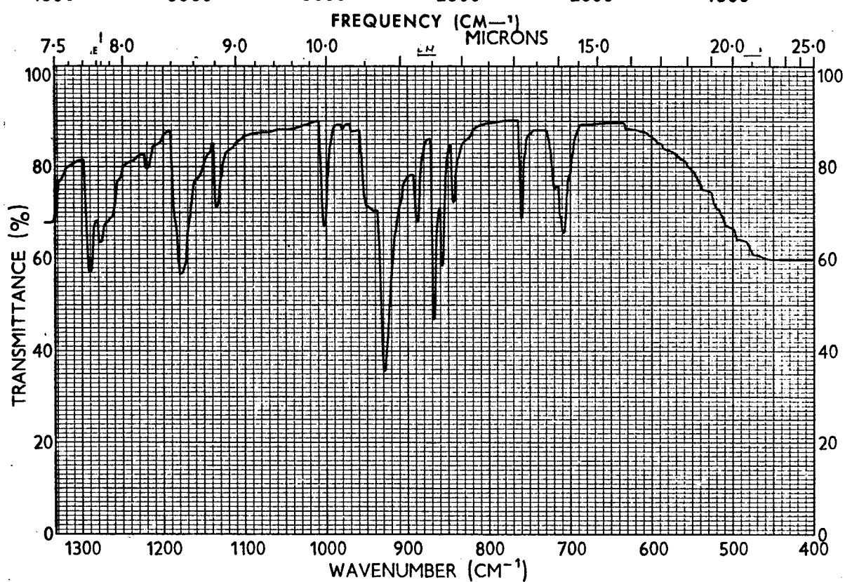
Spectrum No. 949 2,5-Di(2,3,5,6-tetrafluorophenyl)- 1,3,4-oxadiazole (XXI)
