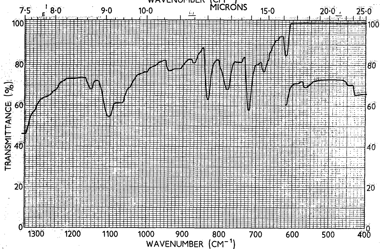
Spectrum No. 1058 Poly(m-phenylenepyromellitimide) (P.I. (1))
