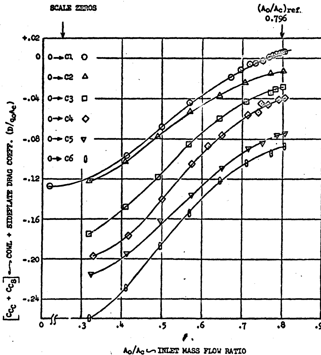
Figure 5L CONV. + SIDEPLATE DRAG \rightarrow RISPIC1 THRU C6, \alpha = \beta = 5^\circ , M_0 = 0.69
