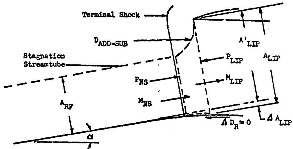
Figure 30. Subsonic Spillage
