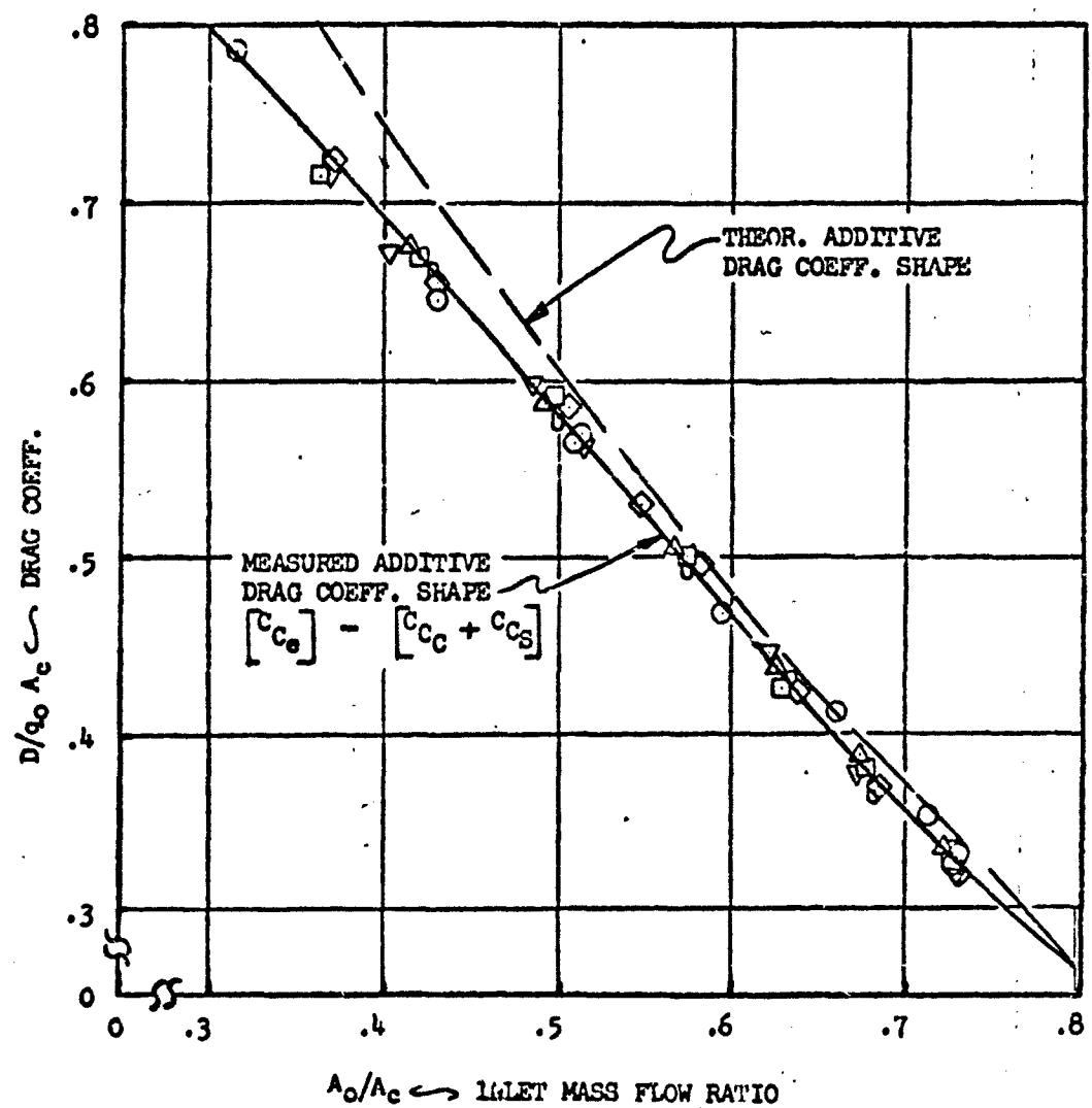
Figure 47. ADDITIVE DRAG COEFF. SHAPES ~ MEASURED vs. THEORY, M_0 = 1.09
