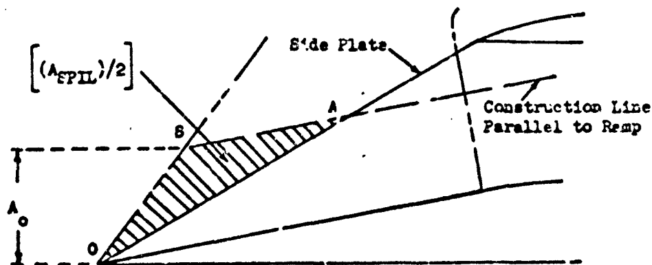
Figure 27. Side Spillage Area
