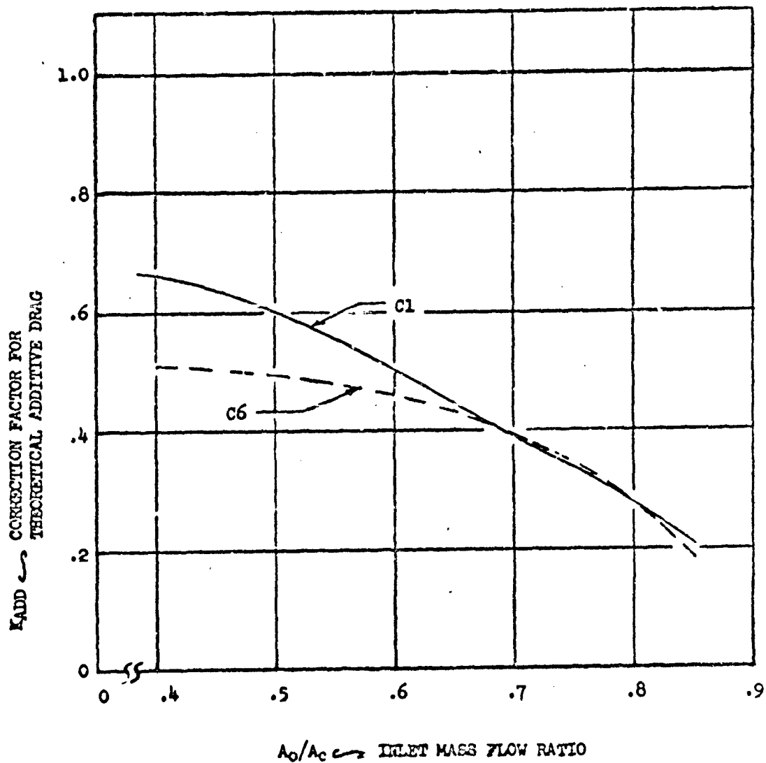
Figure 71. K_{ADD} , R4SP4C1, C6, M_0 = 0.865
