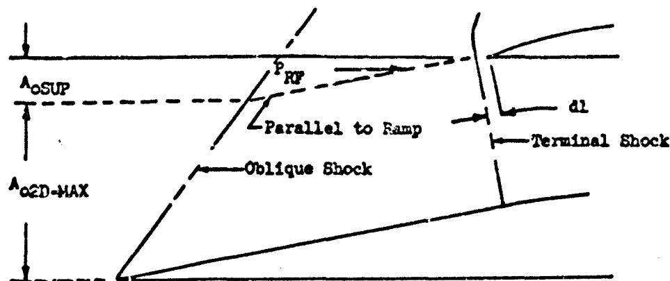
Figure 26. Supersonic Spillage
