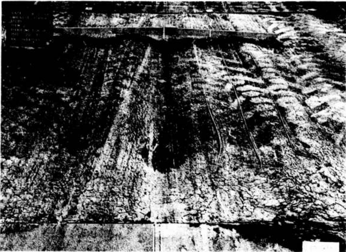
Figure 4. Lane 1, item 2, at 300 coverages (traffic suspended, no failure)
