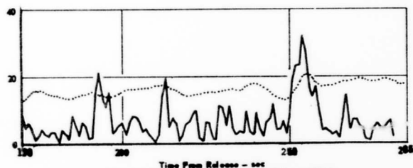
Figure 30 BANK ANGLE AND RATE OF DESCENT vs TIME FROM RELEASE OF PARACHUTIST LAUNCHED AT 60 KCAS AND 30 000 ft PRESSURE ALTITUDE TEST No. 0761
