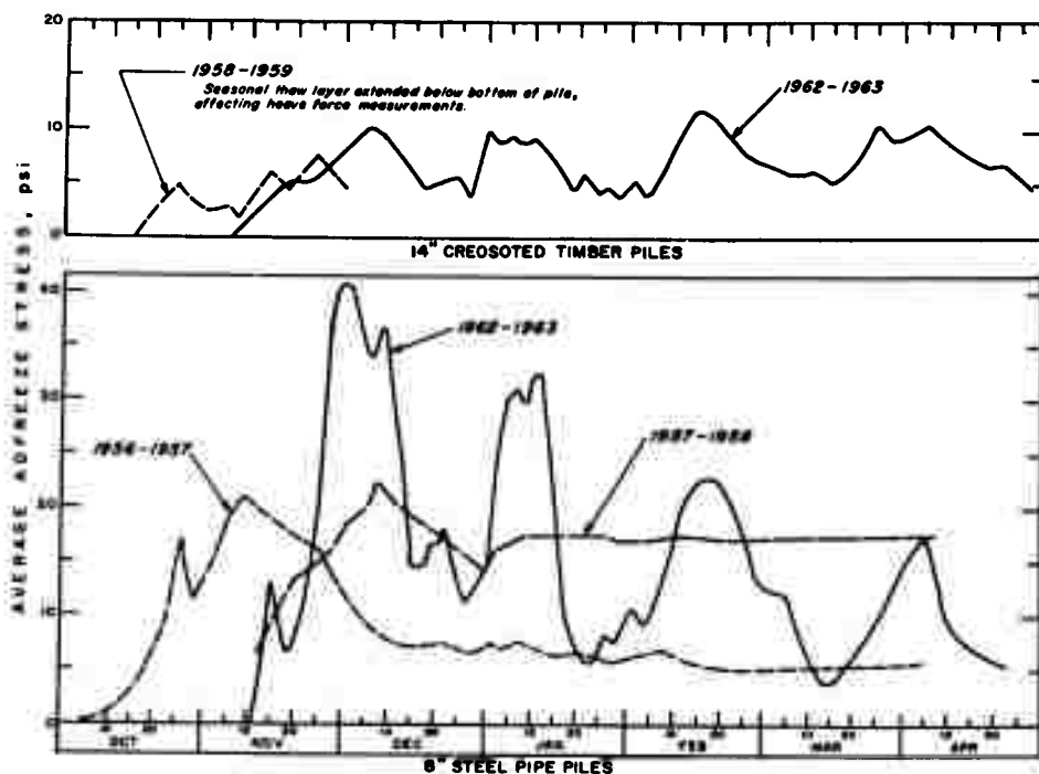
Figure 22. Average adfreeze stress vs time.
