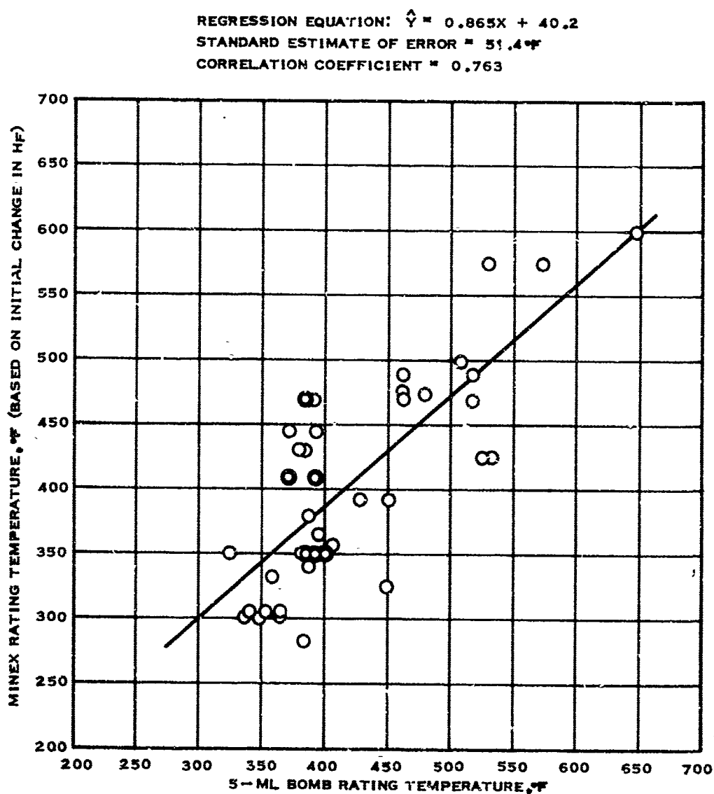
FIGURE 5 RELATIONSHIP BETWEEN 5-ML BOMB AND MINEX RATINGS OF JP FUEL THERMAL STABILITY QUALITY
