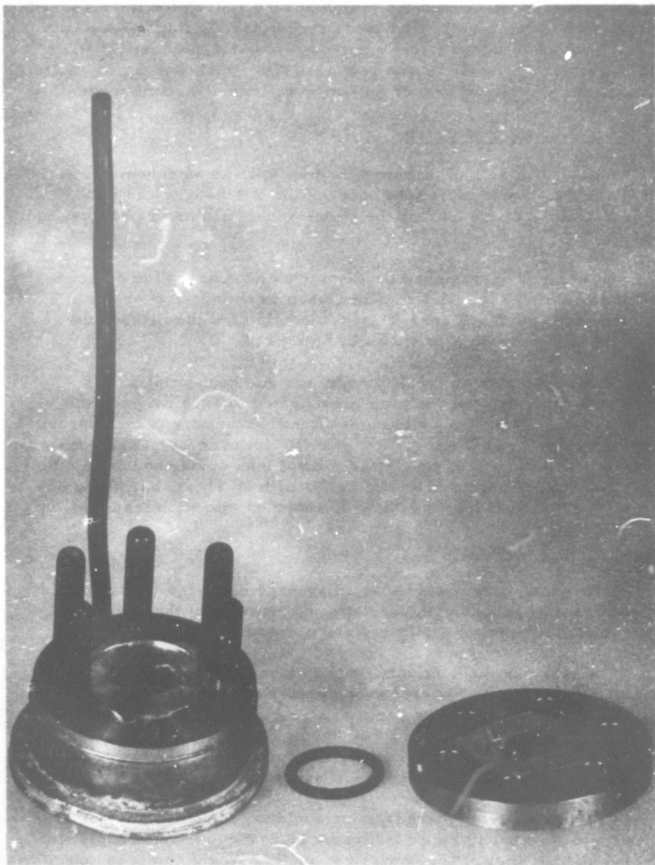
Figure 8 Flat Flanges With Indium-Elastomer Seal
