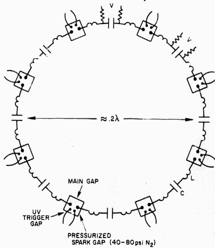
FIG. 1 BASIC RING TRANSMITTER
