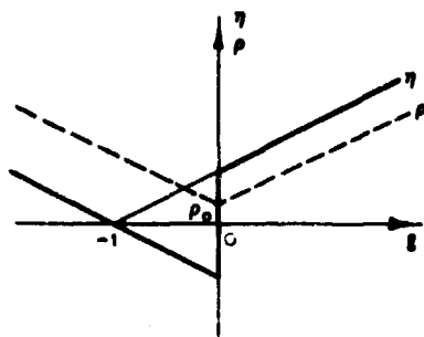
a. System for energy coefficient, considering energy loss due to sinkage at zero slip
