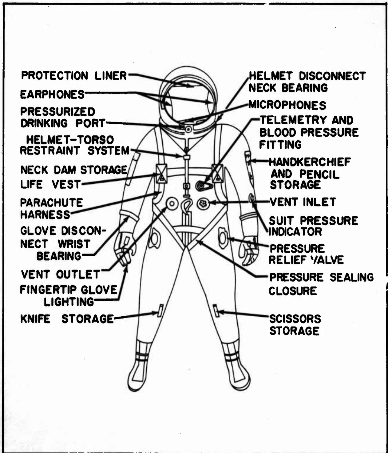
Figure I-8. MOL Type Extravehicular Space Suit
