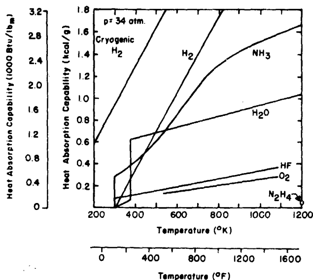
Figure 6. Heat Absorption Capabilities of Some Transpiration Coolants
