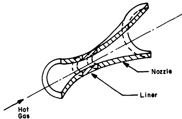
Figure 15. Flow of Hot Gas Through a Rocket Nozzle with a Liner at the Throat 29
