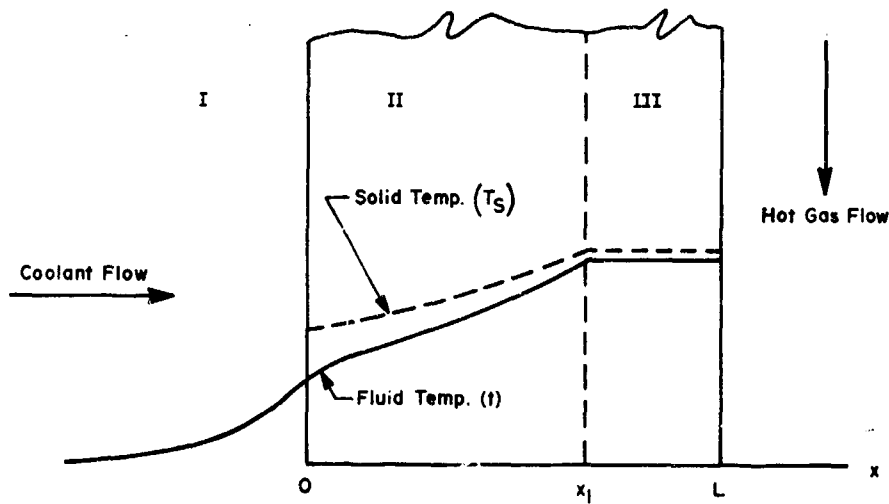
Figure 13. Two-Phase Coolant System (Coolant Exits at a Quality) 13
