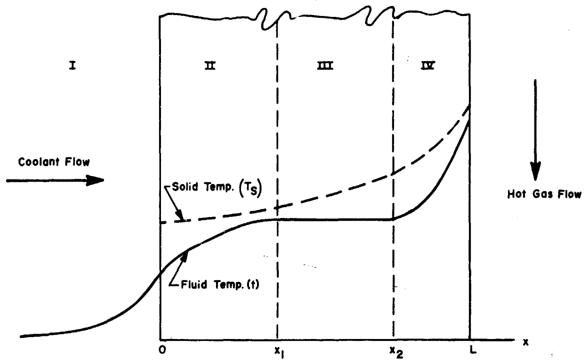
Figure 14. Two-Phase Coolant System (Coolant Exits Superheated) 13
