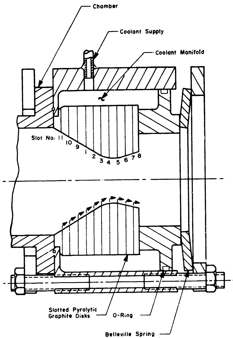
Figure 22. Multislot, Film Cooled Pyrolytic Graphite Nozzle 5
