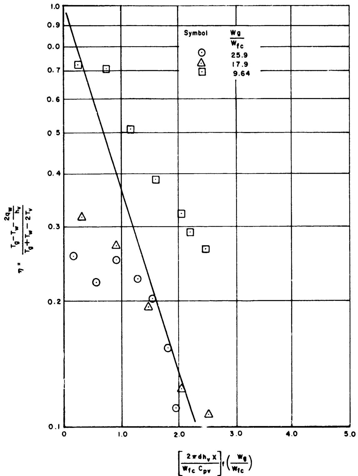
Figure 33. Temperature Ratio Parameter as a Function of the Length Parameter for Water Film Coolant - Gas Stream Reynolds Number = 0.55 ( 10^5 )
