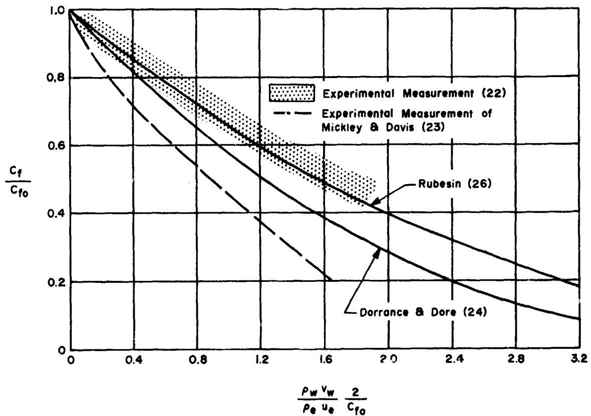
Figure 11. Predicted and Measured Skin Friction for Air Injection into a Turbulent Boundary Layer
