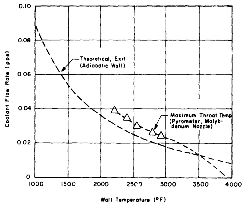
Figure 24. Variation of Analytical and Experimental Nozzle Temperatures with Flow Rate-Radiation/Hydrogen Film Cooling 5
