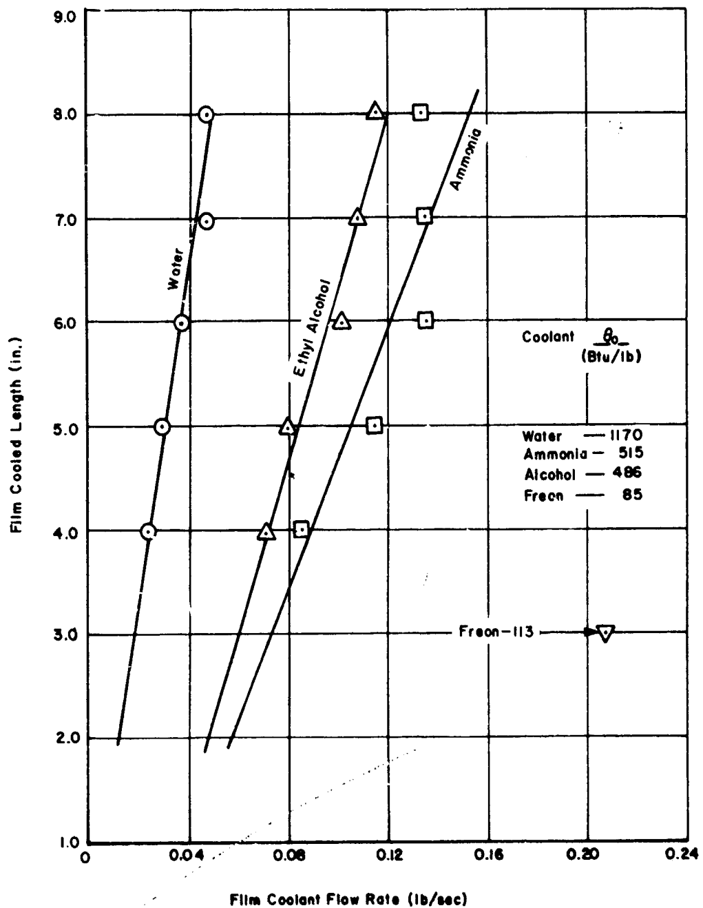
Figure 28. Variation of Film-Cooled Length with Film Coolant Flow Rate for Different Film Coolants
