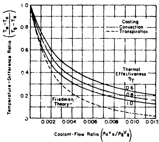
(c) Turbulent flow without radiation Reynolds number = 10^7
