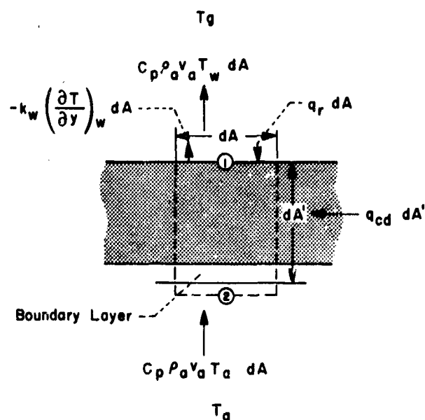
Figure 8. Sketch of Element of Wall Used in Setting Up Heat Balance for Transpiration Cooling
