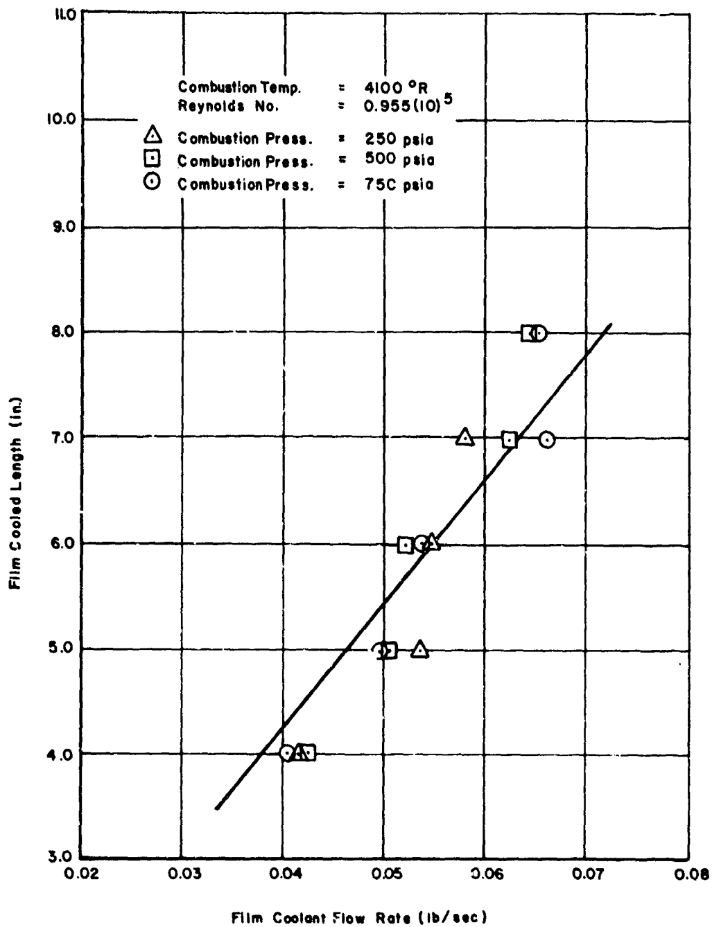
Figure 29. Variation of Film-Cooled Length with Film Coolant Flow Rate for Different Combustion Pressures - H 2 O Film Coolant 31
