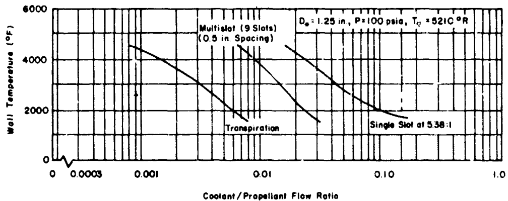
Figure 1. Comparison of Cooling Techniques for Nozzles- \text{O}_2/\text{H}_2 Fuel and \text{H}_2 Coolant 5
