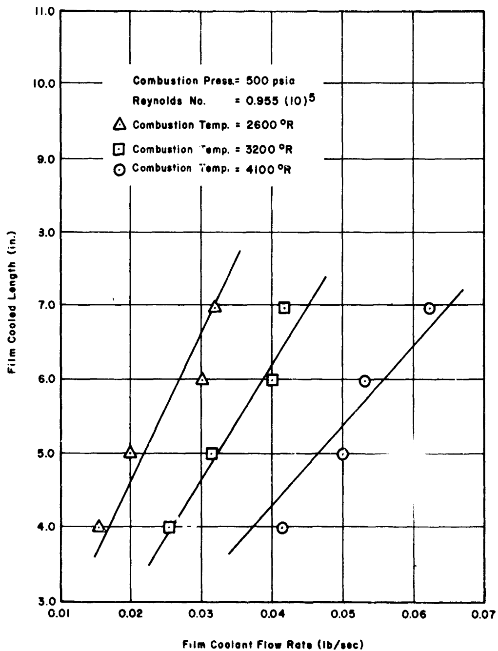
Figure 30. Variation of Film-Cooled Length with Film Coolant Flow Rate for Different Combustion Temperatures - H 2 O Film Coolant 31
