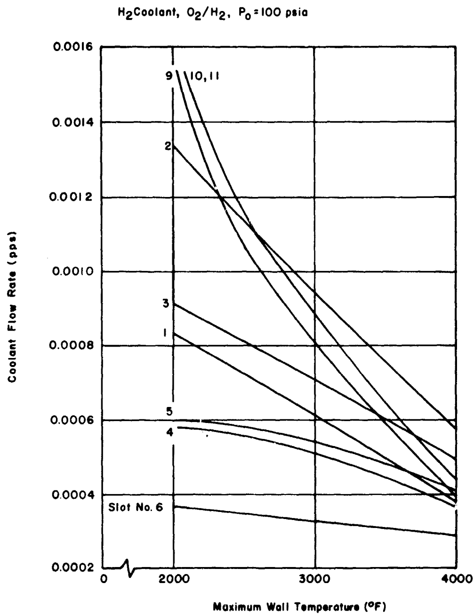
Figure 23. Gaseous Film Cooling for Standard Nozzle with Multislot Cooling 5
