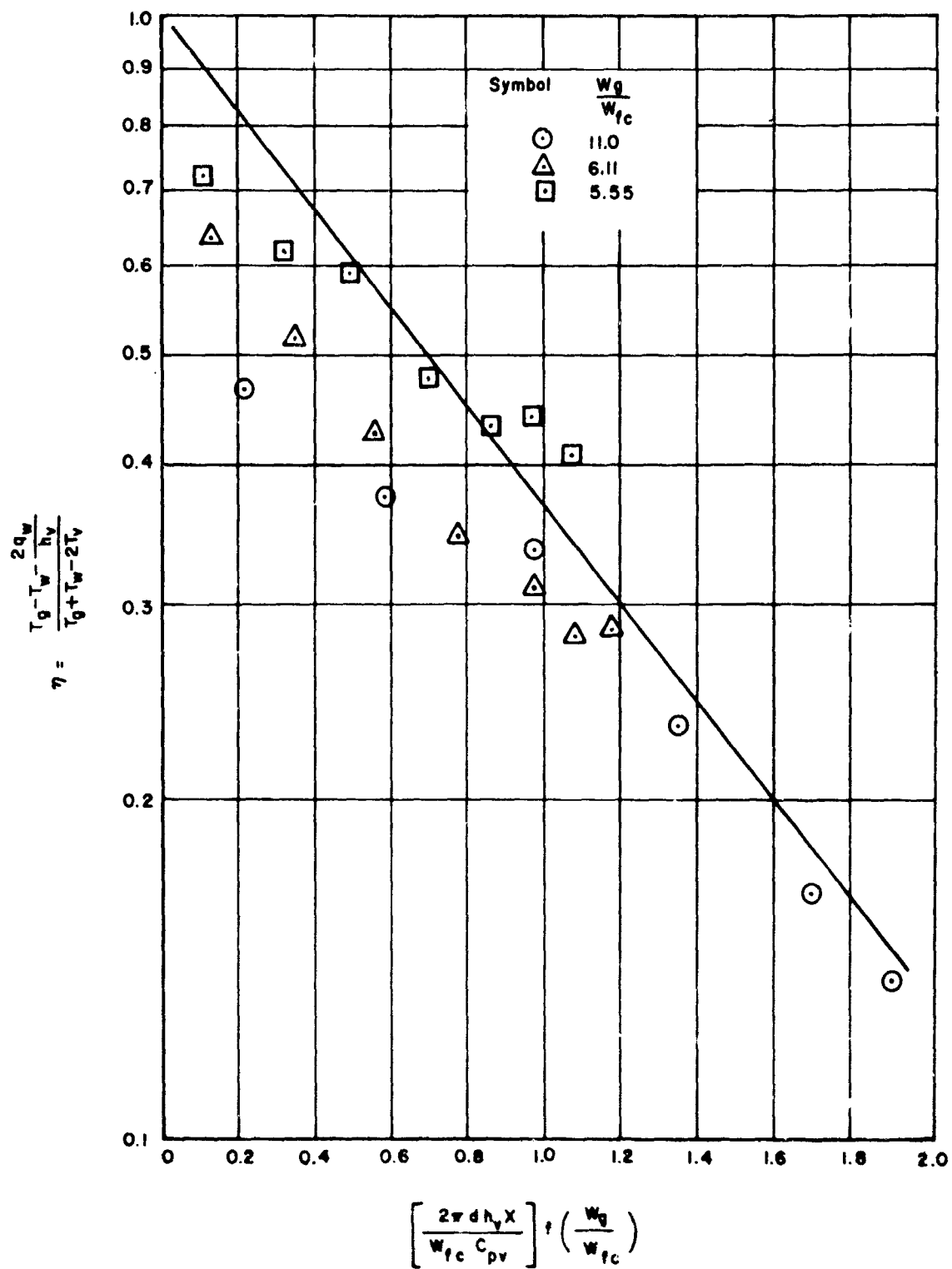
Figure 32. Temperature Ratio Parameter as a Function of the Length Parameter for Ammonia Film Coolant - Gas Stream Reynolds Number = 0.55 (10^5)
