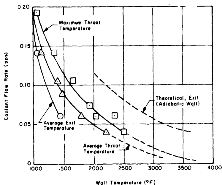
Figure 25. Variation of Analytical and Experimental Nozzle Temperatures with Flow Rate - Radiation/Helium Film Cooling 5
