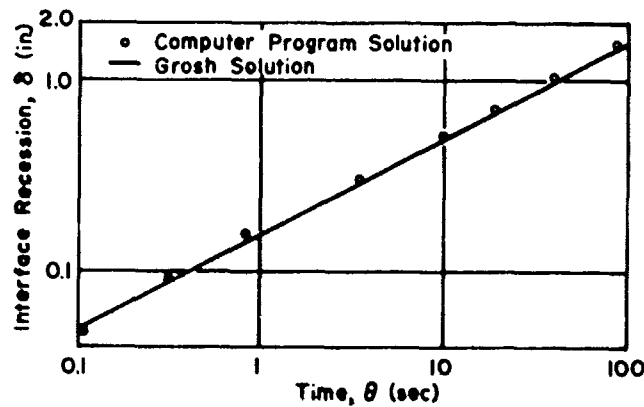
Figure 17. Comparison of Computed Interface Recession Distance with Grosh Solution: Zinc, P = 0.3
