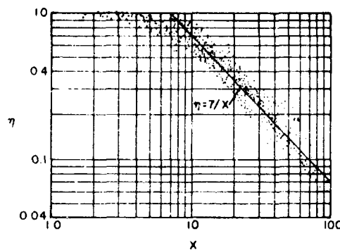
Figure 21. Agreement Between Equation (44) and the Data of Various References 43
