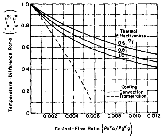
(a) Laminar flow without radiation Reynolds number = 10^4
