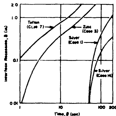
Figure 18. Interface Recession for Various Infiltrants
