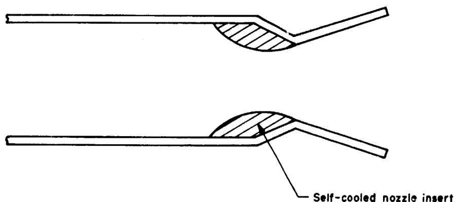
Figure 3. Self-Cooling of Rocket Nozzle
