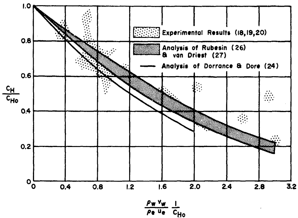
Figure 10. Comparison of Heat Transfer Results
