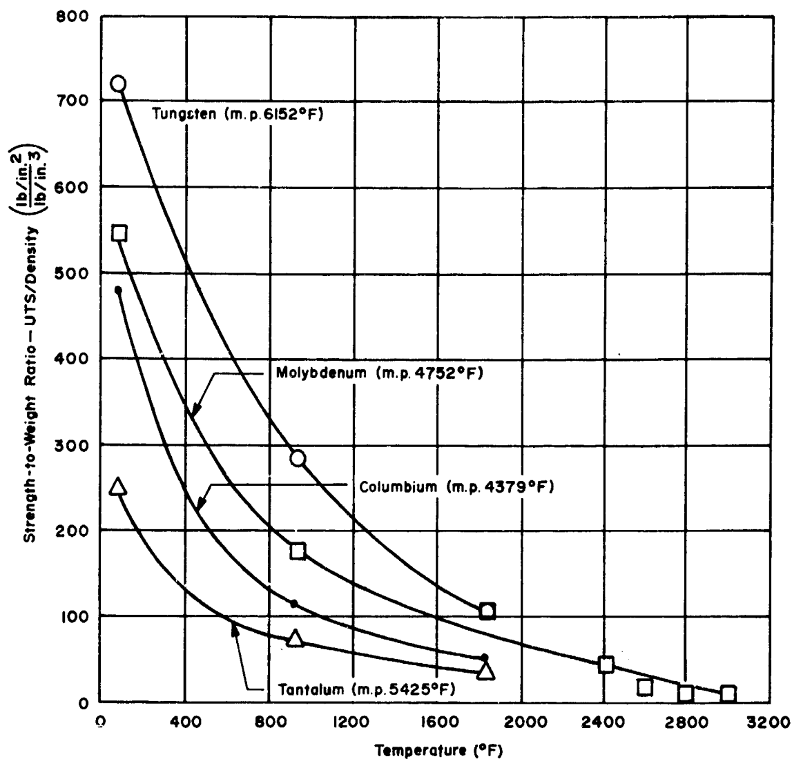
Figure 5. Strength-to-Weight Ratios of Some Refractory Metals 8
