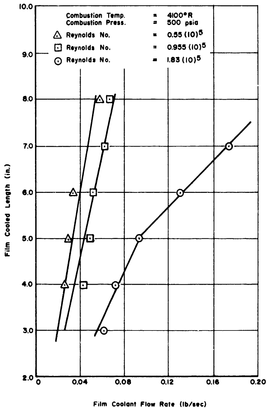
Figure 31. Variation of Film-Cooled Length with Film Coolant Flow Rate for Different Main Stream Reynolds Numbers - H 2 O Film Coolant 31
