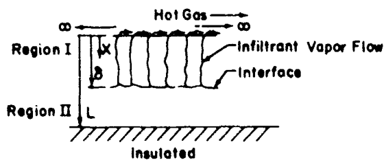
Figure 16. Model After the Liquid/Vapor Interface Has Formed 28
