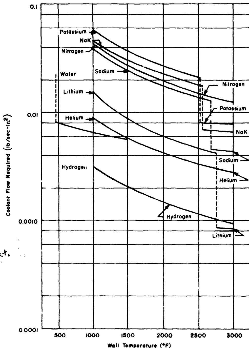
Figure 7. Coolant Weight Requirements Versus Wall Temperature
