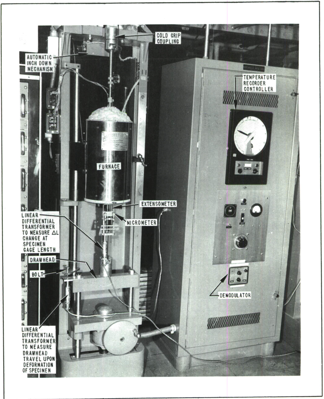
Figure 5. Test Apparatus for Correlation of Strain Measurement Techniques
