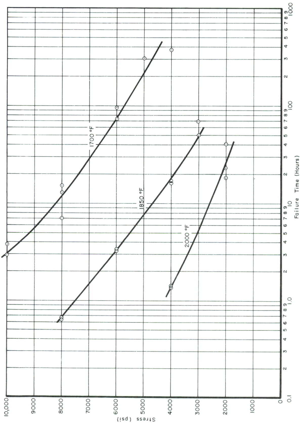
Figure 14. Stress Rupture Properties of Chrome-30
