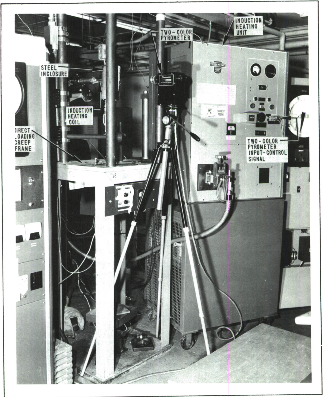
Figure 3. Trial Test Apparatus Setup for 2200°F
