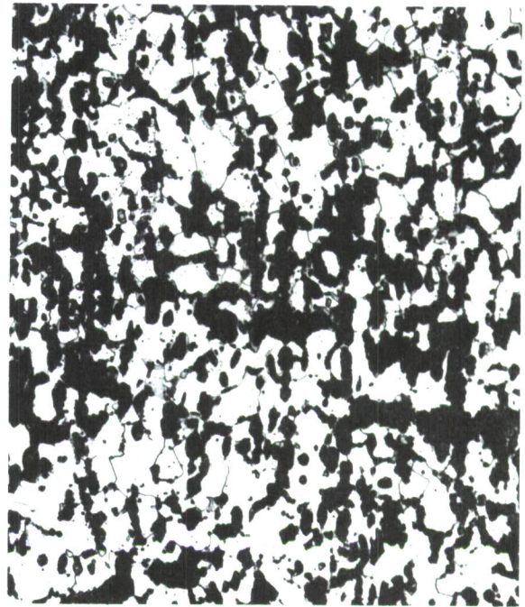
Figure 18B. Stress - 6000 psi Failure - 96.8 hours
