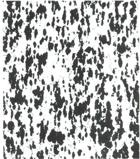
Figure 18D. Stress - 10,000 psi Failure - 3.8 hours
