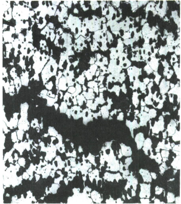
Figure 20B. Stress - 4000 psi Failure - 1.4 hours
