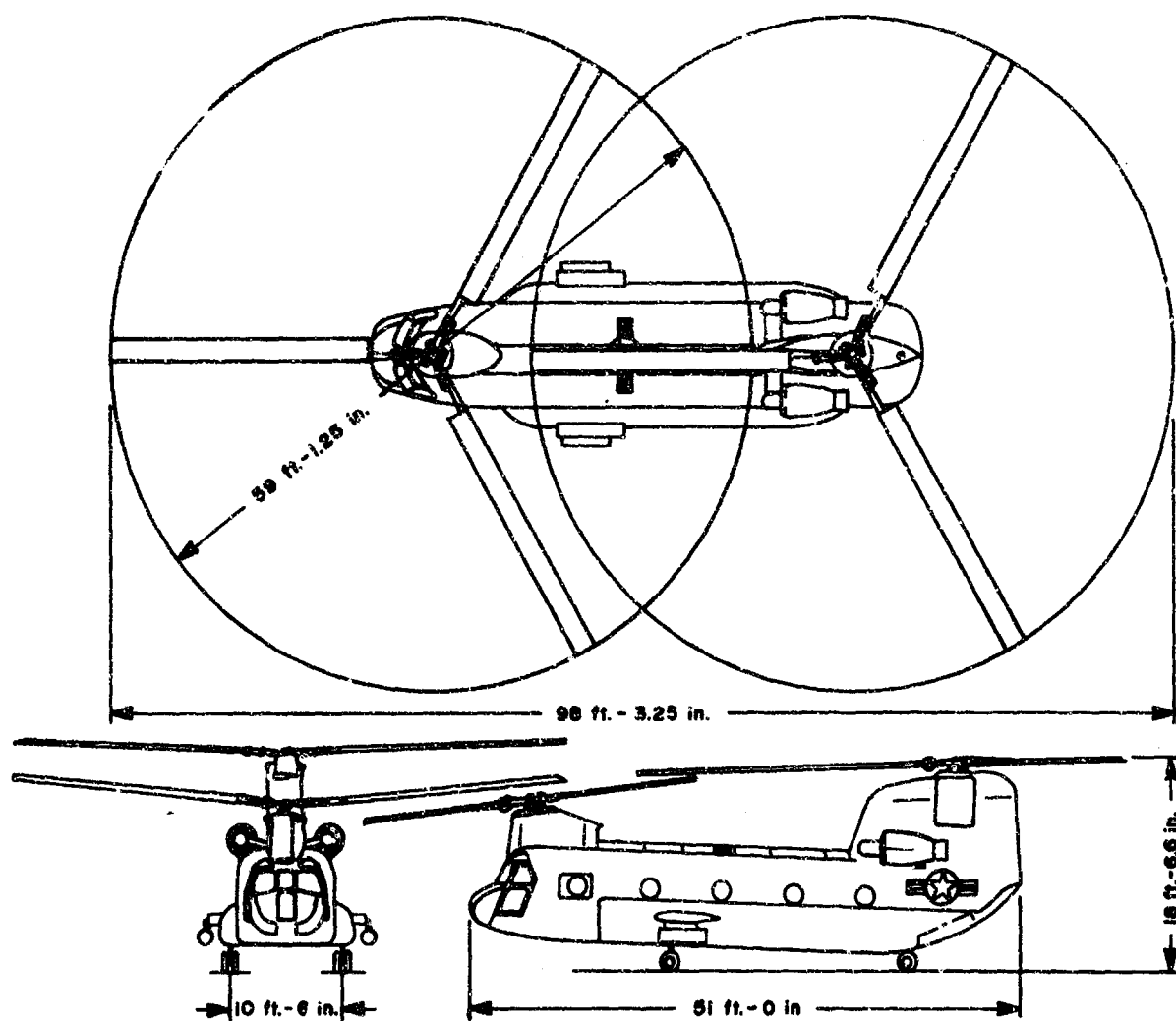
Figure 8. Overall Dimensions of the CHINOOK Helicopter .
