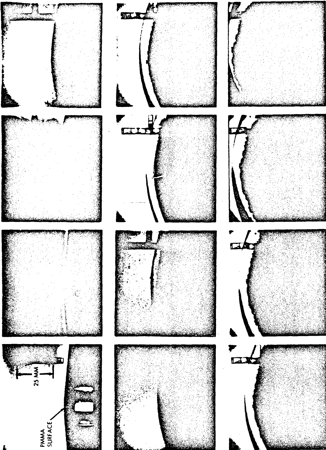
FIG. 4 JACOBS FRAMING CAMERA SEQUENCE OF RECORD 217 ILLUSTRATING SPALL OVERTAKING FOIL. EXPERIMENTAL DETAILS: MODEL SYSTEM SXSSGT, FOIL DIAMETER 3 MM. THE FREE END OF PMMA CYLINDER (127 MM DIAM, 50.8 MM HIGH) HAS BEEN BEVELLED 5° TO LEAVE A PLATFORM OF 10 MM DIAMETER AT CENTER. BACKLIGHTING BY THE DIFFUSE REFLECTED LIGHT OF AN EXPLOSIVE FLASHLAMP. INTERFRAME TIME: 6.53 \mu SEC. FOIL OBSERVED BY PMMA SURFACE IN LAST THREE FRAMES.
