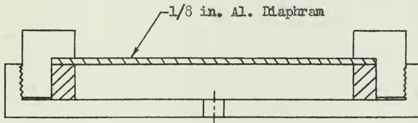
b. Cross Section View Showing Diaphragm
