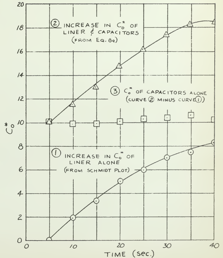
b. CHANGE OF C_o^* WITH TIME
