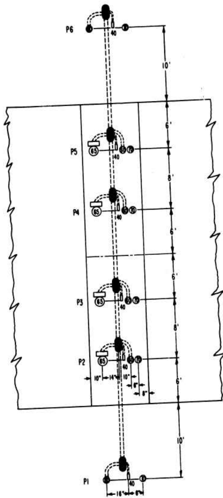
FIGURE 2.3 GAGE LAYOUT ON TERRAIN FEATURES A, B, AND C
