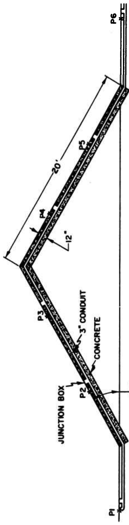
TERRAIN FEATURE TYPE C
