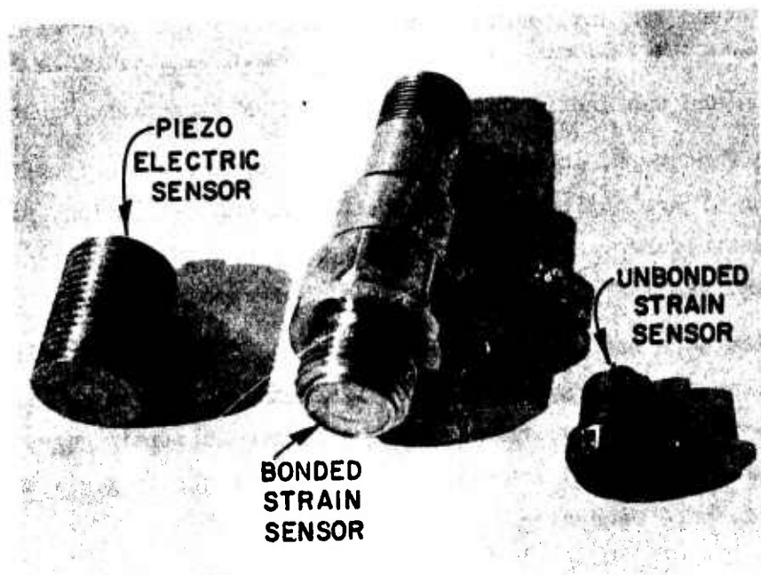
FIGURE 2.7 PRESSURE TRANSDUCERS
