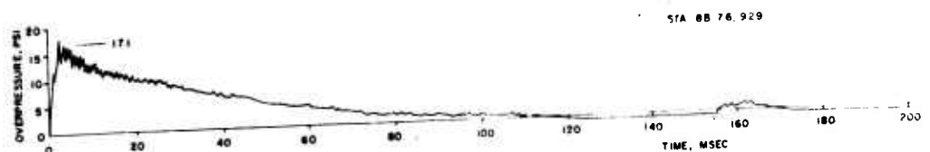
FIGURE B30 SELF-RECORDING OVERPRESSURE-TIME RECORDS FROM TERRAIN FEATURE B
