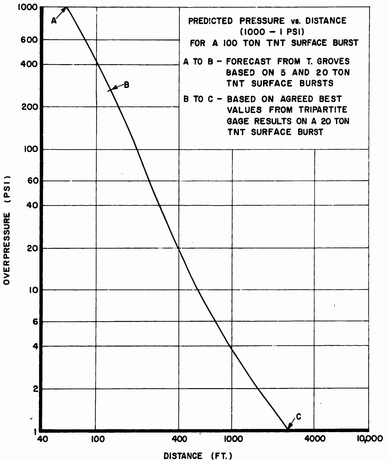
FIGURE 1.1 PREDICTED MAXIMUM OVERPRESSURE FOR 100 TON HE SURFACE BURST
