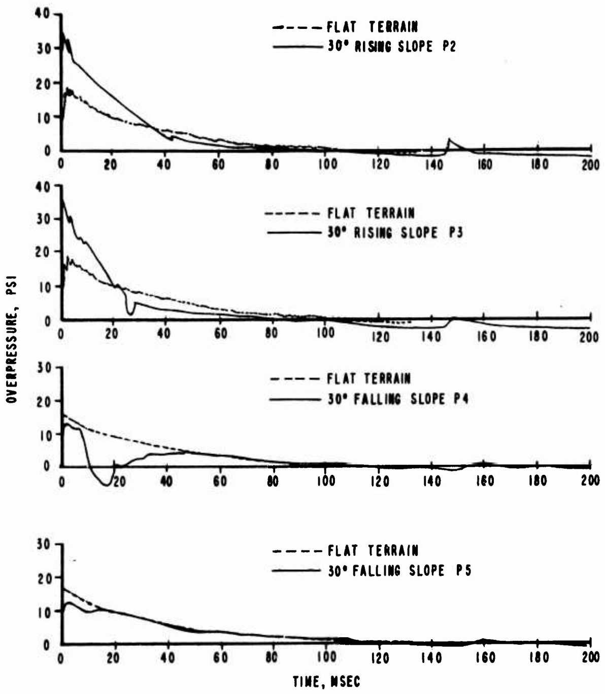
FIGURE 4.2 OVERPRESSURE - TIME ON TERRAIN FEATURE C COMPARED WITH CONTROL LINE 59
