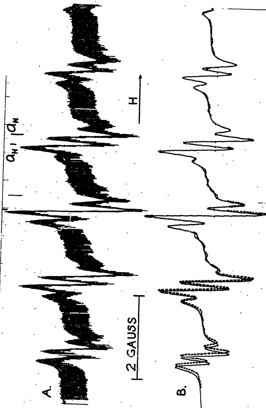
Figure 15 (a). Experimental EPR spectrum of sodium-reduced terephthalonitrile with TEAP added; 100 cps frequency markers. (b). Comparison of experimental spectrum (....) with spectrum calculated from least-squares refined coupling constants.
