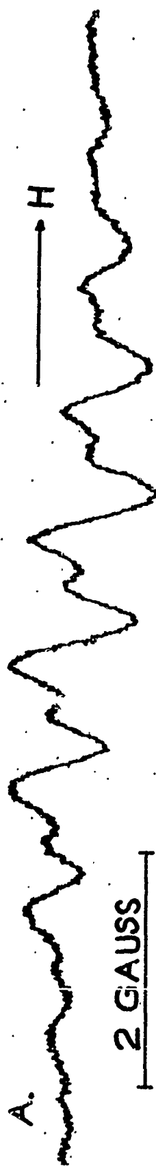
Figure 13 (a). Experimental EPR spectrum of a radical obtained by sodium reduction of hexacyanobenzene, with TRAP added.
