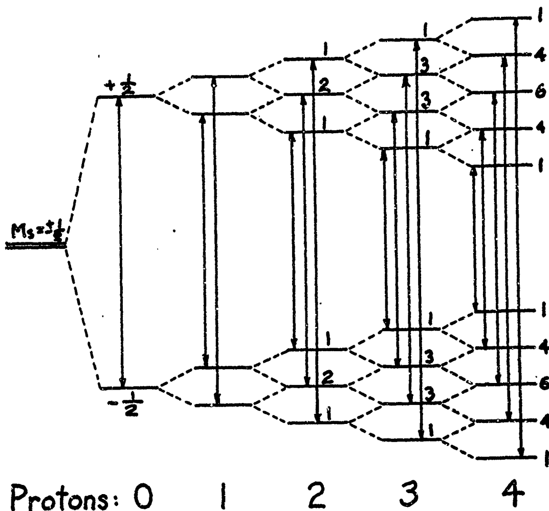
Fig. 4 (a). Hyperfine energy levels resulting from interaction of an unpaired electron with various numbers of equivalent protons. Arrows indicate allowed EPR transitions; numbers refer to degeneracies of energy levels and resulting intensity ratios of transitions. [98]
