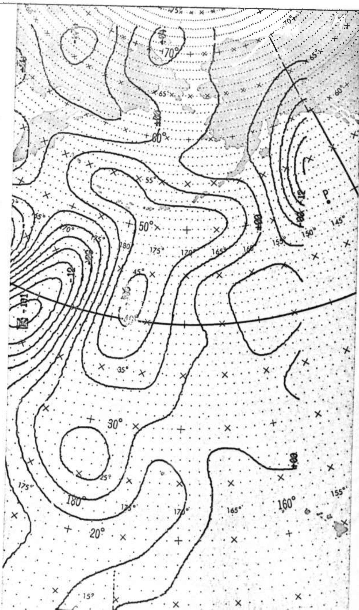
Figure 10 Local change of thickness, \Delta h , Pacific
