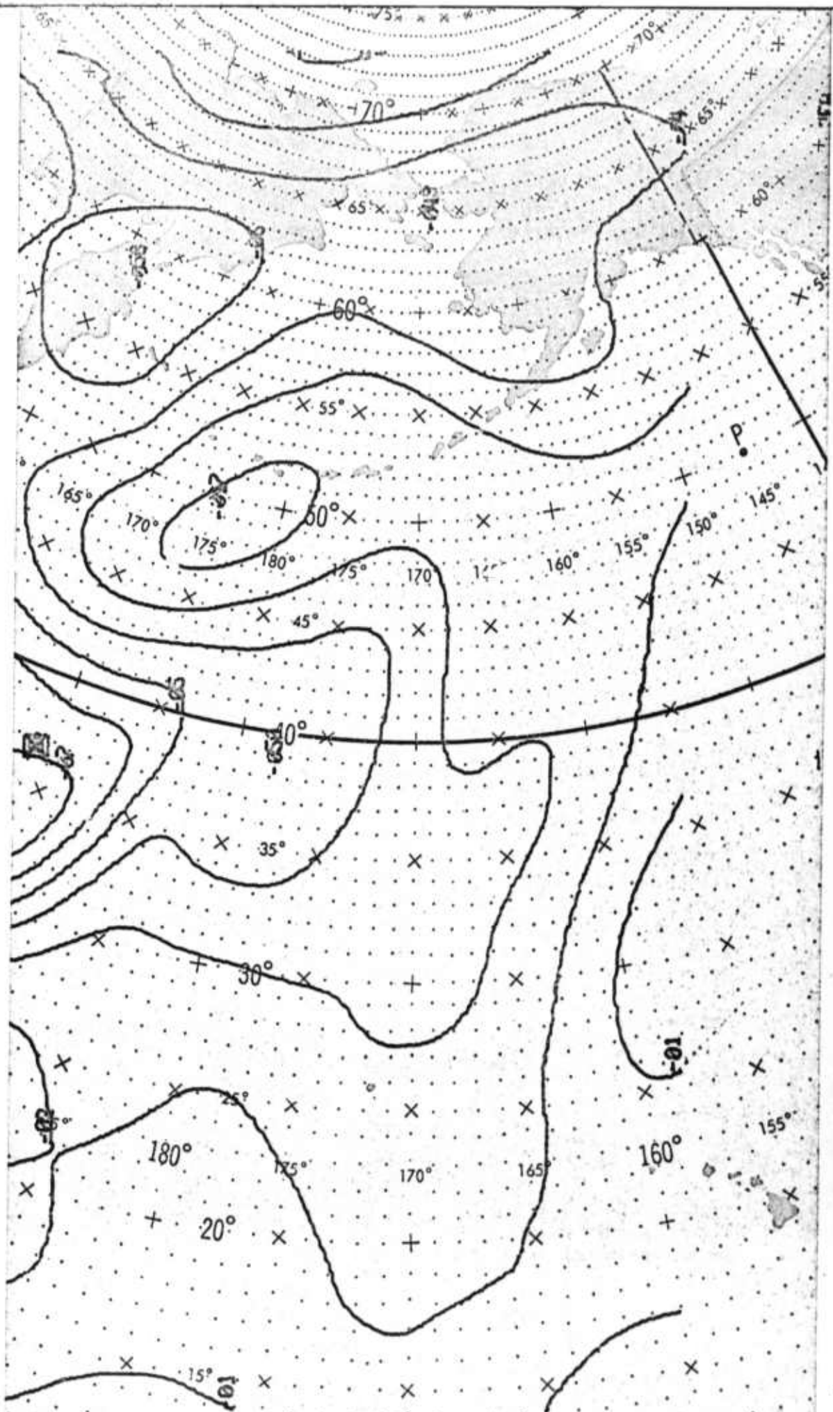
Figure 22 Mean Heating term, \bar{H} , Pacific
