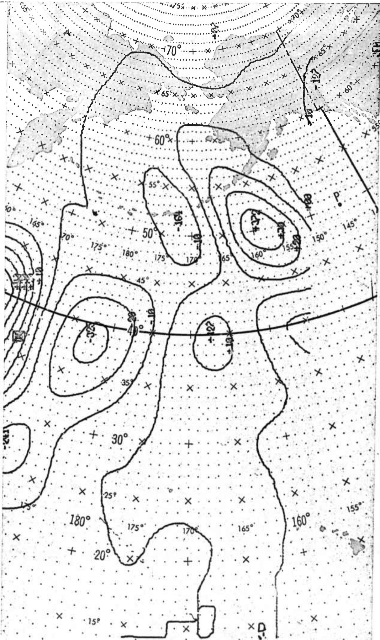
Figure 14 \sigma_w 500 , Pacific
