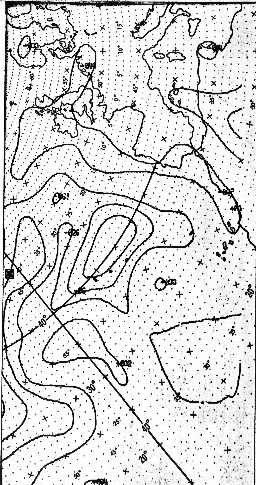
Figure 7. The combined local change of thickness and estimated horizontal advection, Atlantic.
