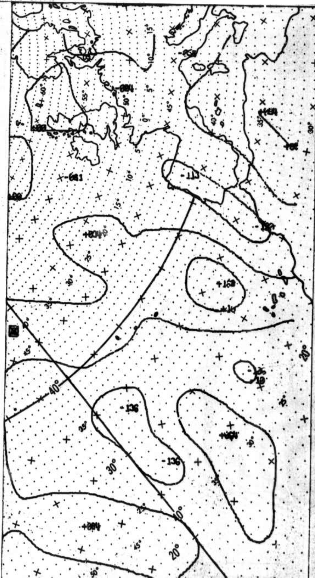
Figure 11 0°W 850° Atlantic
