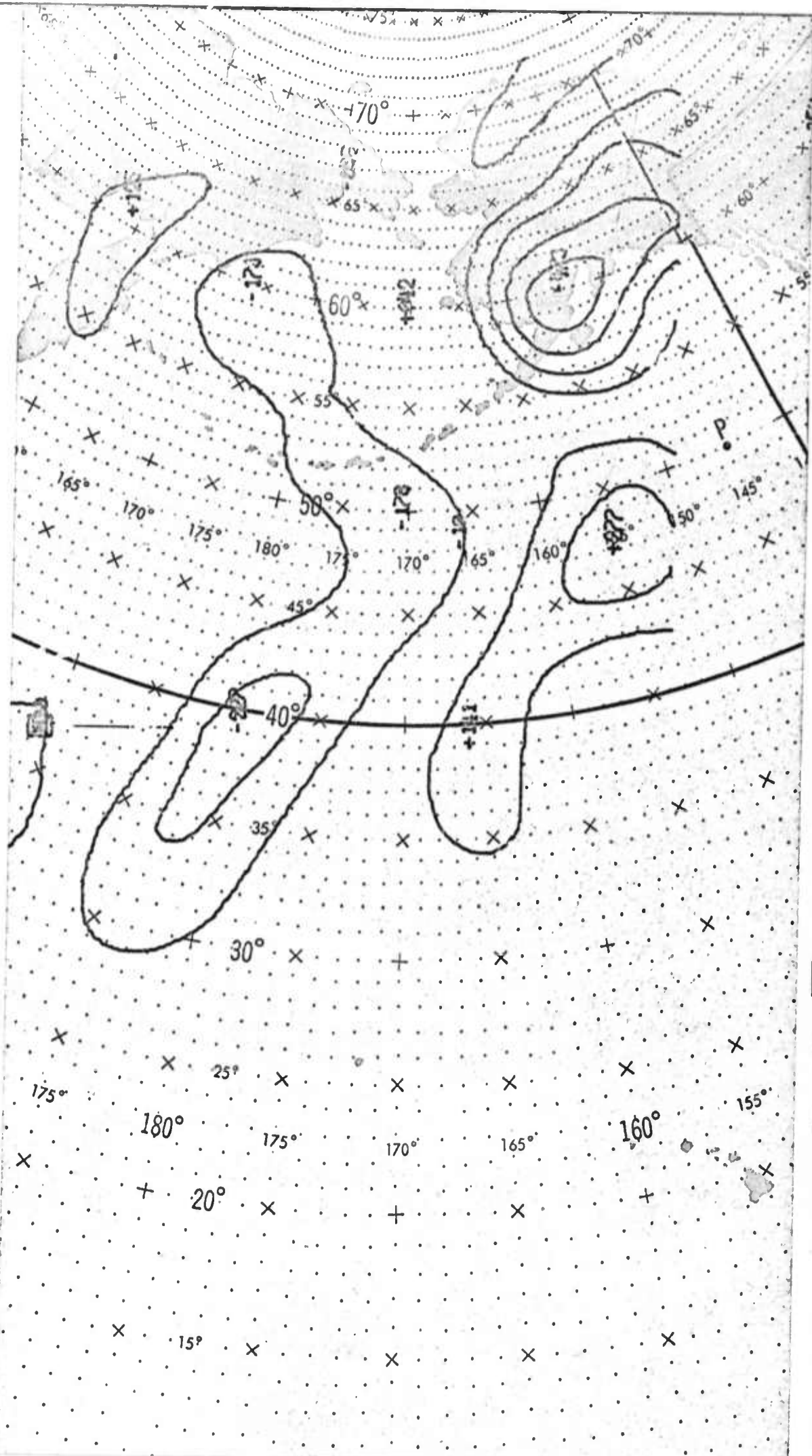
Figure 16 \overline{\sigma\omega} 850' Pacific
