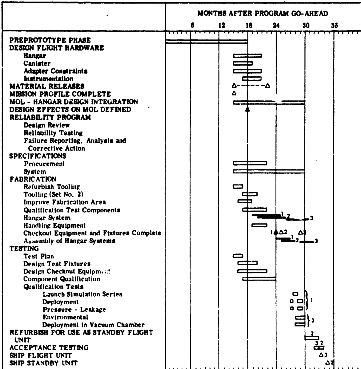
Figure 15. Space Maintenance Hangar Flight Hardware Plan and Schedule
