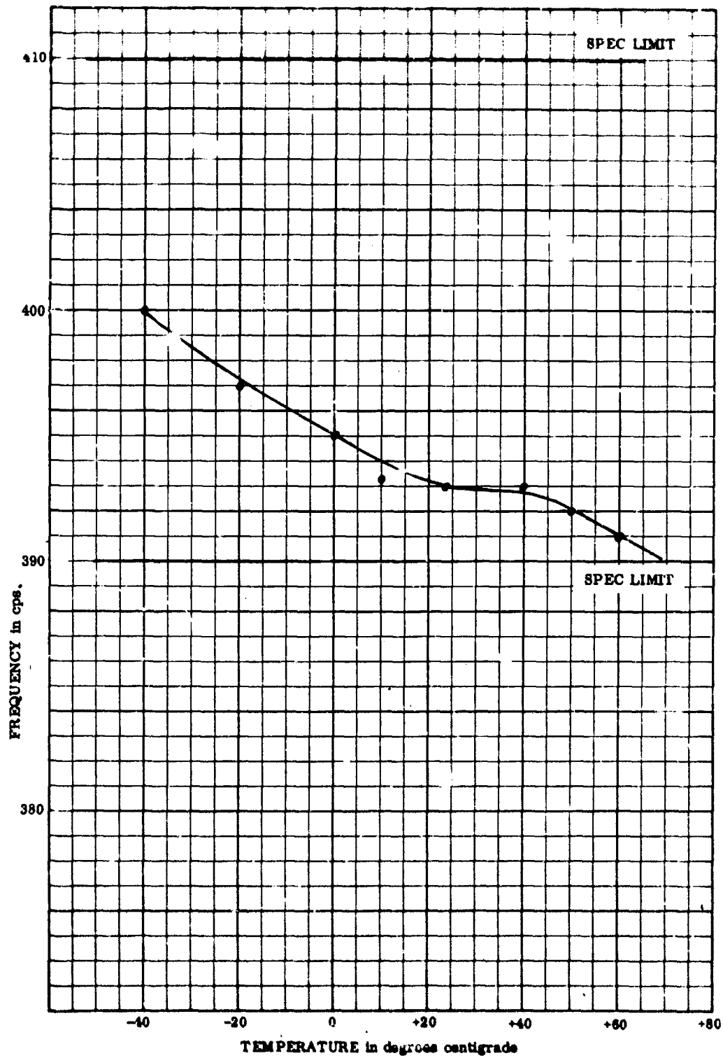
Figure 19. Glide Slope Tone Frequency vs Temperature
