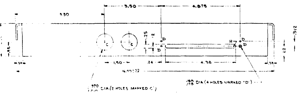
Figure A-60. Shelf (E2205251)
