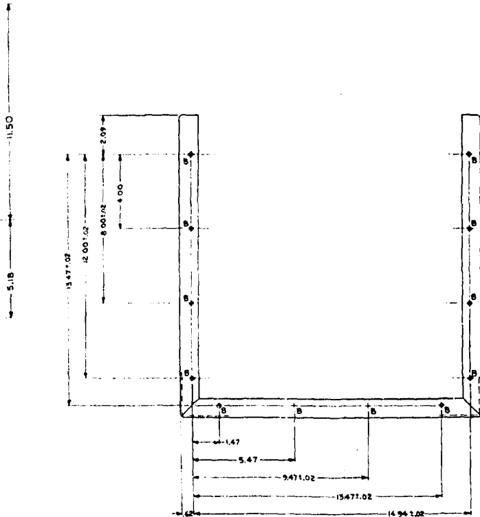
VIEW B-B
