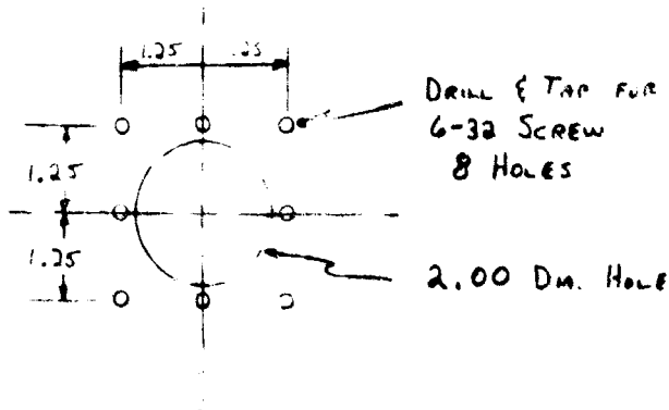
Hole Detail 'C'
