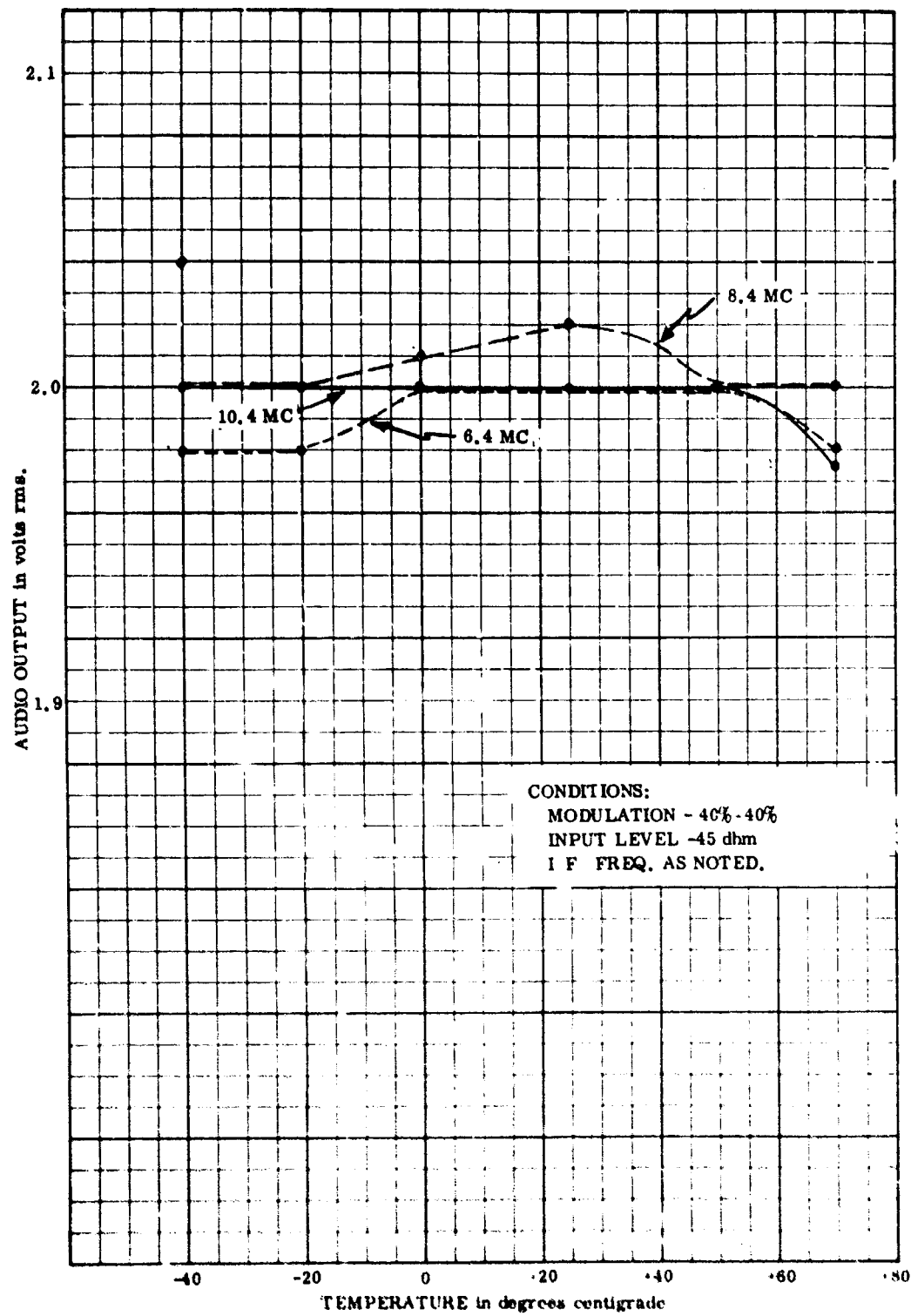
Figure 13. Slide Slope IF Output vs Temperature
