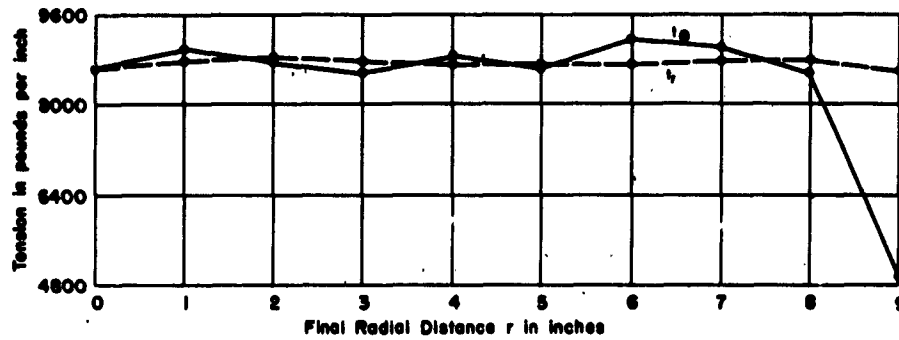
Figure 9e - Pressure p = 1000 Pounds per Square Inch; s_0 = 3.1561 Inches
