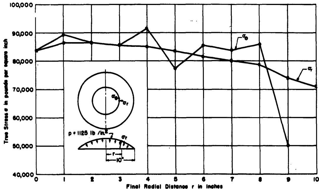
Figure 10 - Radial and Circumferential Stresses
