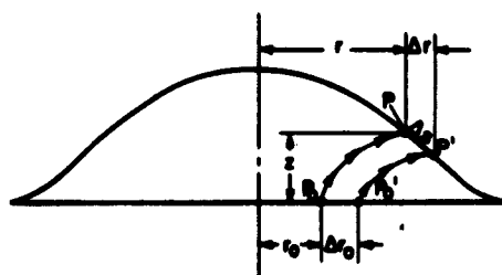
Figure 2 - Displacement of an Element P_0 P'_0 P and P' are fixed points on the plate.
