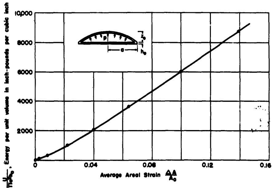
Figure 14 - Energy Plotted against Average Areal Strain
