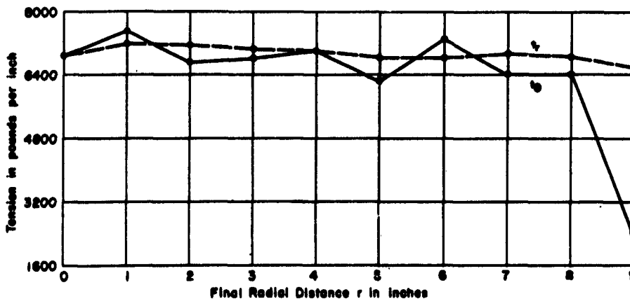
Figure 9b - Pressure p = 400 Pounds per Square Inch; s_0 = 1.495 Inch
