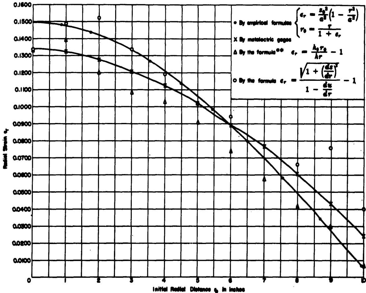
Figure 3 - Radial Strain Plotted on a Basis of Initial Radial Distance
