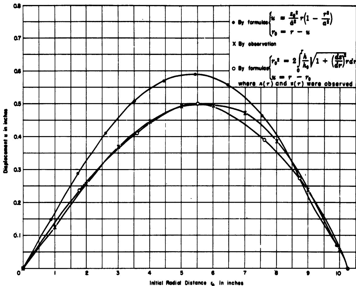
Figure 5 - Radial Displacement Plotted on a Basis of Initial Radial Distance
