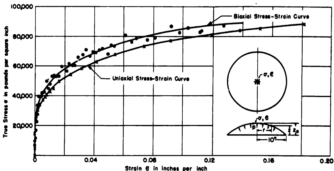
Figure 11 - Comparison of Uniaxial with Biaxial Stress-Strain Curve Stresses were computed at the center of the plate by the formula t = (-p/2)(d^2z/dr^2) , where t is the tension and h the thickness at the center of the plate. The pressure p(s_0) , the strain \epsilon(s_0) at center, and the profile function z(s_0, r) were obtained by measurement.
