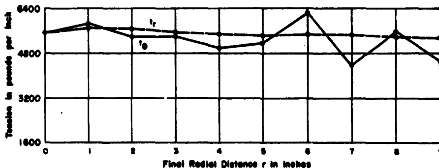
Figure 9a - Pressure p = 200 Pounds per Square Inch; s_0 = 0.9282 Inch
