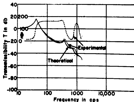
Figure 8 - Superposition of Theoretical and Experimental Curves of Transmissibility T in db and Phase in degrees versus Frequency in cps
