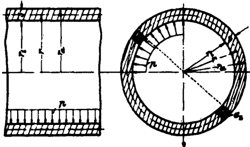
Figure 10 - Designations for the Frameless Tube of Infinite Length
