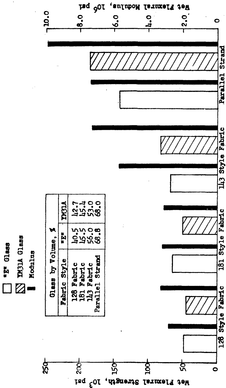
Figure 6 - Effect of Reinforcement Structure on Wet Flexural Properties of "E" and IM31A Glass Laminates
