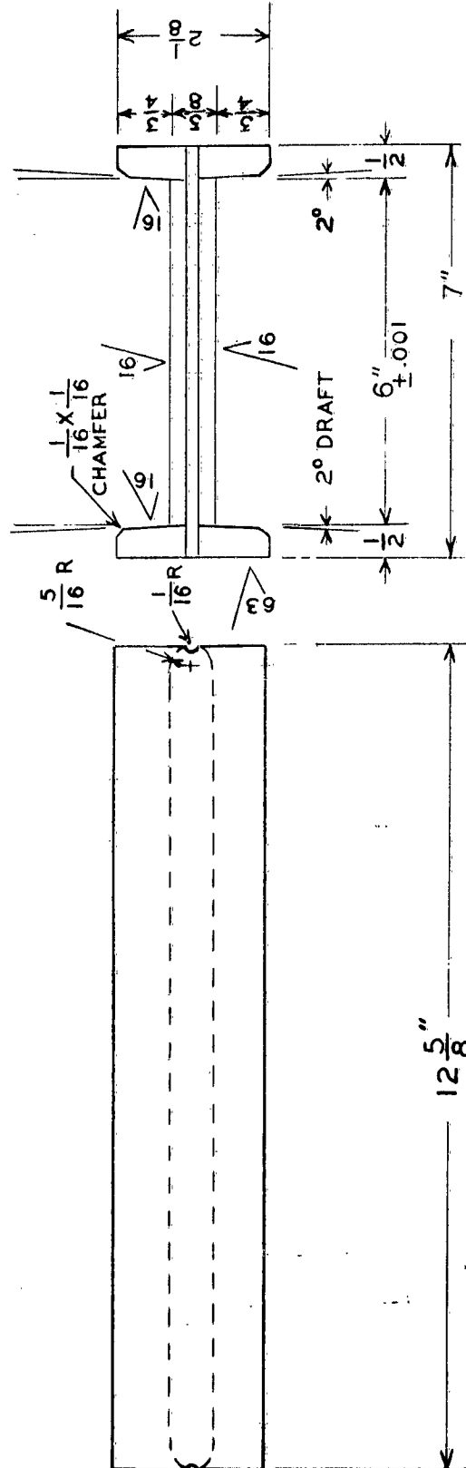
Figure 15 - Parallel Strand Specimen Mold: Double Female Section ( 1 required)
