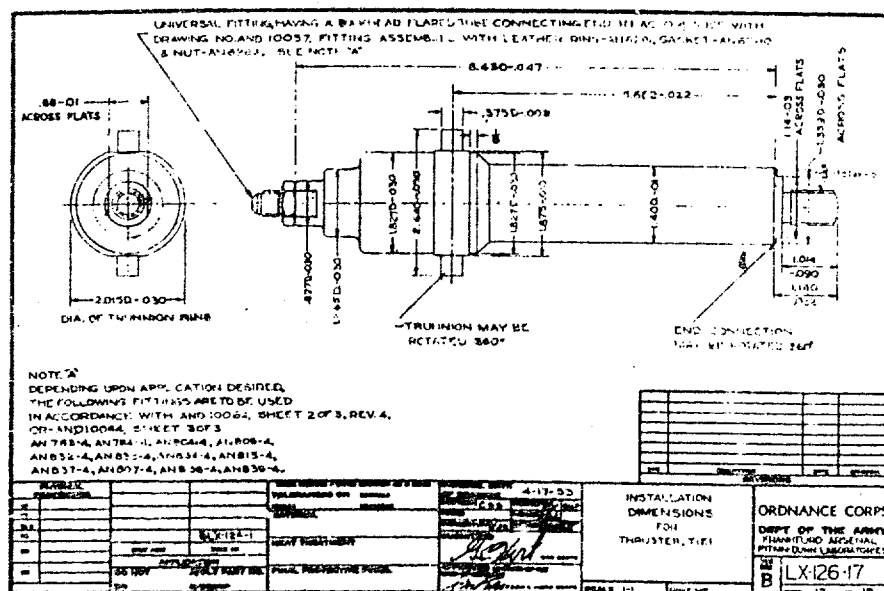
Figure 7. Thruster, T1E1 A - Assembly B - Installation dimensions
