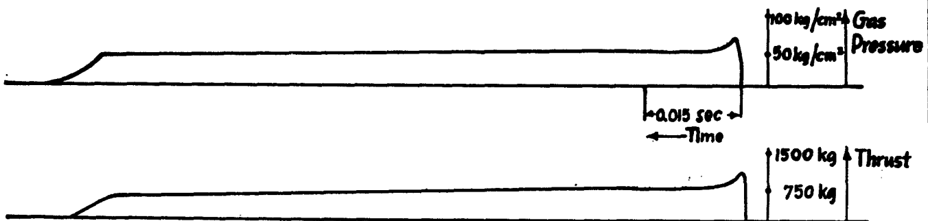
Figure 5 — Smooth Burning
