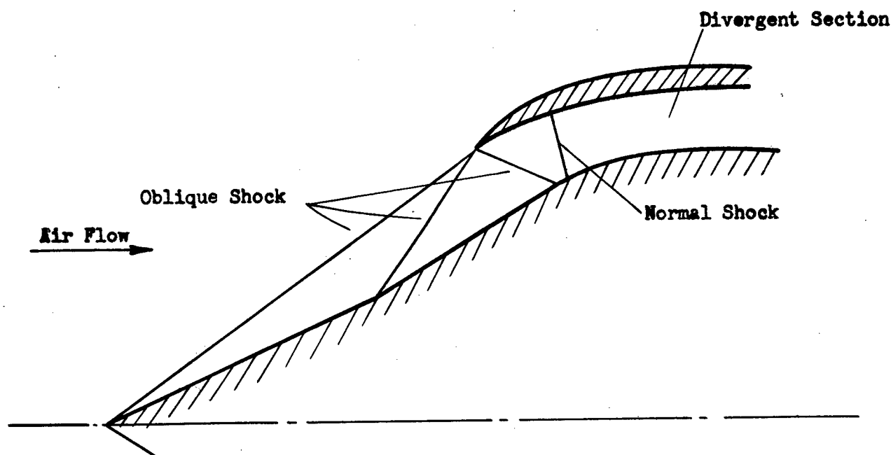
Figure 3 — Oswatitsch Diffuser
