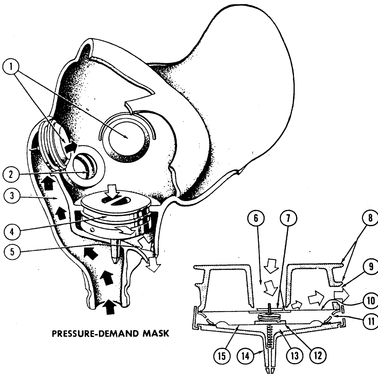
EXHALATION VALVE DETAILS
