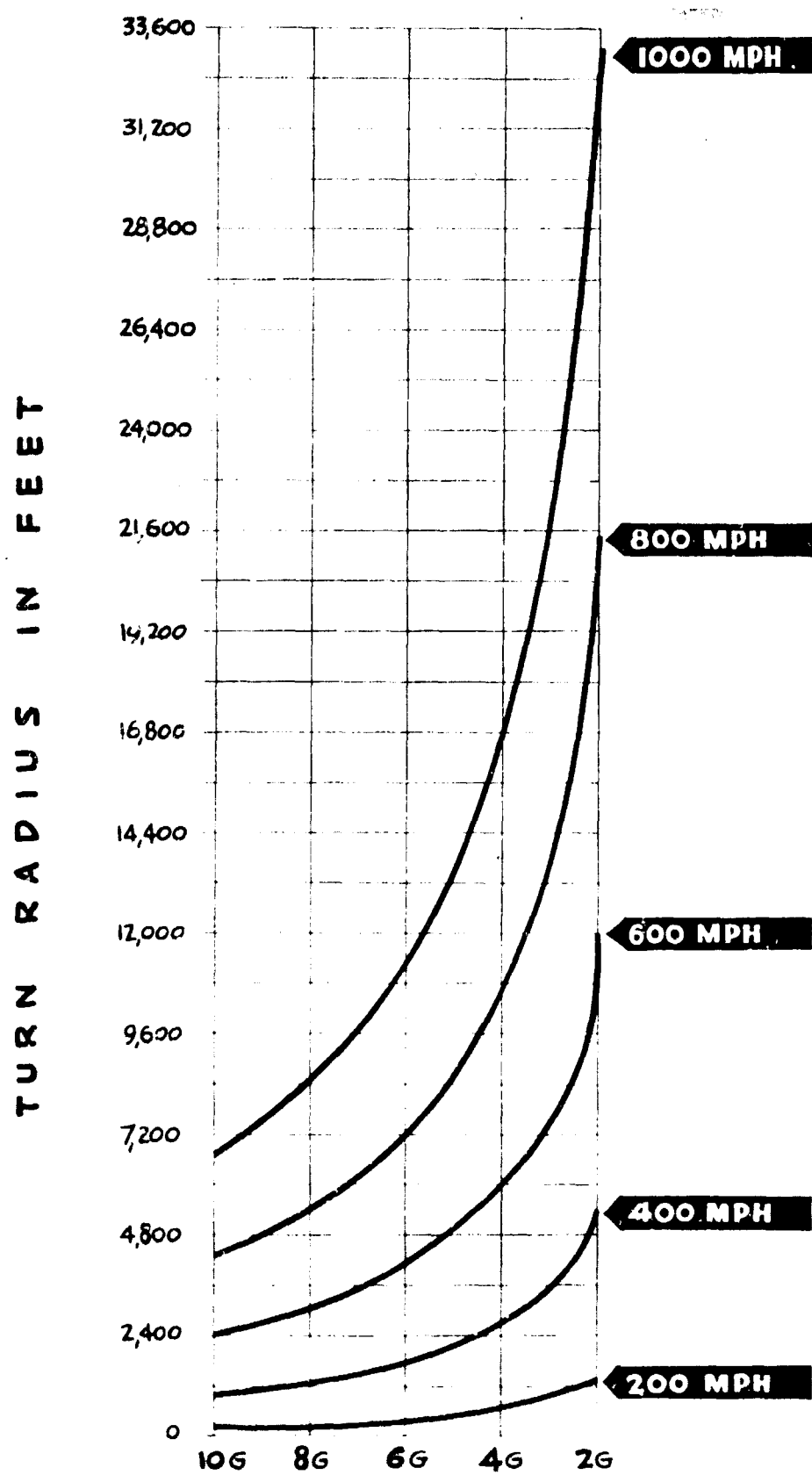
Figures 10 & 11 — "G" Force Resulting from Various Radius of Turn with Constant Speed
