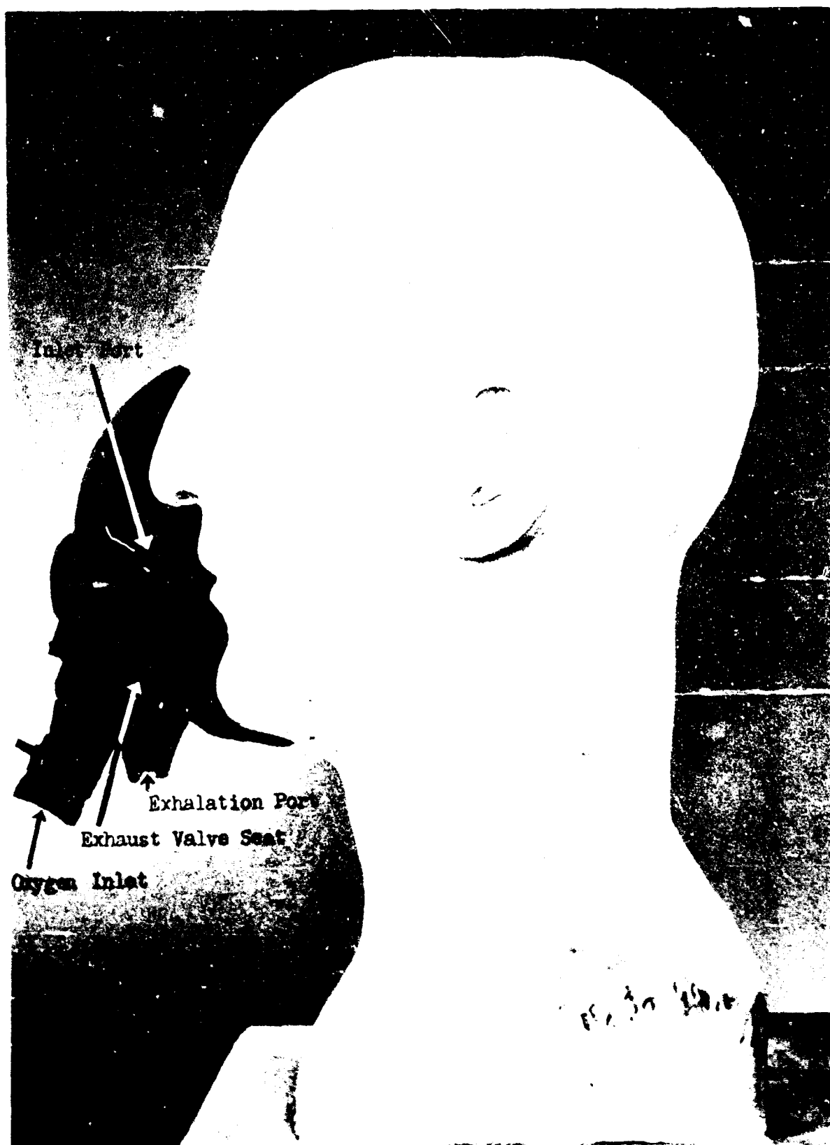
Figure 34 — Fit of Oxygen Mask on face
