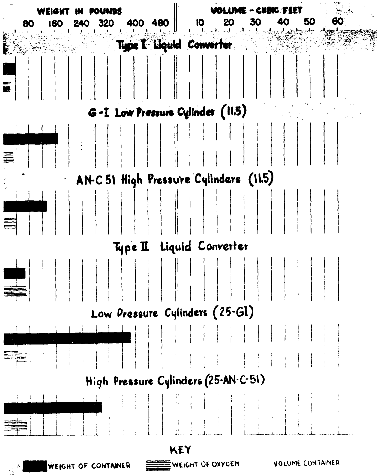
Figure 20 — Relative Weights of Gaseous and Liquid Oxygen Containers
