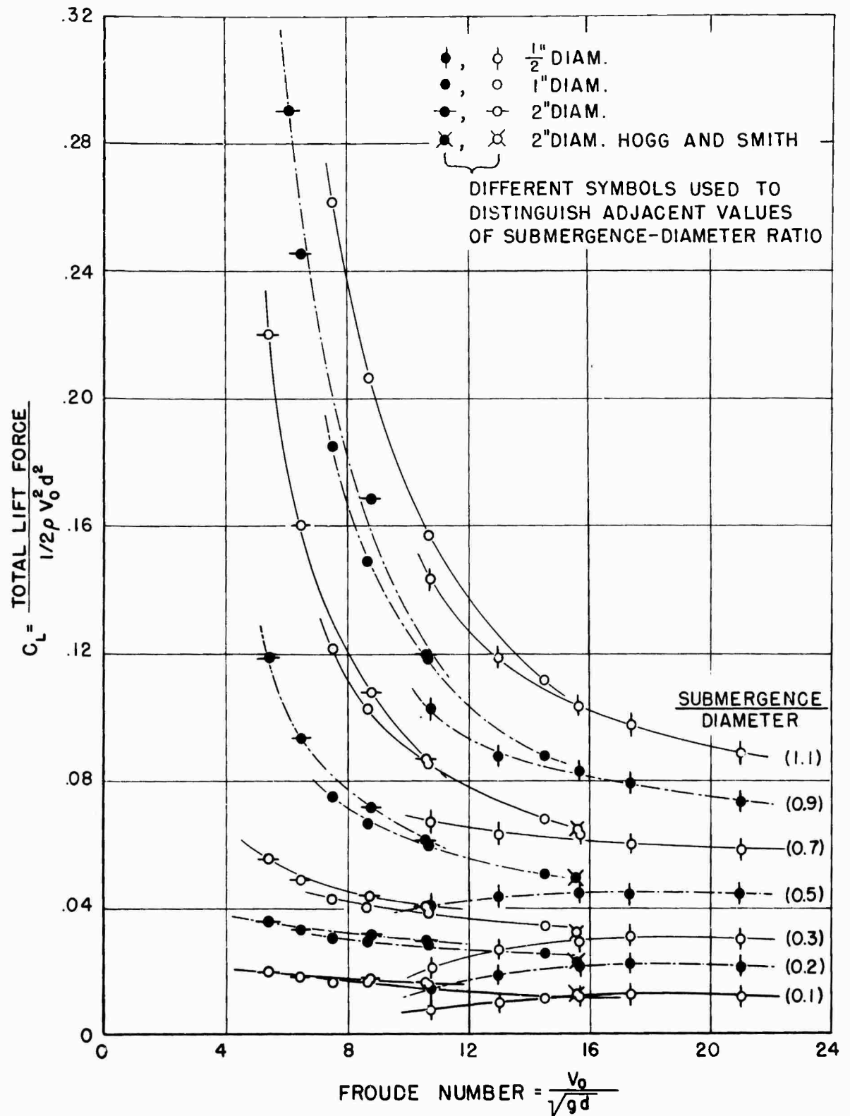
Fig. 6 - Plot of lift coefficient vs. Froude Number for hollow cylinders planing on water. Angle of attack \alpha = 4.5^\circ .
