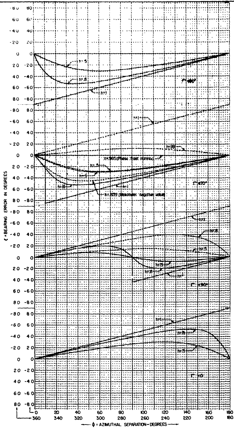
ADCOCK AND PHASE FRONT NORMAL (DOTTED) RDF BEARING ERROR
