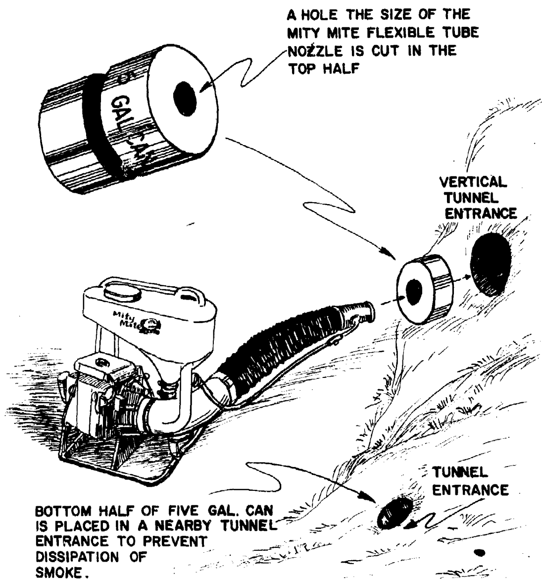
FIELD EXPEDIENT METHOD USING 5 GALLON CAN
