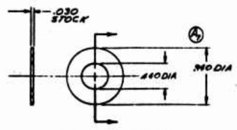
-3 RING DETAIL
