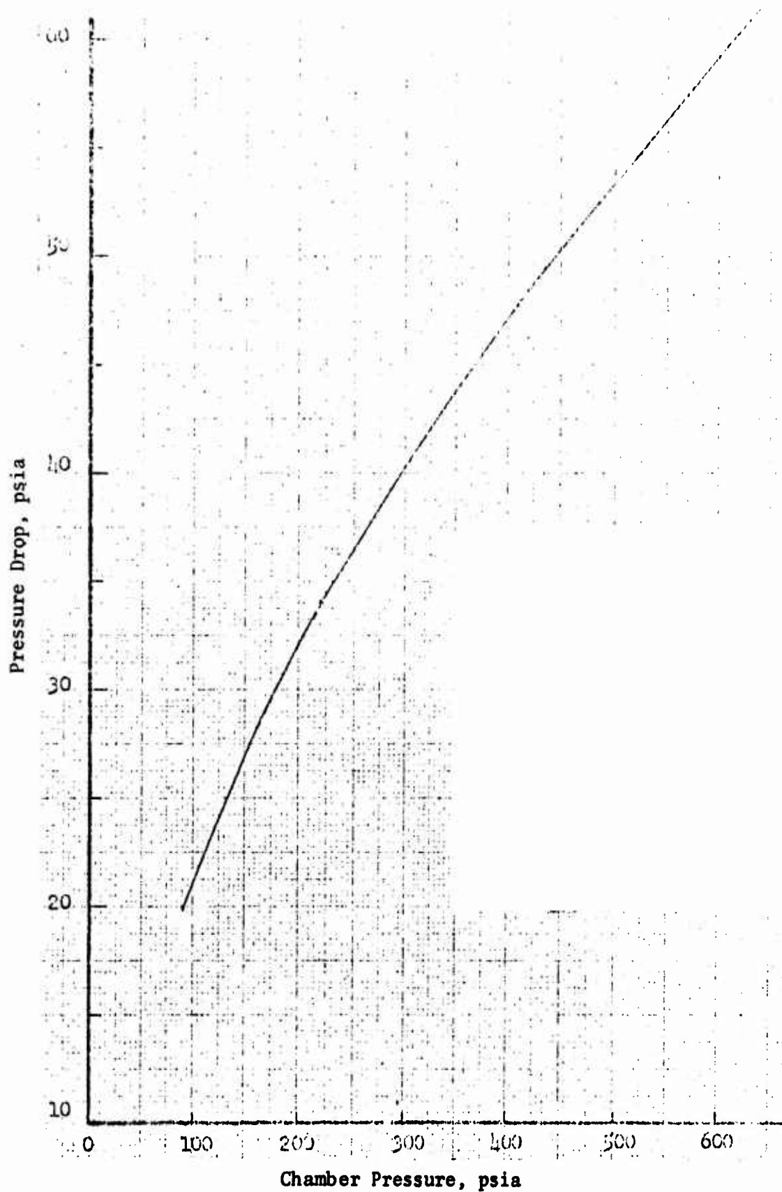
Figure 60. Nozzle Extension Tube Assembly Pressure Drop (U)
