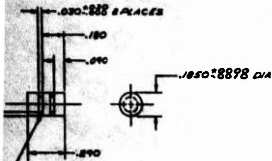
⑤-3 PLUG DETAIL SCALE 4/1
