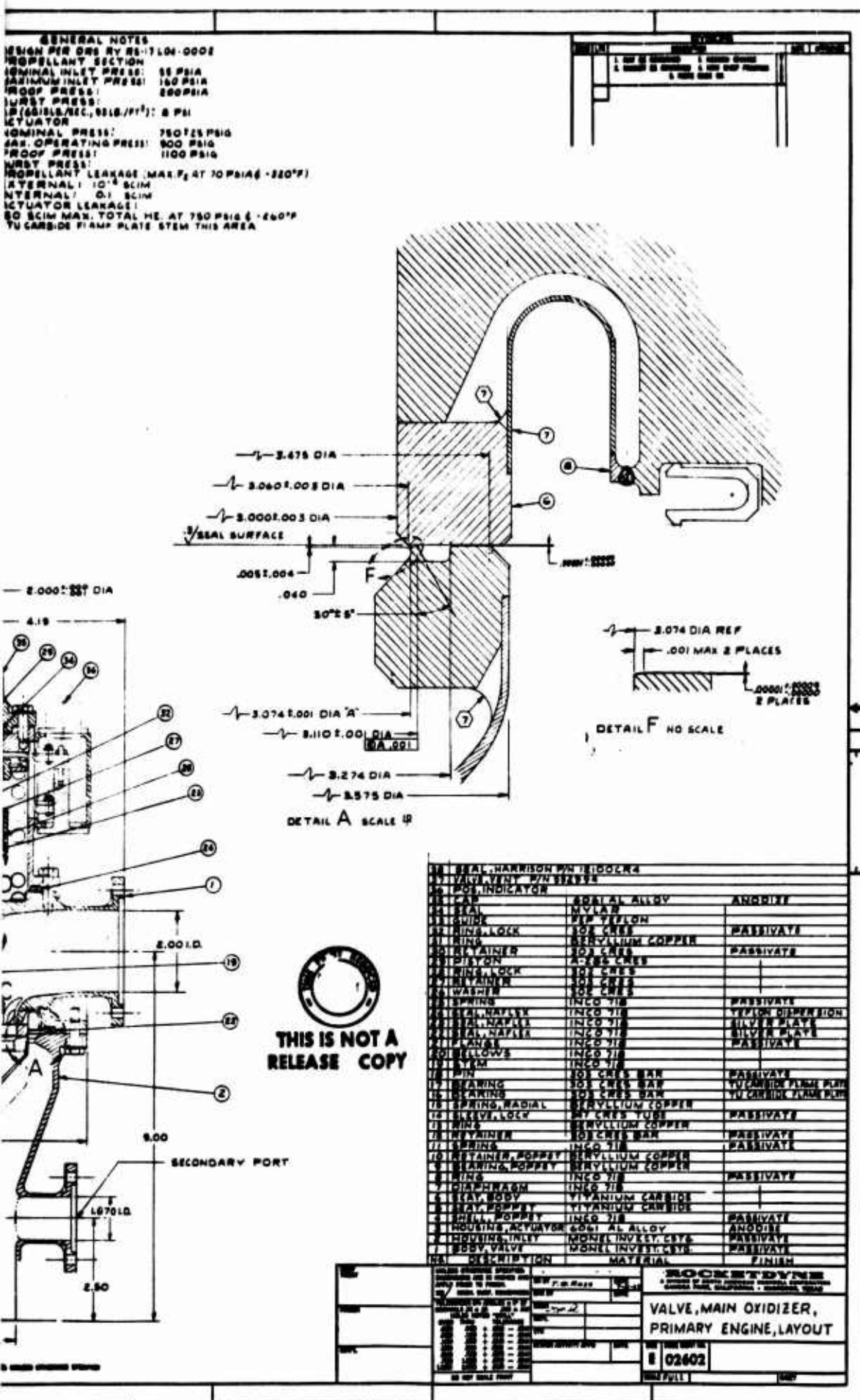
Figure 25. Main Engine Oxidizer Valve (U)
