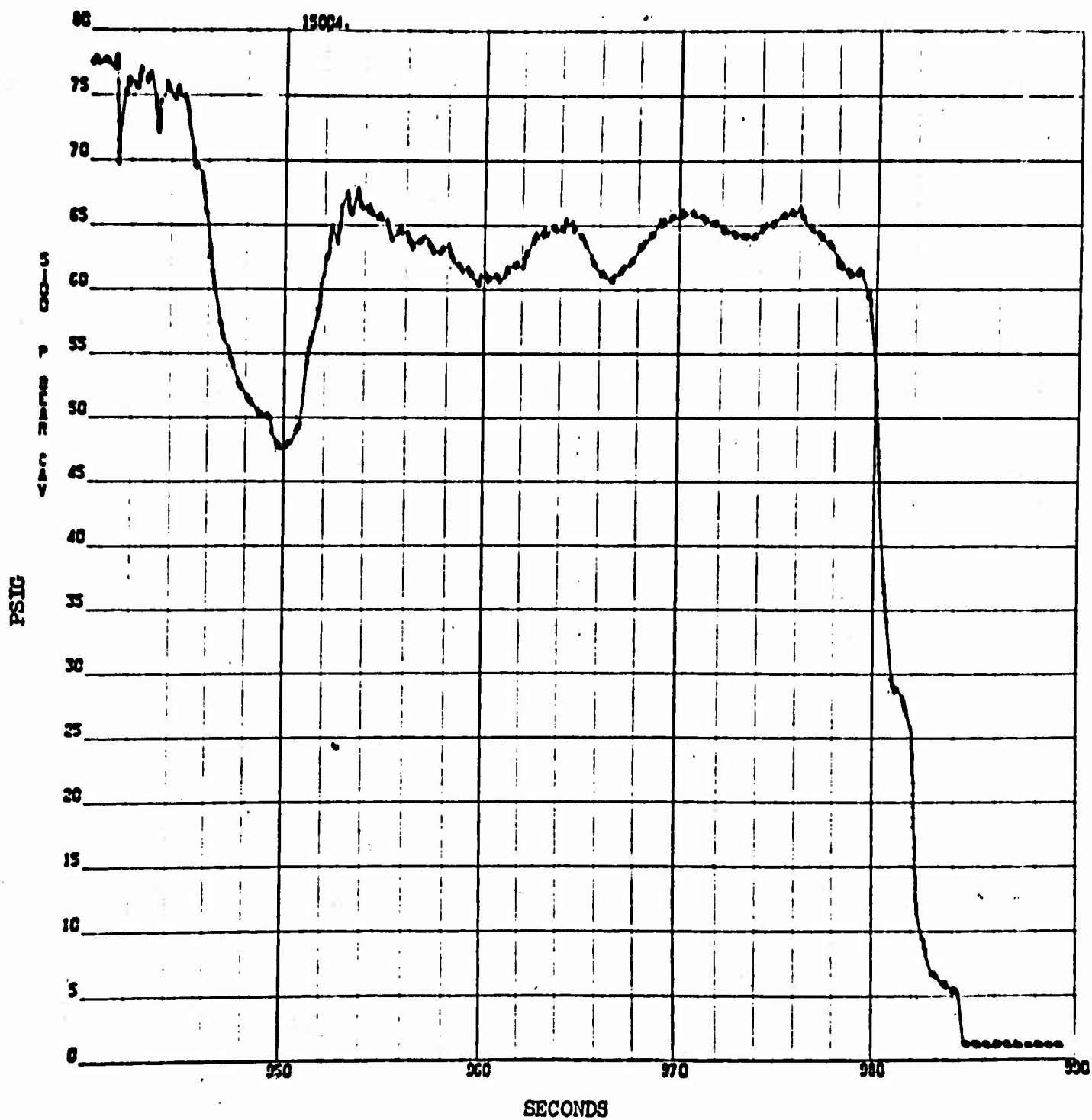
Figure 73. Test 004: 940 to 990 Seconds, Last 50 Seconds; Bearing Cavity Pressure (C)
