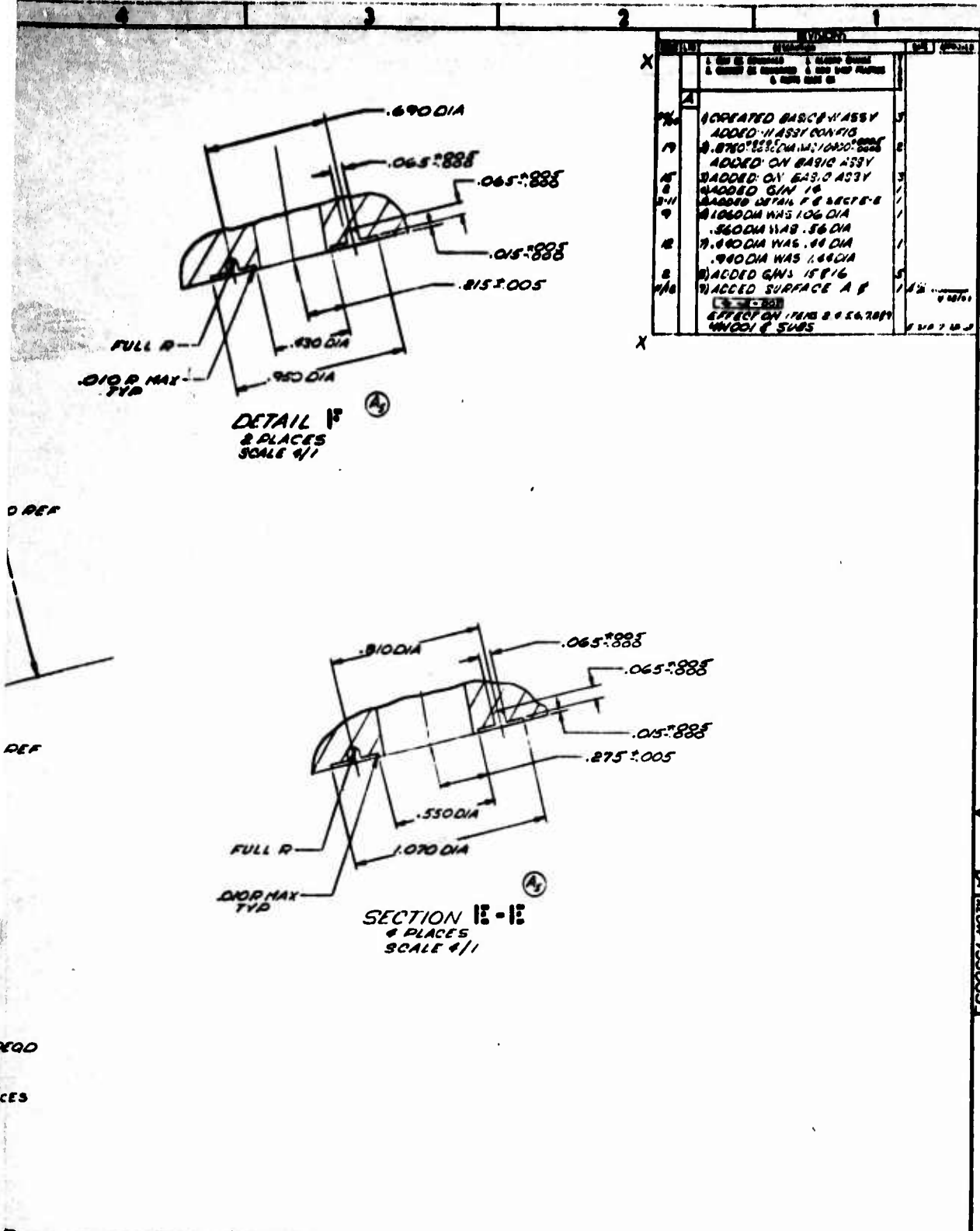
Figure 46. Prototype Segment Assembly (U)
