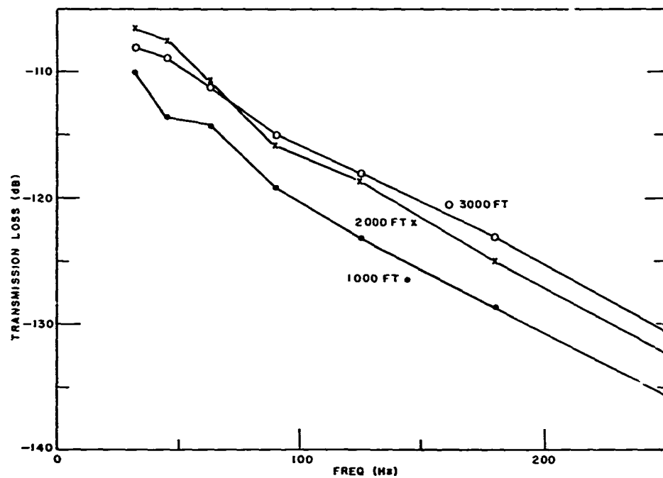
Fig. 36. HW 1A, Lady Lana DSS, Mk 59 4 lb TNT, range 3264.1 n.m.
