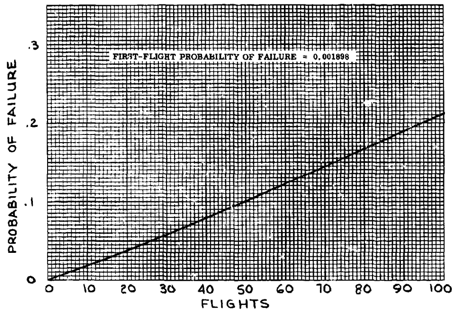
Figure 6-8 Reusable Launch Vehicle (LO 2 /LH 2 ), Mission I, Autogenous Pressurization, Regulator Controlled (C)
