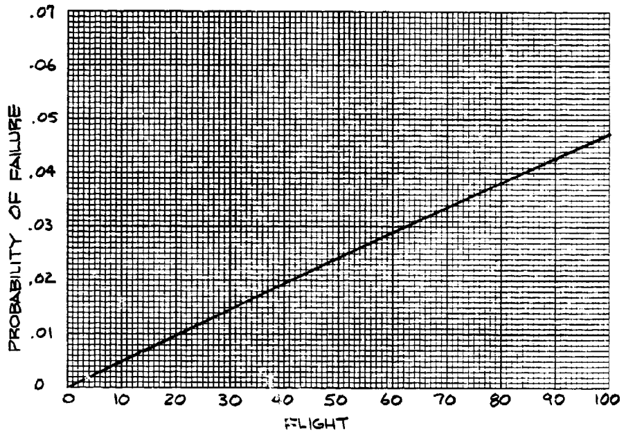
Figure 6-10 Reusable Launch Vehicle ( \text{LO}_2/\text{LH}_2 ), Mission I, Propellant Utilization, Capacitance Gaging (C)
