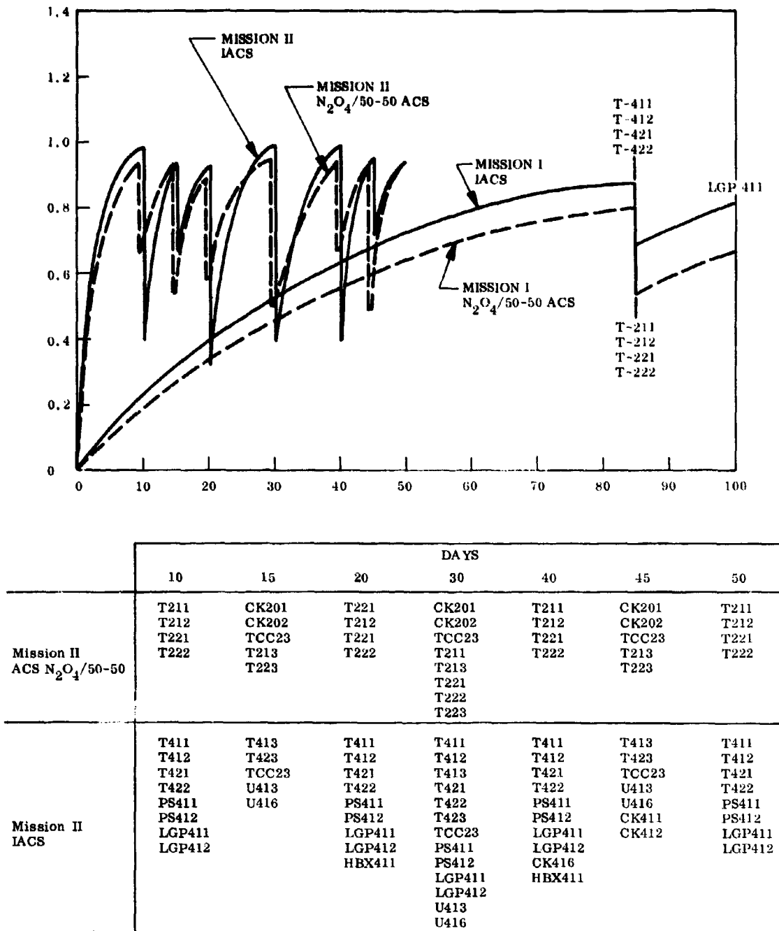
Figure 7-3 Comparison of Reusable Launch Vehicle Attitude Control Subsystems (U)
