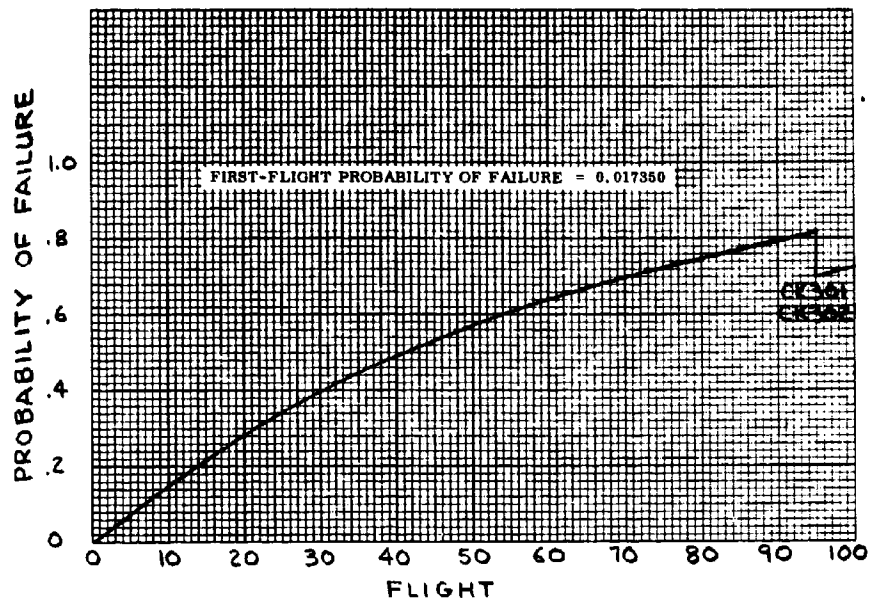
Figure 6-59 Cryogenic Spacecraft ( LF_2/LH_2 ), Mission IV, Attitude Control System, Nonintegrated 2 (C)
