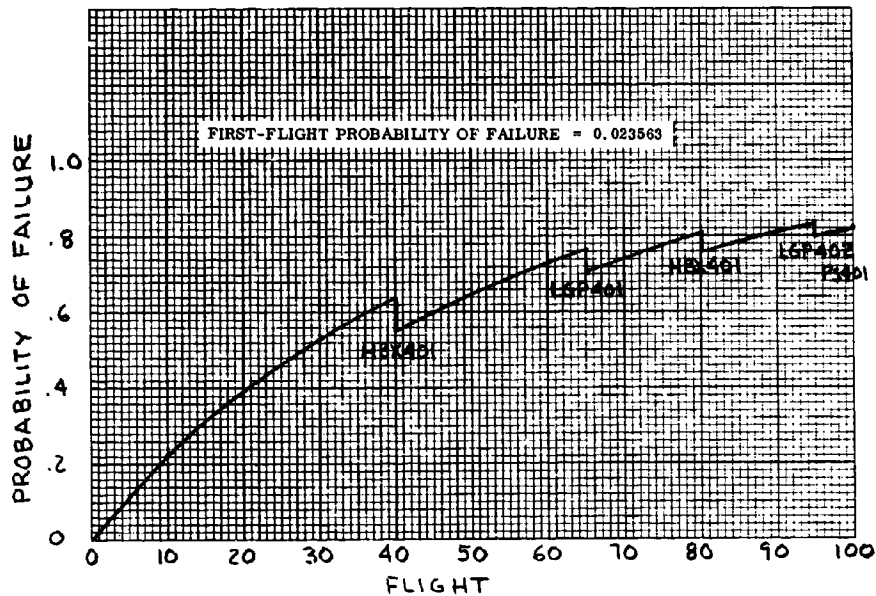
Figure 6-60 Cryogenic Spacecraft ( LF_2/LH_2 ), Mission IV, Attitude Control System, Integrated 2 (C)
