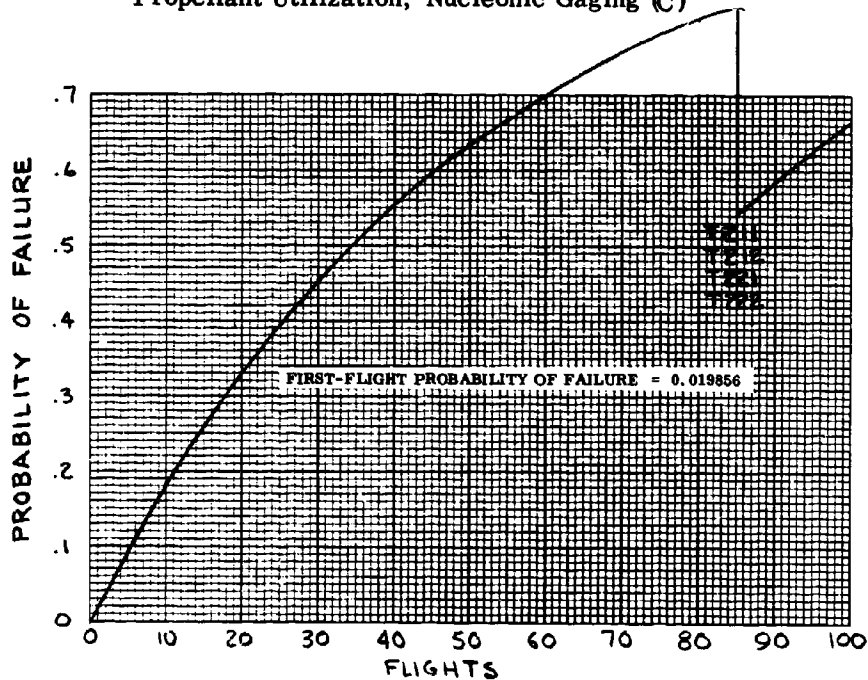
Figure 6-14 Reusable Launch Vehicle ( LO_2/LH_2 ), Mission I, ACS System, Nonintegrated (C)
