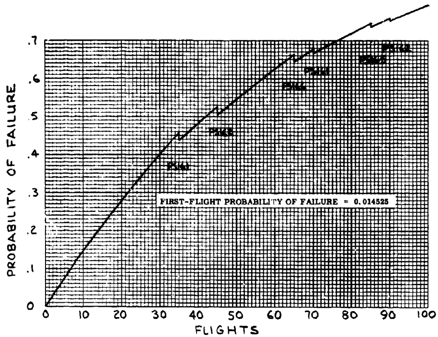
Figure 6-9 Reusable Launch Vehicle ( \text{LO}_2/\text{LH}_2 ), Mission I, Autogenous Pressurization, Valve Controlled (C)
