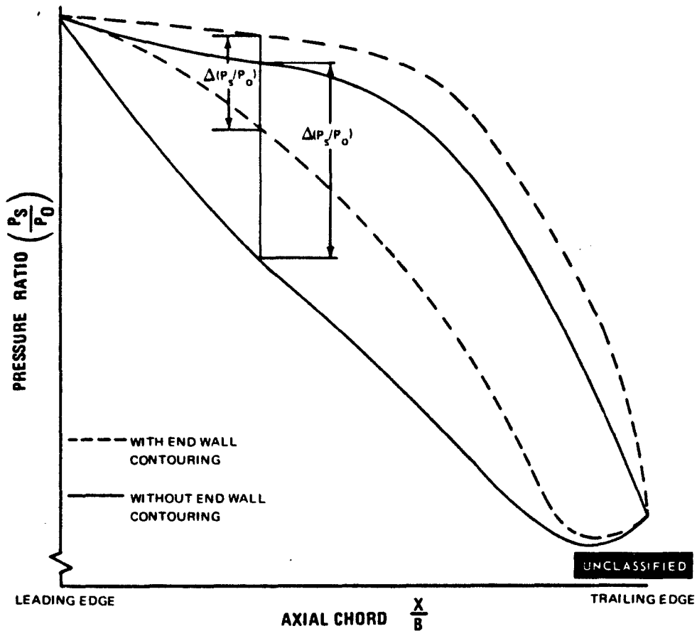
Figure 34 Pressure Distribution
