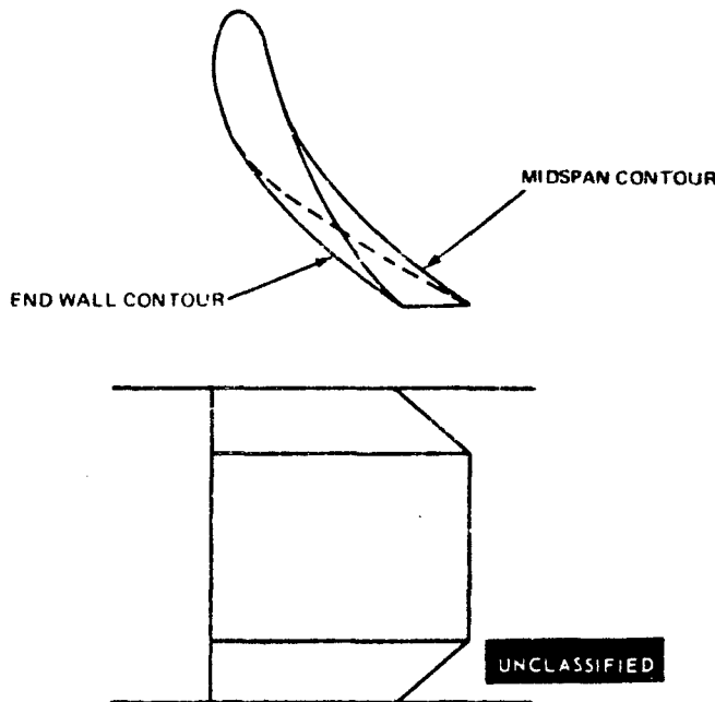
Figure 35 Local Uncambered Airfoil
