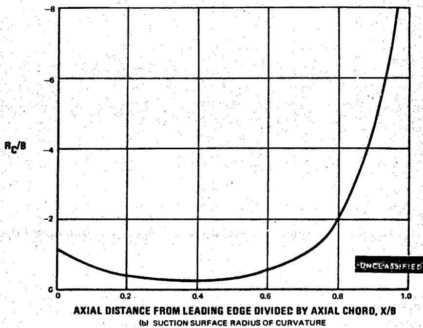
Figure 119 Medium Reaction, Medium Solidity, First Stage Blade, 1/4 Root Section
