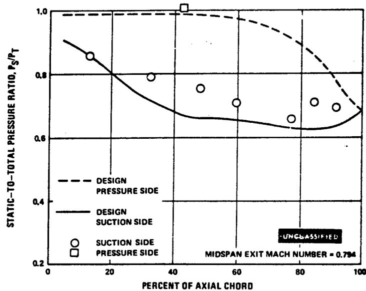
Figure 76 Static-to-Total Pressure Ratio vs. Percent of Axial Chord, First Vane Cascade – Tip Section, Inlet Screen Removed
