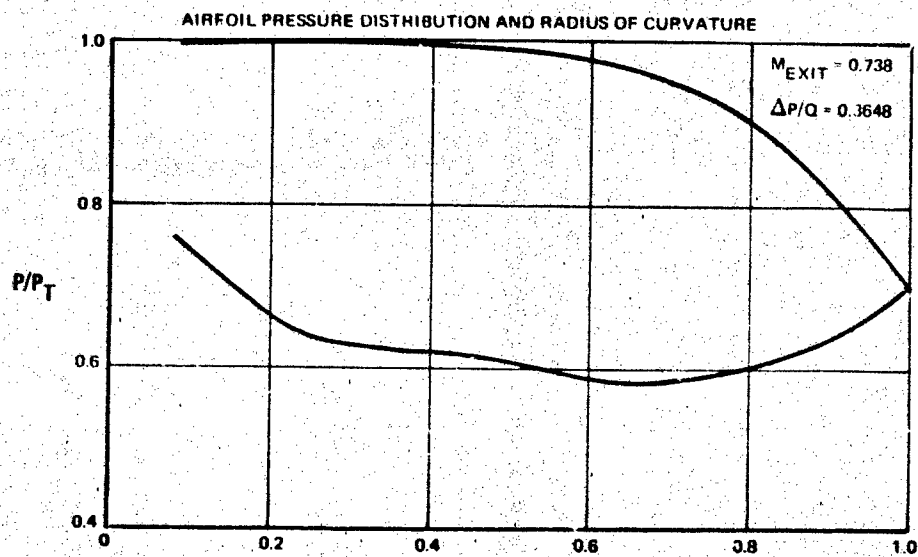
(a) AIRFOIL SURFACE PRESSURE DISTRIBUTION
