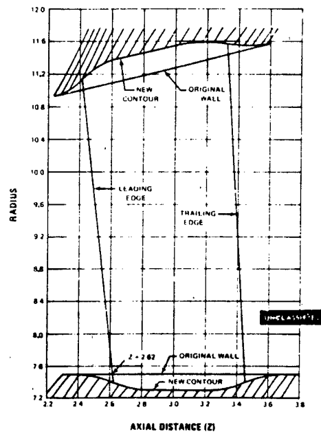
Figure 97 End-Wall Contouring, Second Stage Vane
