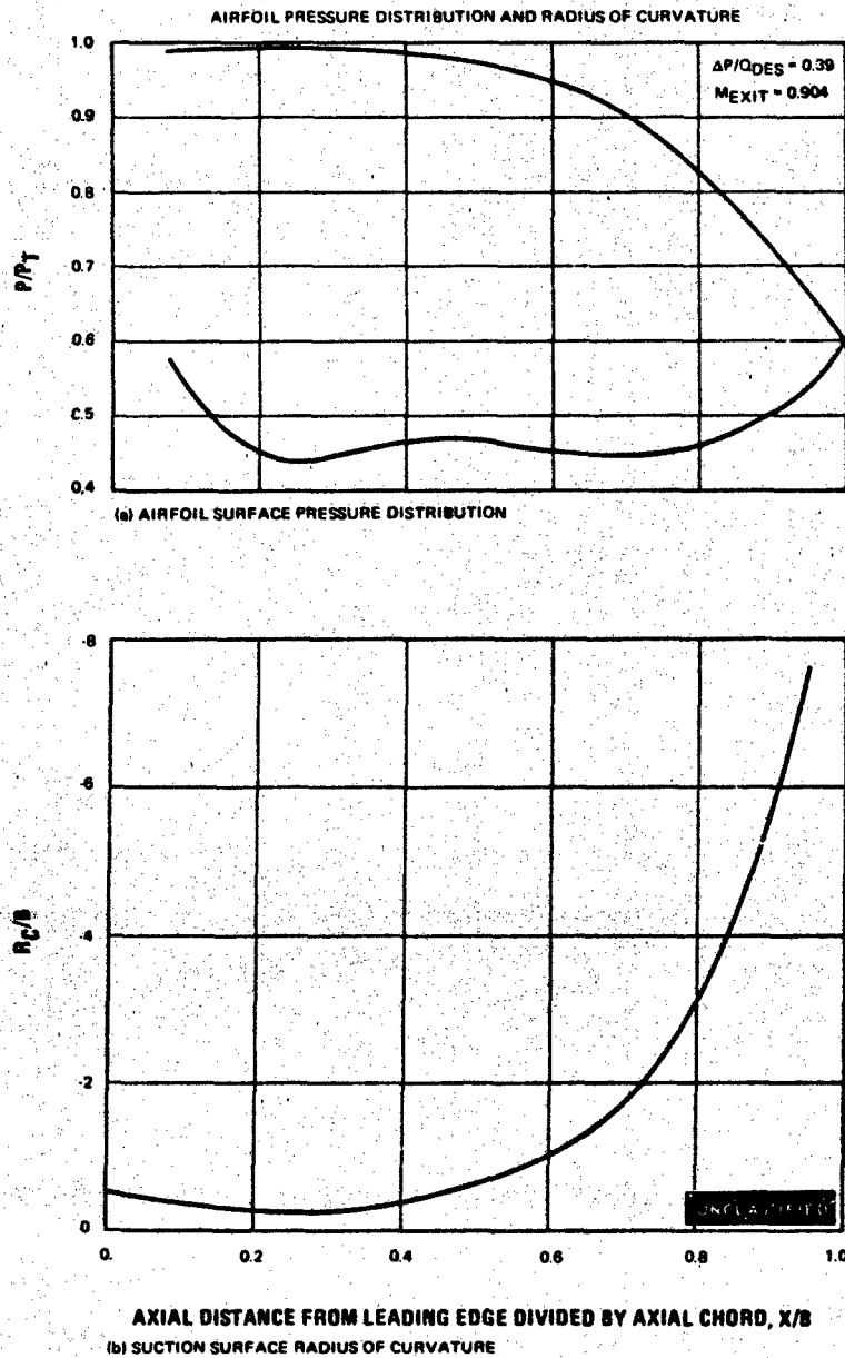
Figure 143 Medium Reaction, Medium Solidity, Second Stage Blade, Mean Section
