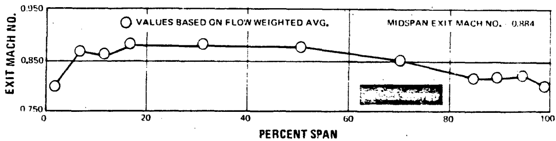
Figure 48 Spanwise Exit Mach Number Distribution, First Vane Screen Installed, Computed at Specified Intervals, Midspan Exit Mach No. = 0.884
