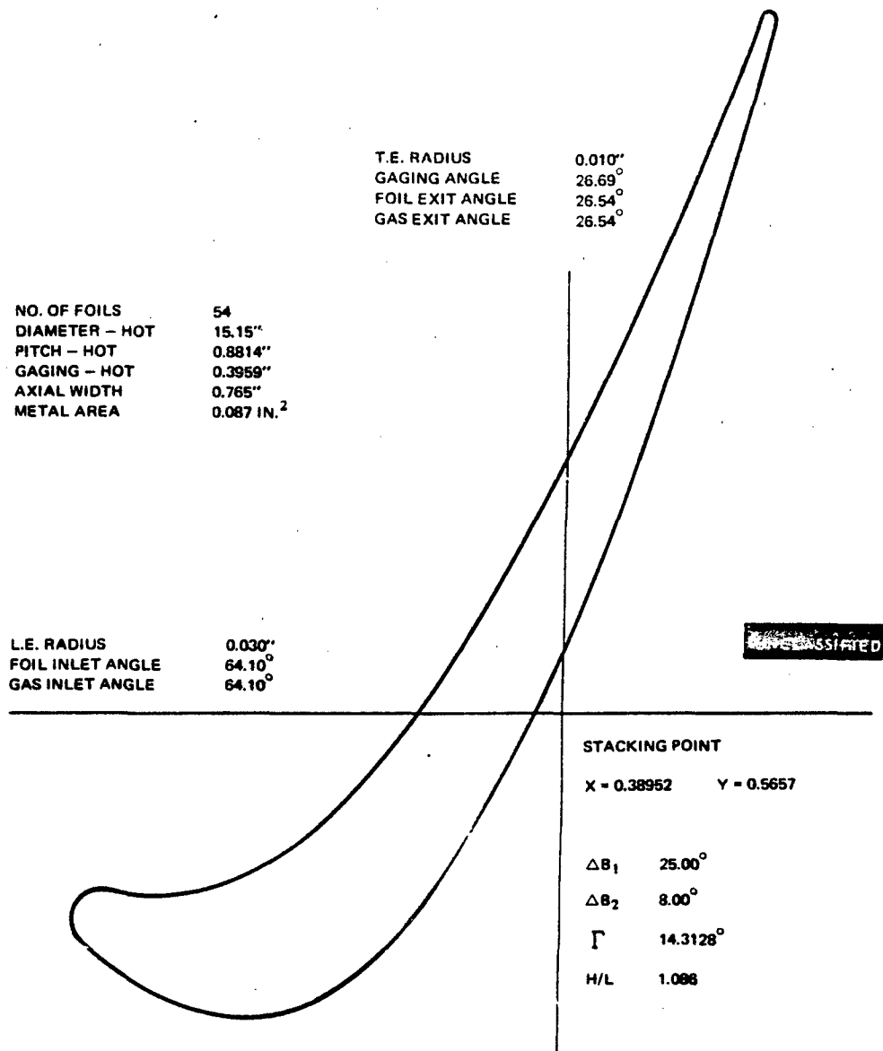
Figure 105 Medium Reaction, Medium Solidity, First Stage Vane, Root (F-F) Section
