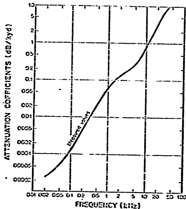
Figure k-7. Sound Attenuation. (B)
