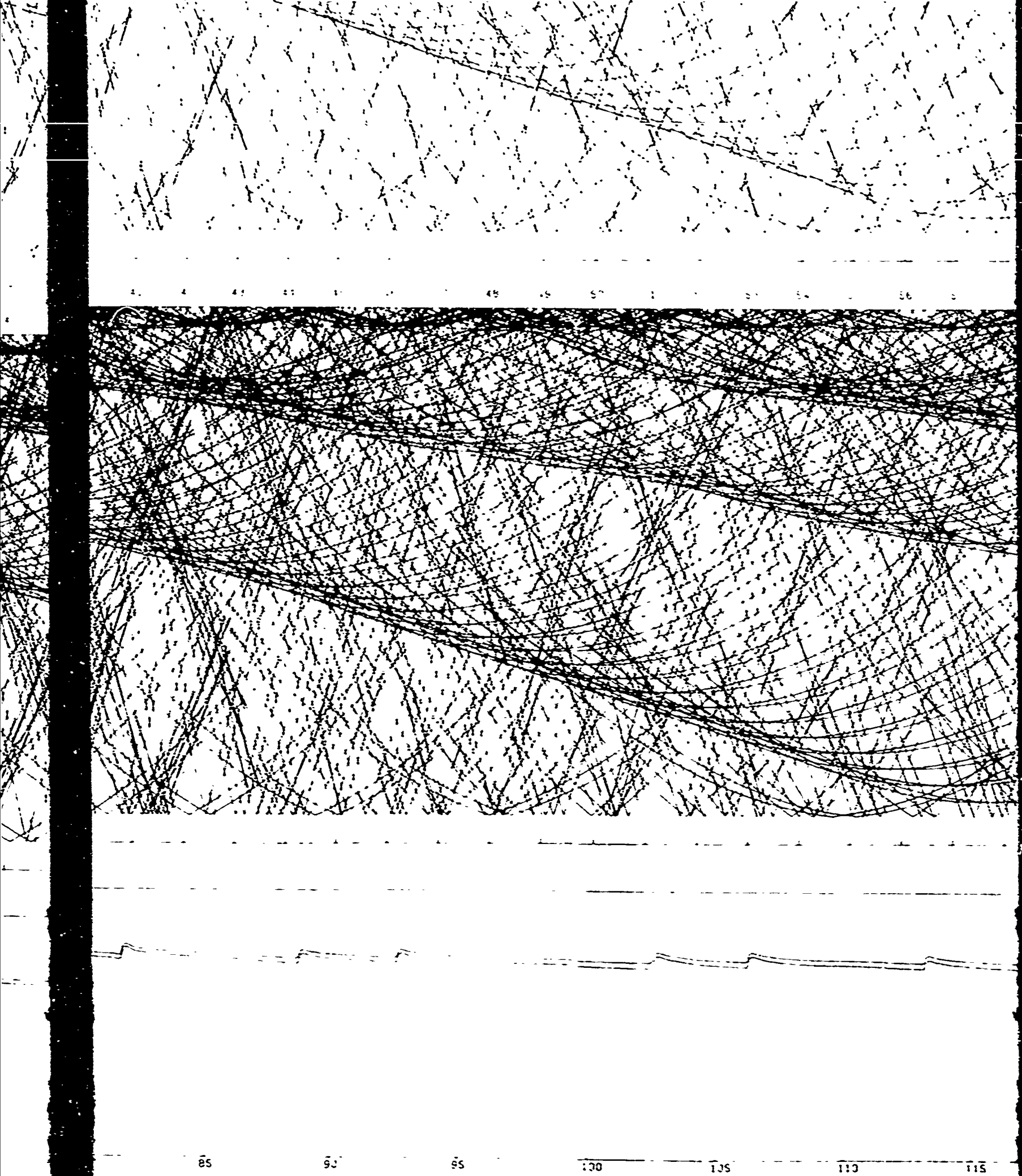
FIGURE 74. RAY PATHS AND TRANSMISSION LOSS -- EASTERN MEDITERRANEAN WINTER
