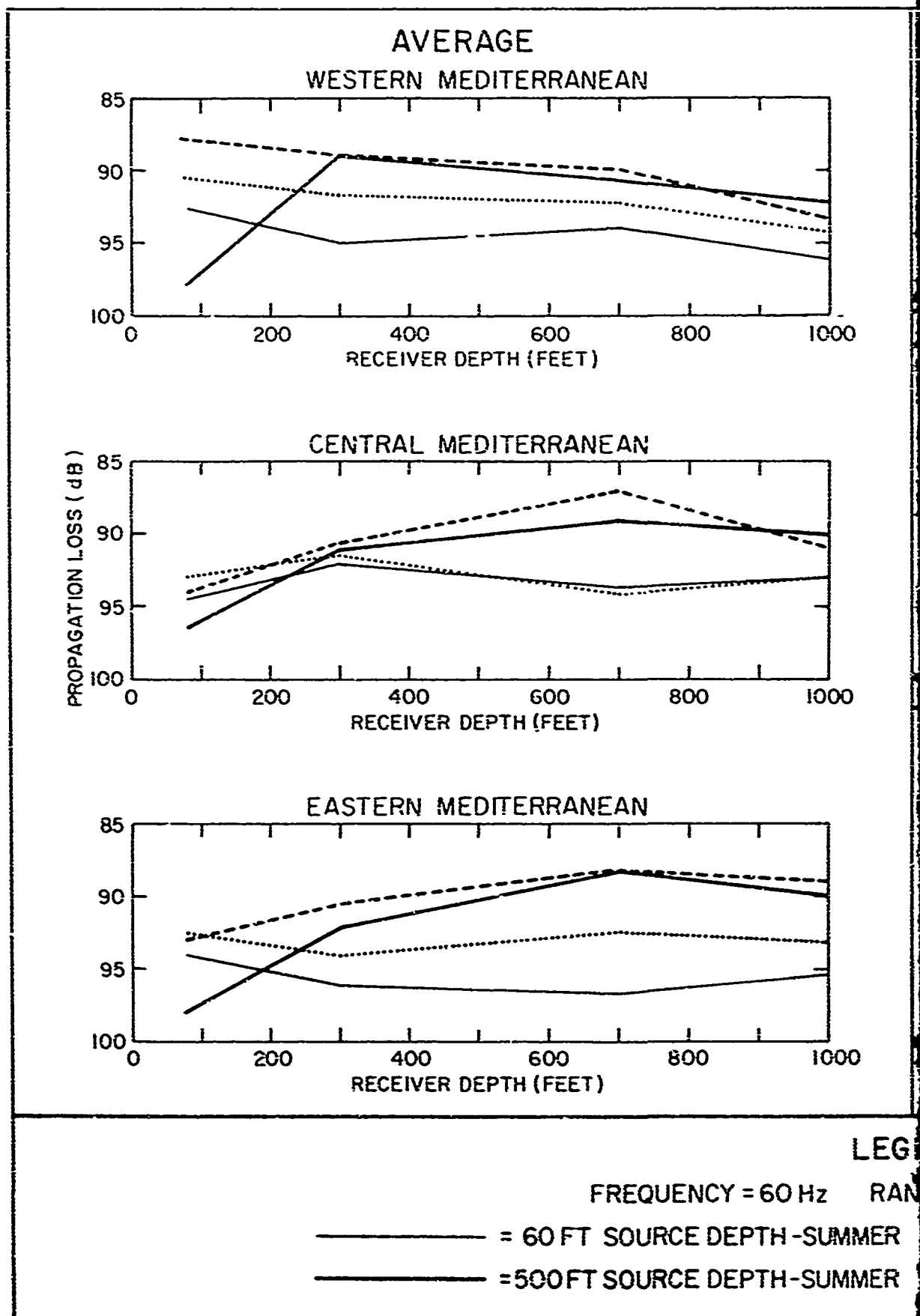
FIGURE 77. CALCULATED AVERAGE AND MINIMUM PROPAGATION LOSS -- WE
