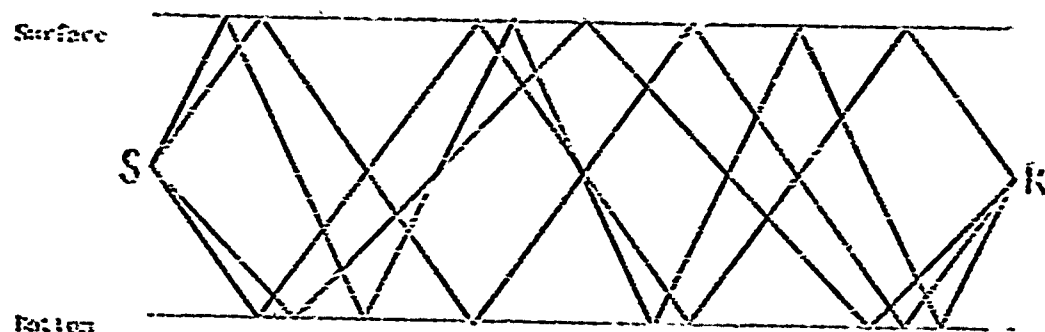
Figure A-4. Reflection of Sound Rays with Two Bottom Bounces (ii)
