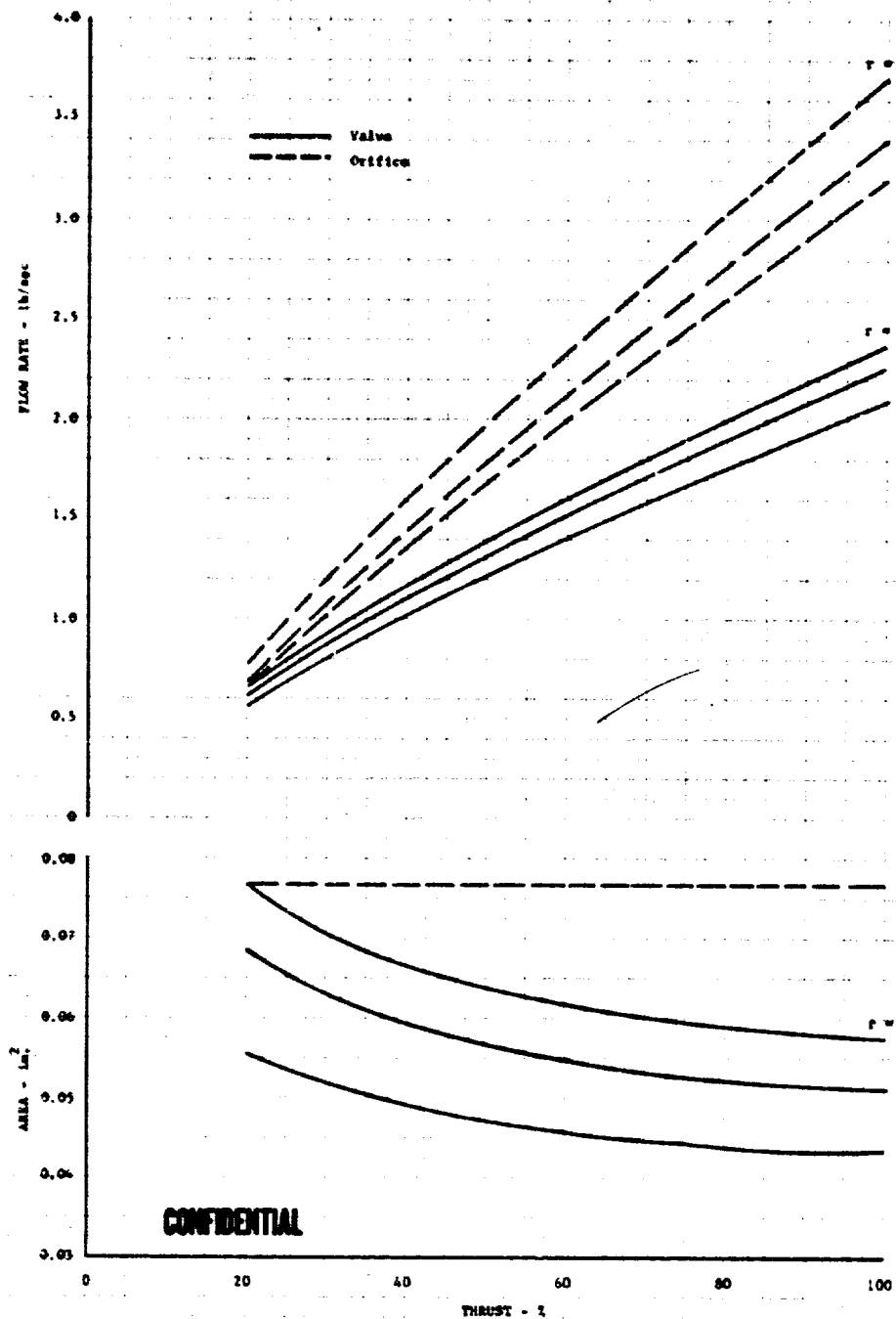
(U) Figure 26. Effect of Fuel Preburner Supply Tap-Off Location on Lightweight Heat Exchanger Coolant Valve
