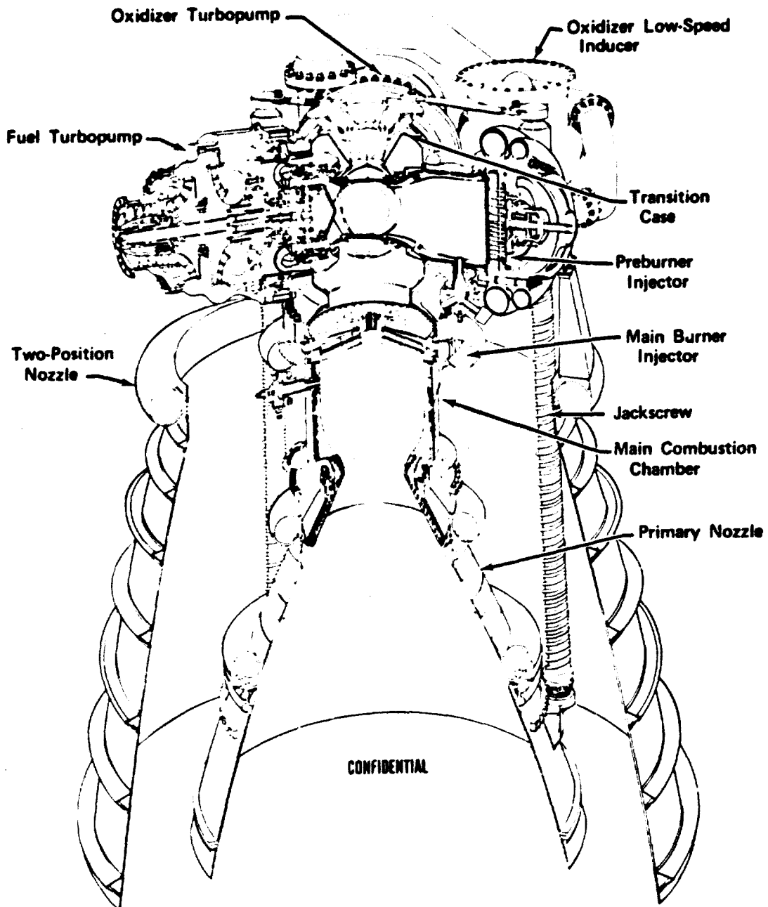
(U) Figure 14. XLR129-P-1 Demonstrator Engine
