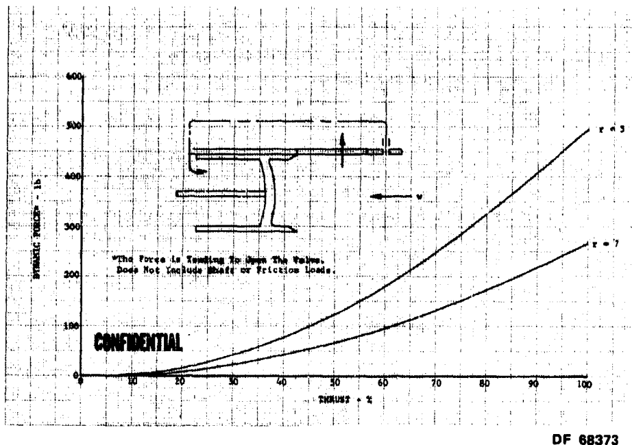
(U) Figure 450. Dynamic Force vs Thrust (Internal Sleeve Valve - Reverse Flow)
