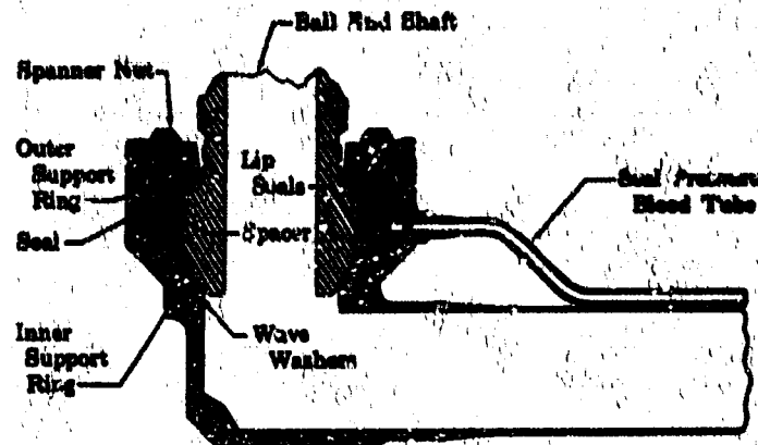
(U) Figure 514. Single Transfer Tube Assembly Ball Joint
