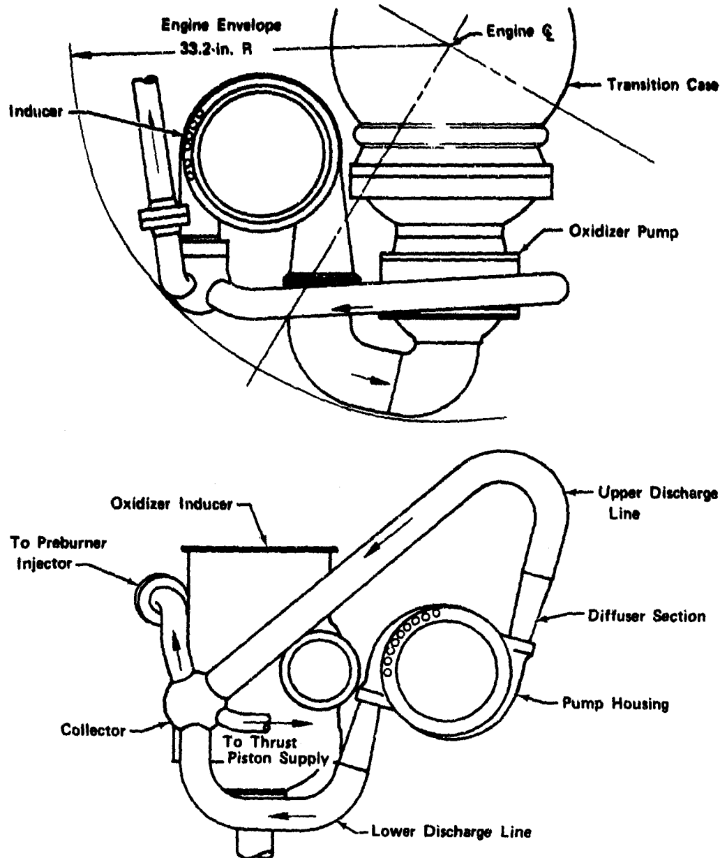
(U) Figure 554. General Arrangement of Oxidizer Pump Discharge Lines With Oxidizer Low-Speed Inducer
