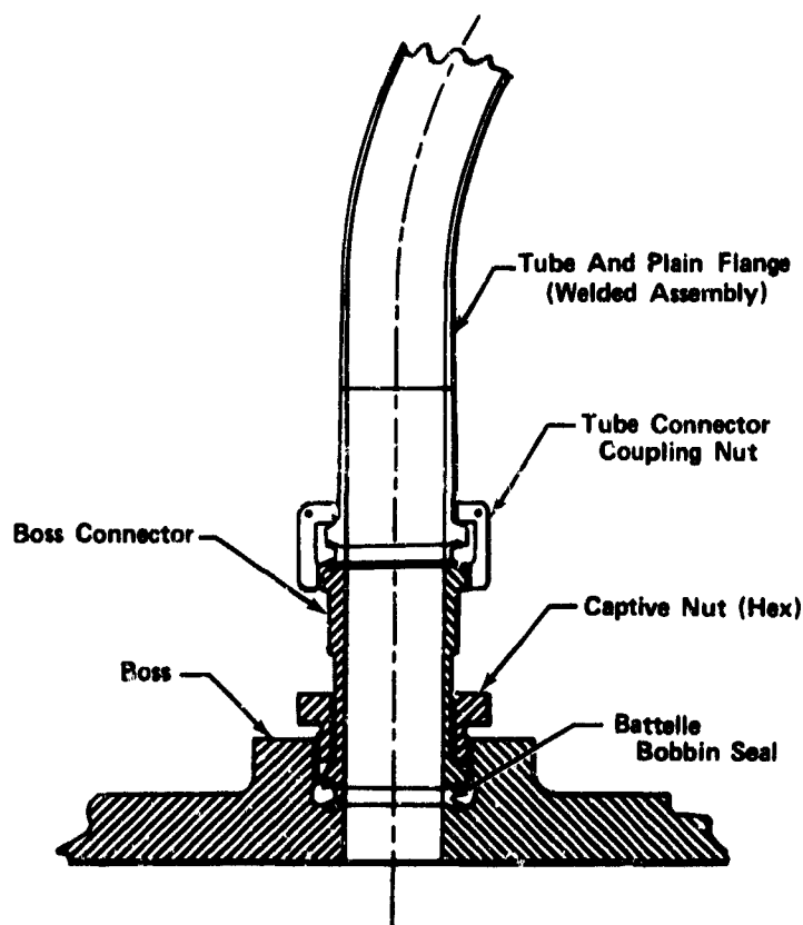
(U) Figure 564. Inconel 718 High Pressure Boss Connector
