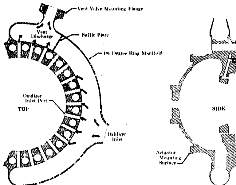
(U) Figure 423. Preburner Dome Cross Section
