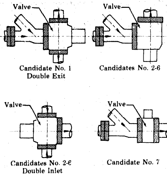
(U) Figure 466. Preburner Fuel Valve Installation Schematic
