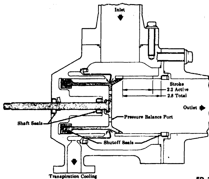
(U) Figure 447. Internal Sleeve Valve (Fixed Ports) Candidate
