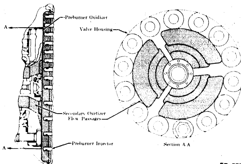
(U) Figure 424. Secondary Oxidizer Flow Passage
