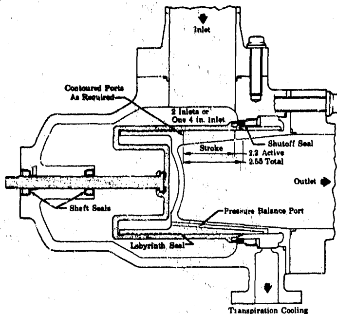
(U) Figure 446. External Sleeve Valve Candidate
