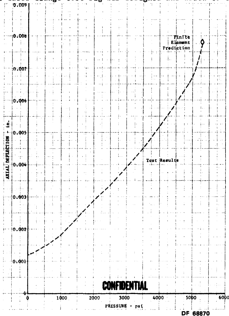
(U) Figure 537. Axial Deflection at ID of Flange, Rig 35120-3
