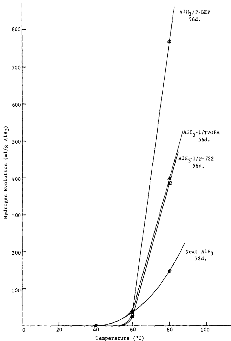
Figure VIII-4 - Hydrogen Evolved from \text{AlH}_3/\text{NF} Mixtures
