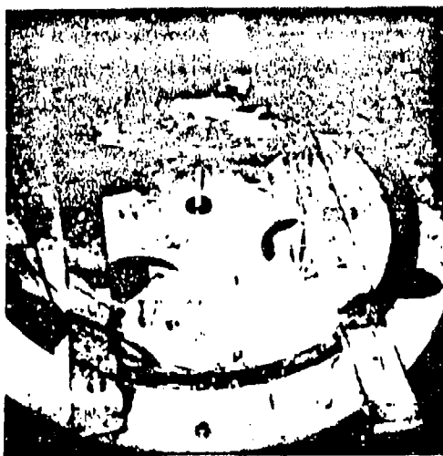
Figure 2-41. X404363-1 2 inch thick cylindrical chamber section. (U)
