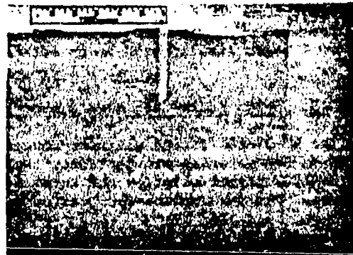
Figure B-15. MX-2600 Silica Phenolic Ablative Liner After Testing (U)
