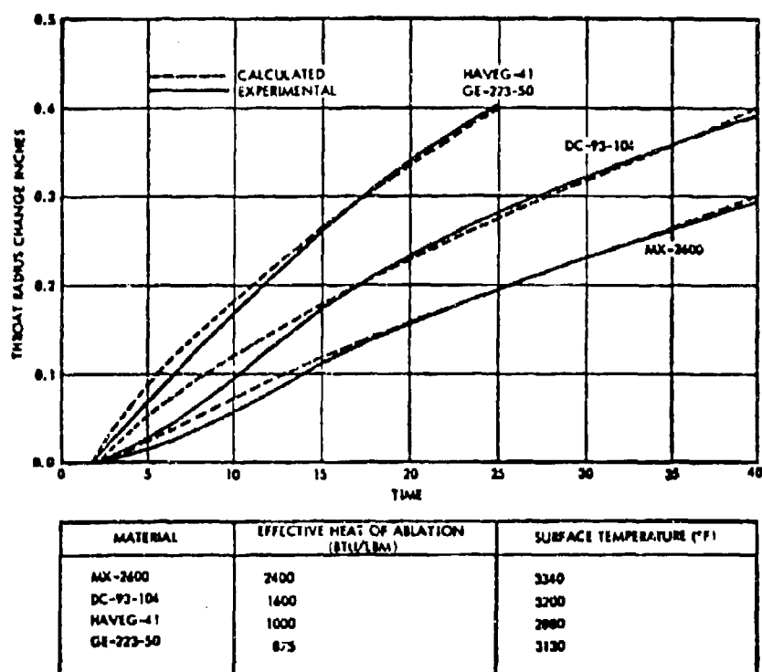
Figure C-5. Thermal Modeling of Erosion Characteristics of Four Candidate Low-Cost Ablative Liner Materials (U)
