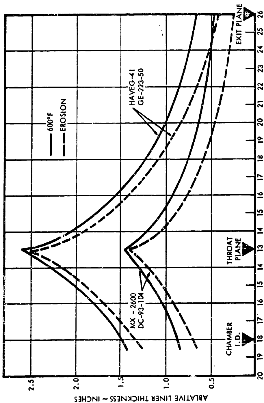
250 K LB F THRUST ENGINE INTERNAL RADIUS ~ INCHES Figure 2-5. 250,000 lbf Long-Duration Thrust Chamber Ablative Liner Thickness for Single 120-second Continuous Burn (Gas Recovery Temperature = 4850°F) (U)
