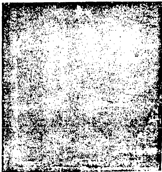
MXA-150 Oxidizer-Rich 300-Second Exposure (U) Figure B-65
