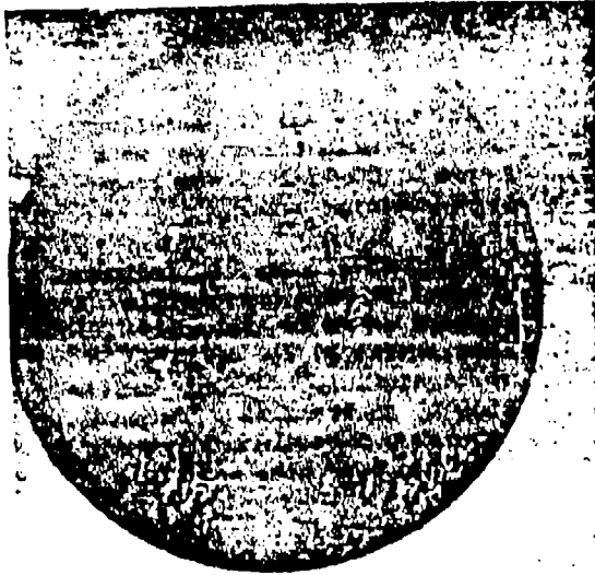
MX-2600 Oxidizer-Rich 60-Second Exposure (U) Figure B-45
