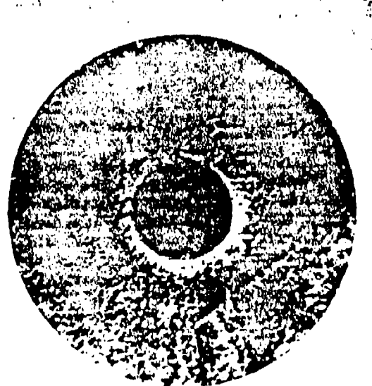
MX-2600 Fuel-Rich 60-Second Exposure (U) Figure B-46
