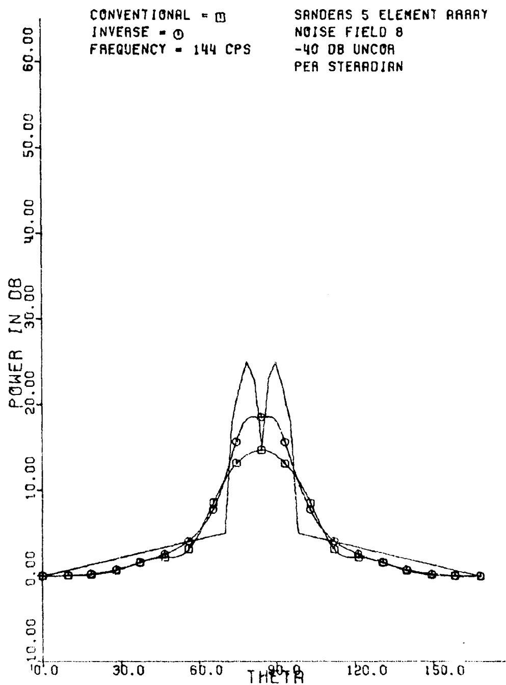
(U) Figure B57. BR noise field 8 144 cps.
