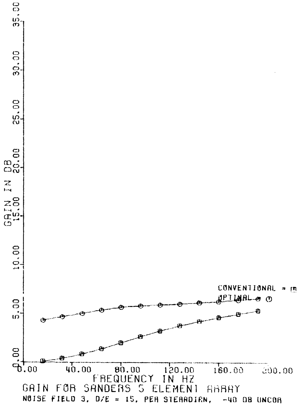
(U) Figure D16. Array gain - noise field 3 - D/E = 15.
