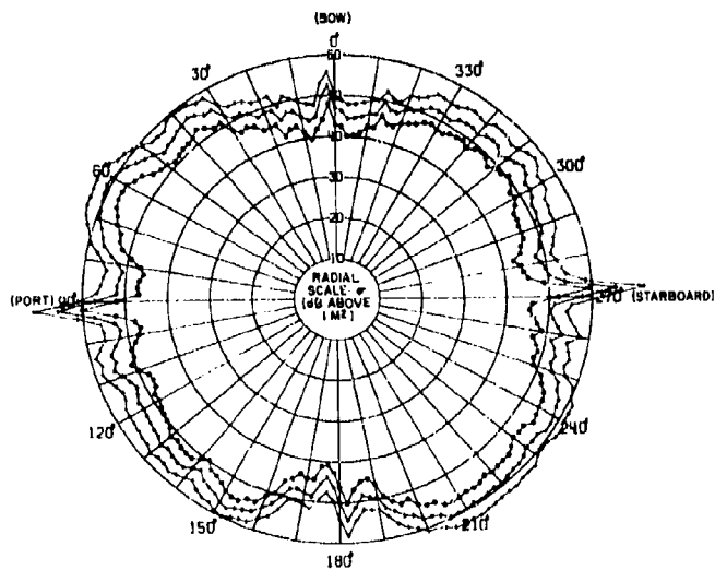
Fig. 45(C) - Radar cross section of the AFS 5 at 5500 MHz for vertical polarization
