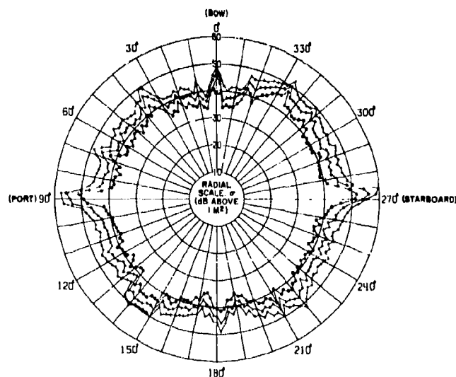
Fig. 13(C) - Radar cross section of the DDG 19 at 1300 MHz for horizontal polarization. Shown are the 20, 50, and 80 percentile values of the RCS distribution function denoted by a circle ( \circ ), a triangle ( \Delta ), and a cross (+) respectively.
