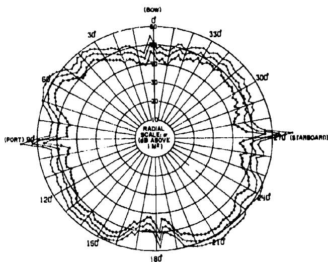
Fig. 44(C) - Radar cross section of the AFS 5 at 5500 MHz for horizontal polarization
