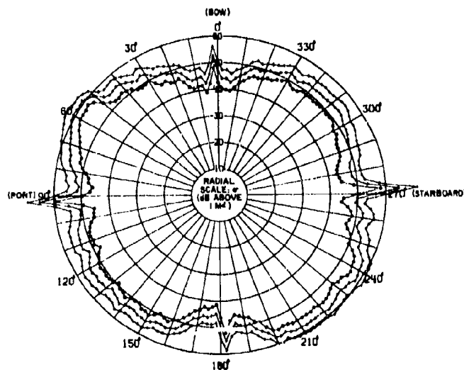
Fig. 43(C) - Radar cross section of the AFS 5 at 9225 MHz for vertical polarization
