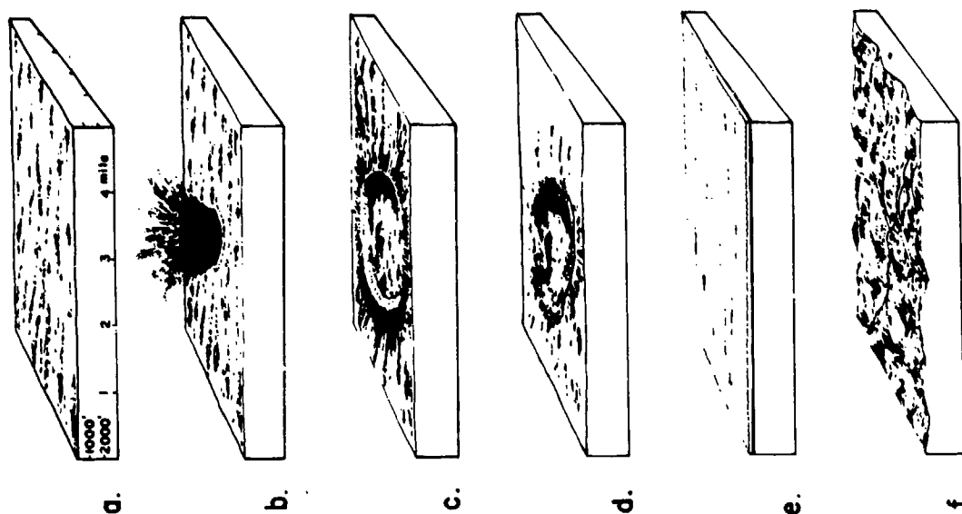
Figure 13c. Diagrammatic sequence of events during formation and subsequent history of the Flynn Creek crater.
