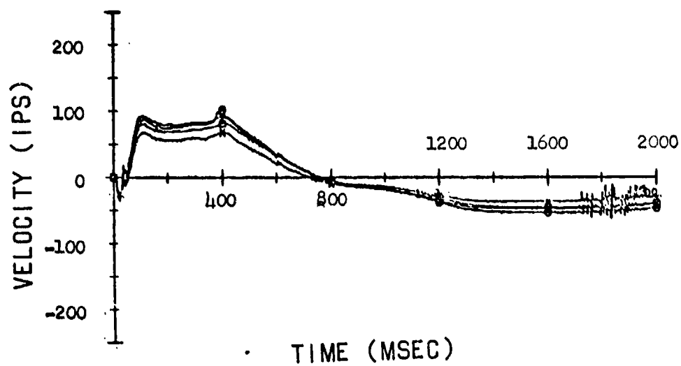
Figure 5 (U) Airblast induced vertical silo velocities (U).
