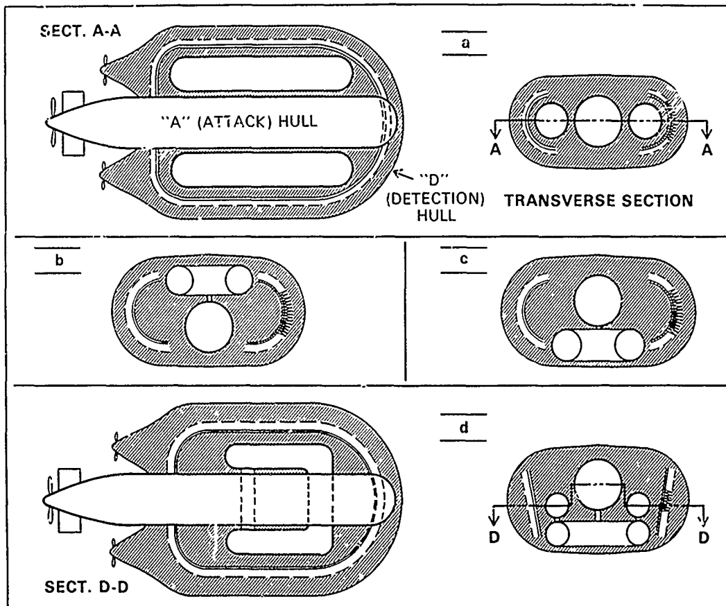
Fig. 2. Candidate ADA submarine configurations.
