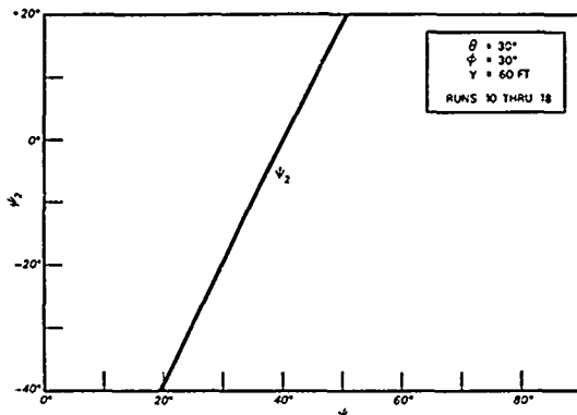
Fig. 23. Solution of docking impact equations — angle of "A" hull after impact vs. angle of hull before impact.
