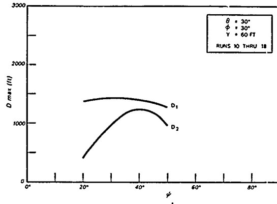
Fig. 20. Solution of docking impact equations — deflection of shock mitigator vs. entrance angle.
