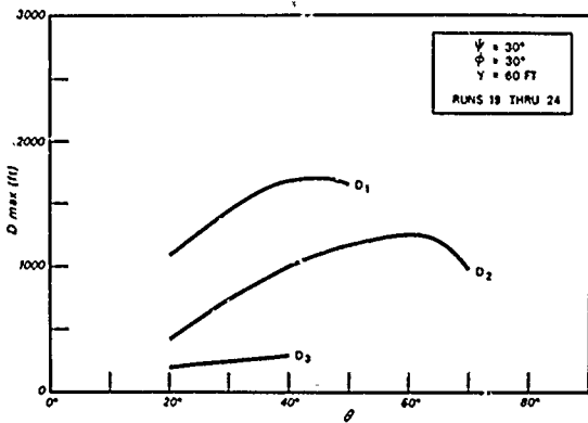
Fig. 19. Solution of docking impact equations — deflection of shock mitigator vs. angle of "A" hull.
