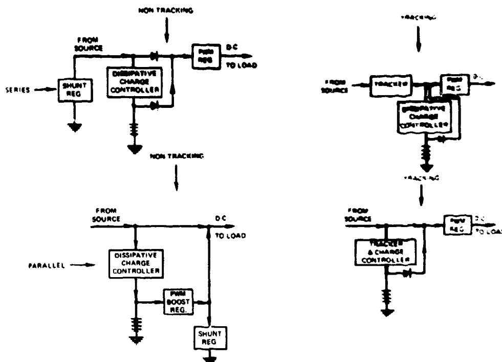
Fig. 4-21 - Comparison of power subsystems
