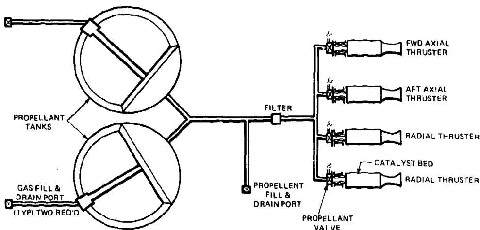
Fig. 4-26 - Functional schematic diagram of the propulsion subsystem
