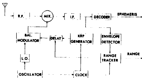
Fig. 3-30 - KRP receiver block diagram
