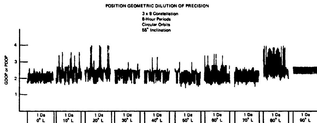
Fig. A-4 - Position geometric dilution of precision for the 3-by-9 constellation using 8-hr periods and circular orbits at a 55-degree inclination
