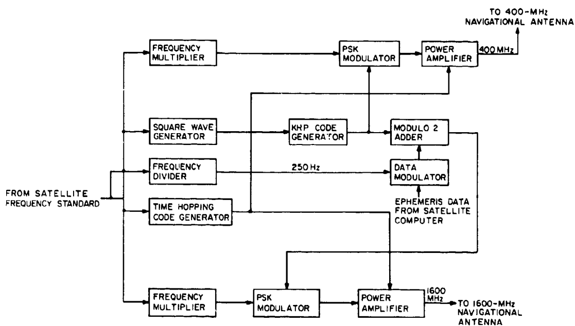
Fig. 4-14 - Satellite KRP L-band transmitter
