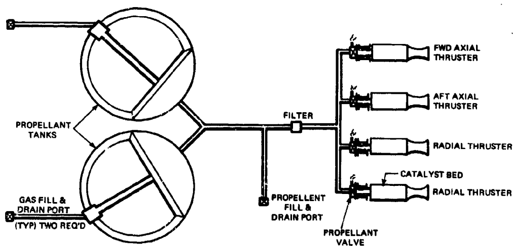
Fig. 3-18 - Propulsion subsystem diagram
