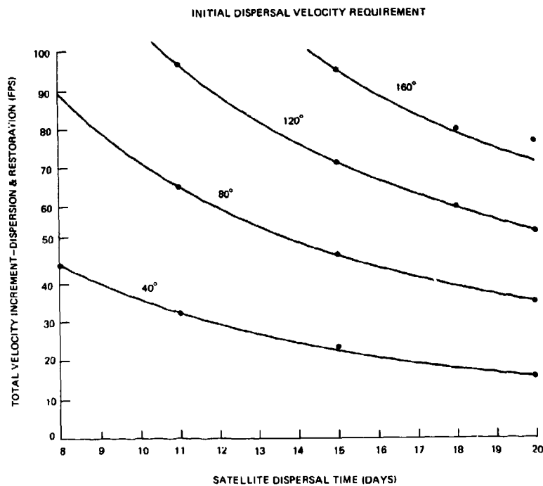
Fig. 4-7 - Timation satellite system initial dispersal velocity requirement
