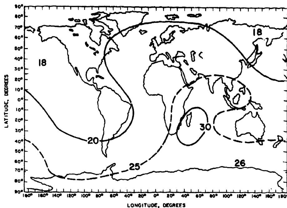
Fig. 1-4 - Error contours (in feet) for a user with a good clock for a 3-by-9, 8-hr, 55-degree constellation
