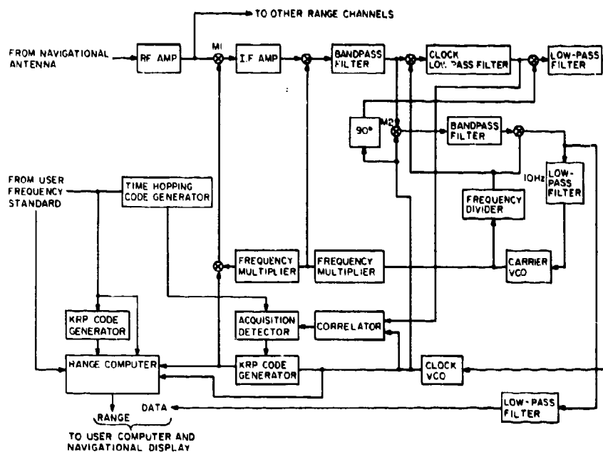
Fig. 4-33 - Block diagram of the 1600-MHz KRP receiver
