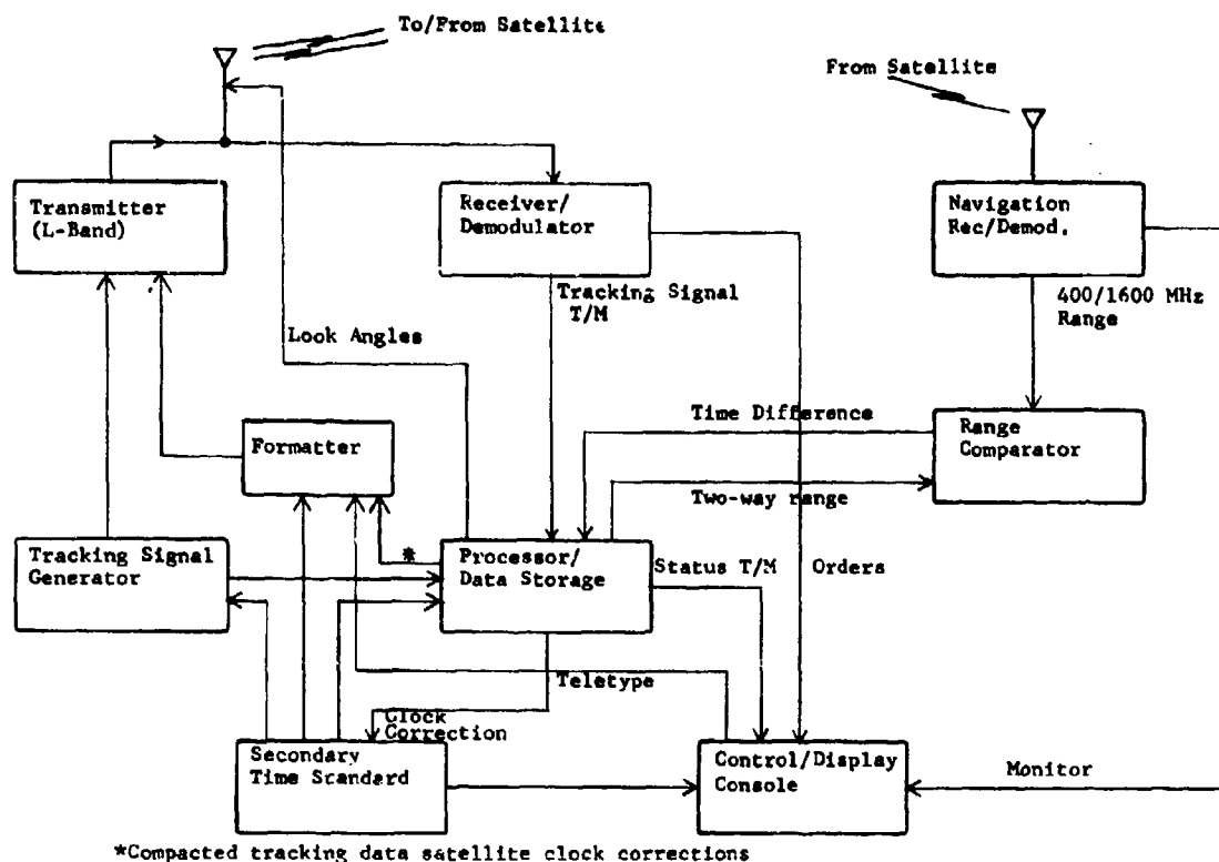
Fig. 3-20 - RGS functional block diagram
