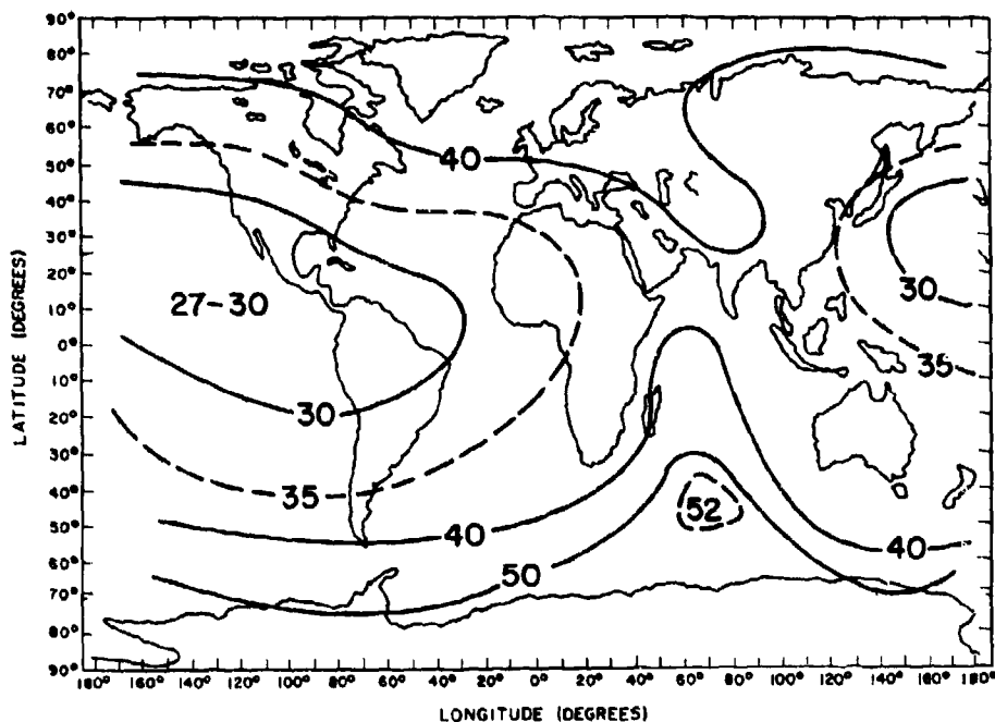
Fig. 4-4 - Typical position fix errors for 3 x 9 inclined orbit constellation using four ground stations
