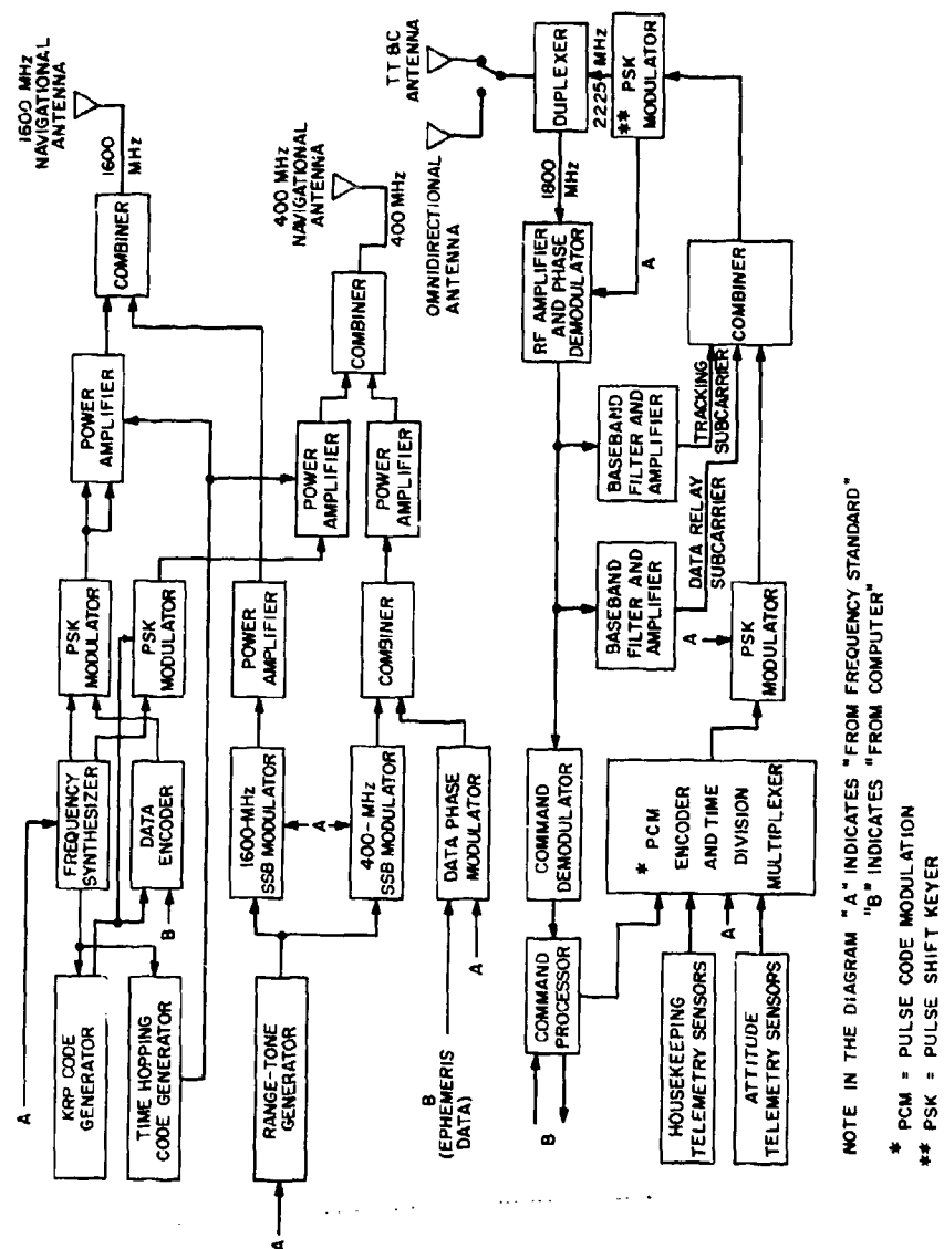
Fig. 3-15 - Data package block diagram
