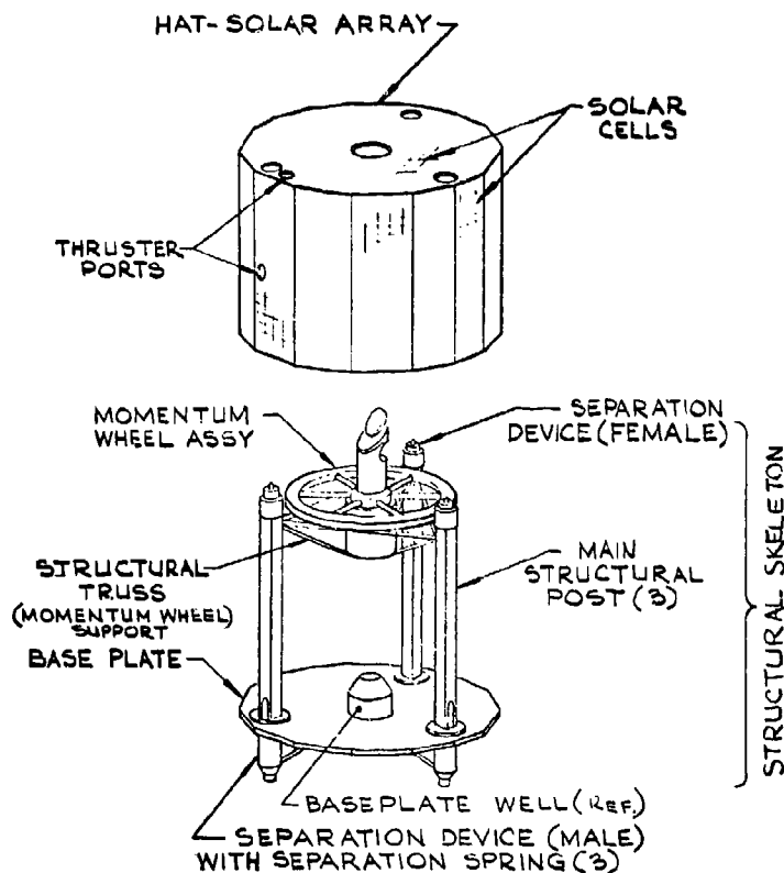
Fig. 4-8 - Timation satellite (main structural components)
