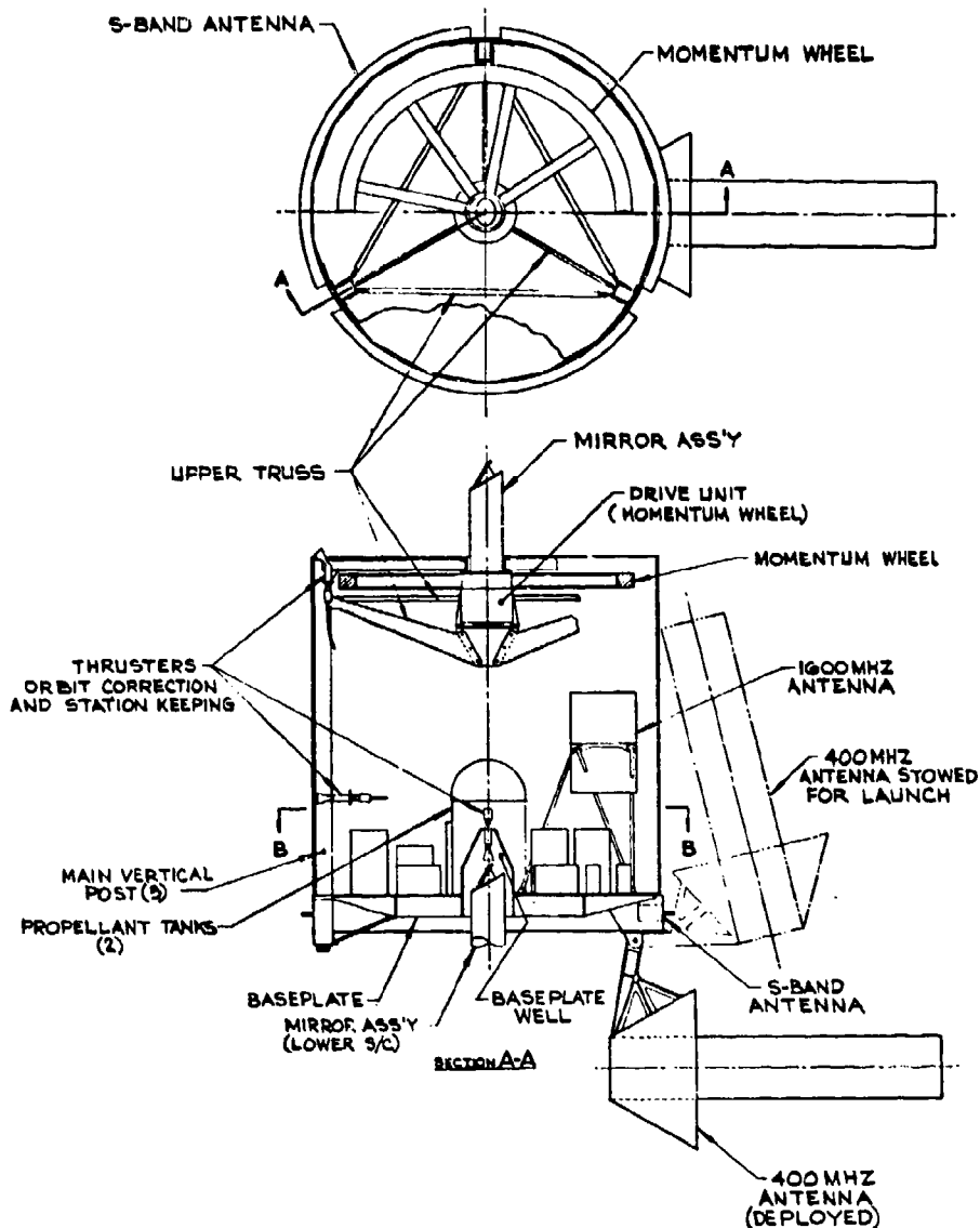
Fig. 3-12 - Spacecraft mechanical configuration
