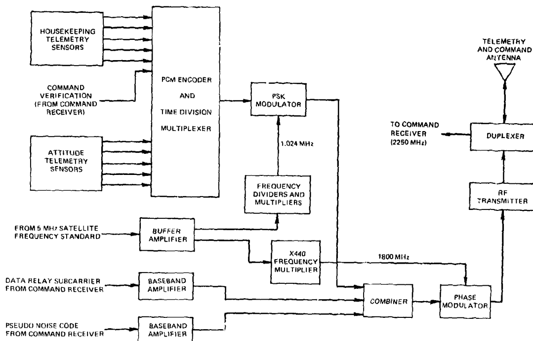
Fig. 4-17 - Timation satellite (telemetry encoder and transmitter)
