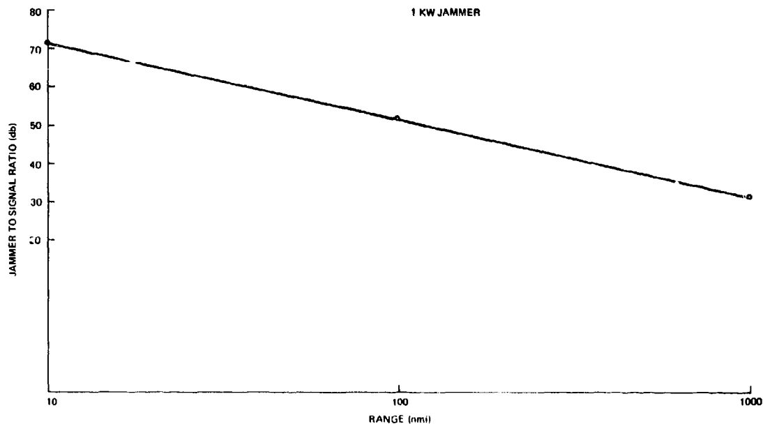
Fig. 3-7 - Jammer power vs jammer-to-user distance
