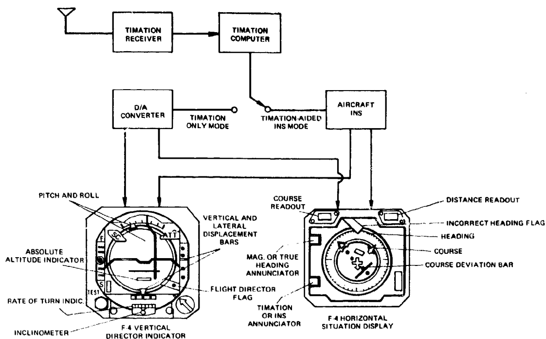
Fig. 3-31 - Display implementation for category 1 user
