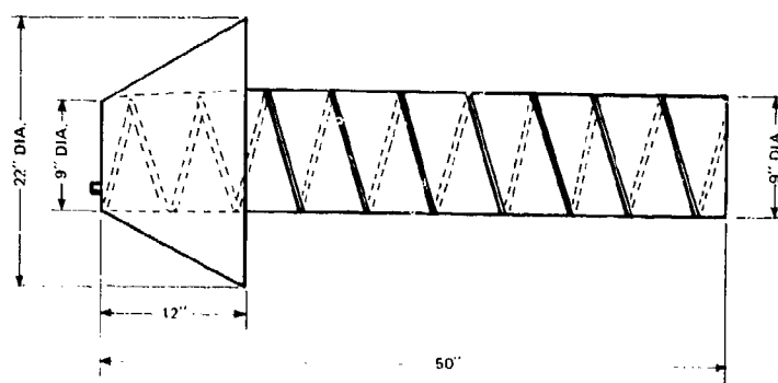
Fig. 4-12 - 400-MHz navigation links (antenna design)
