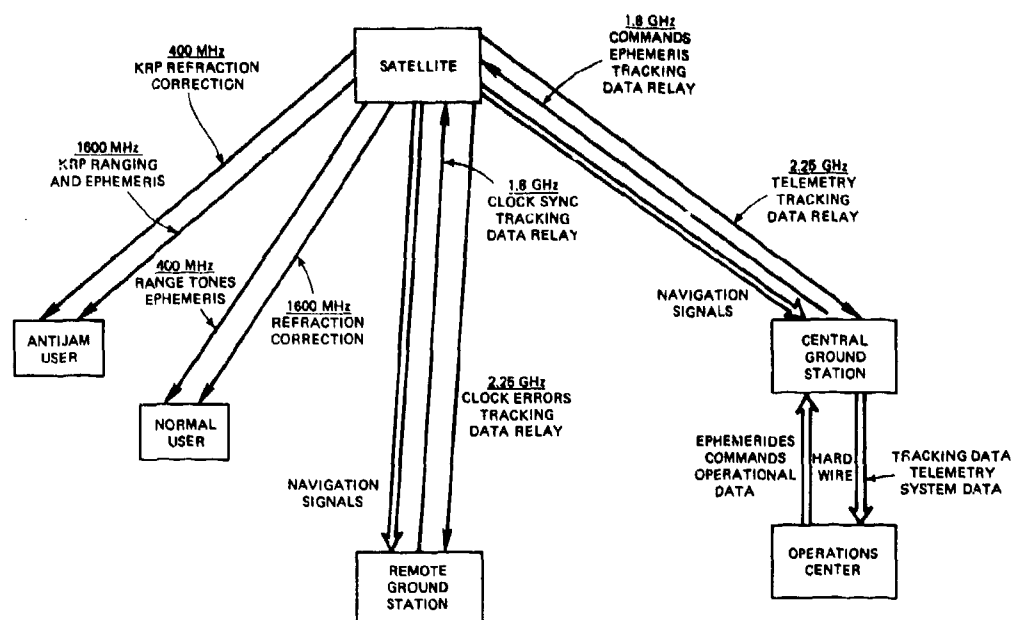
Fig. 3-6 - Timation data links
