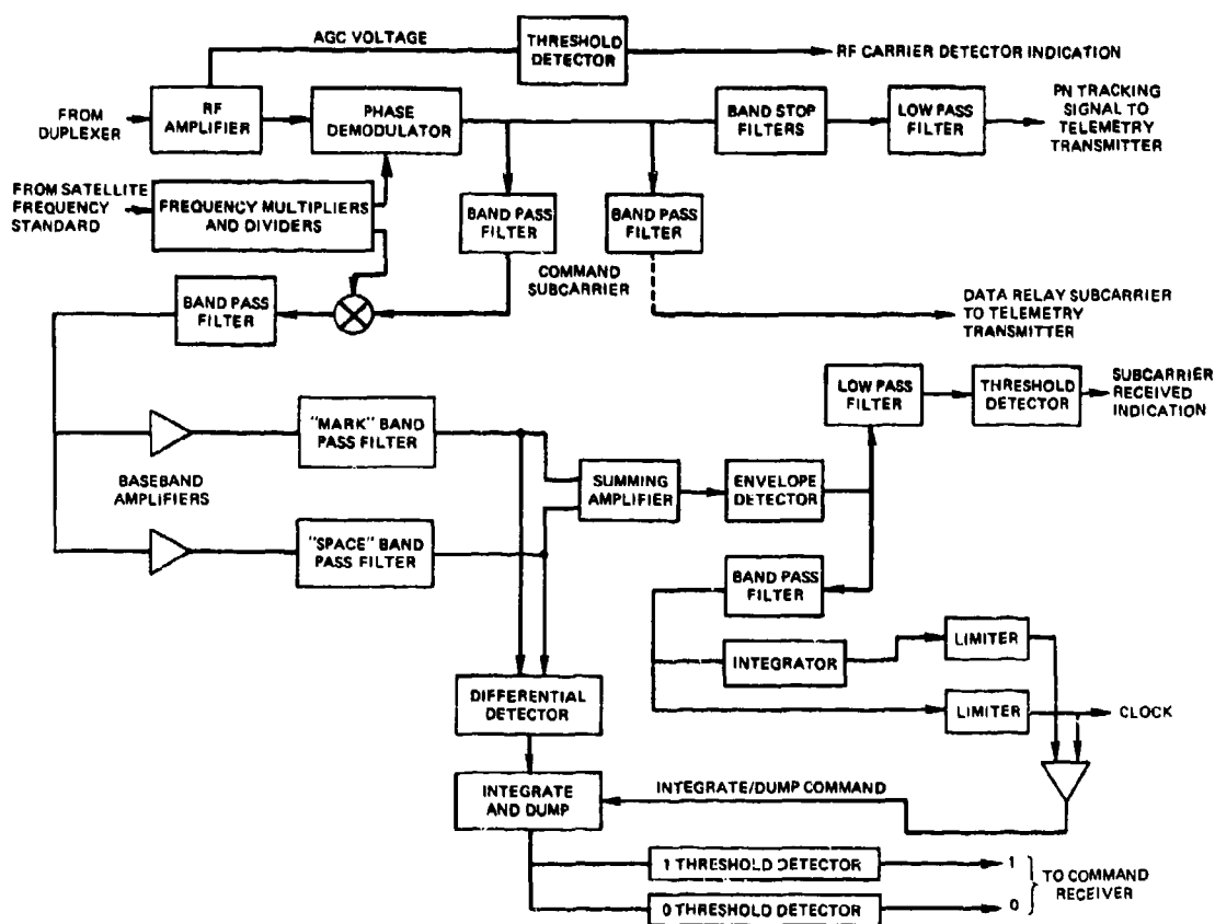
Fig. 4-19 - Timation satellite command demodulator
