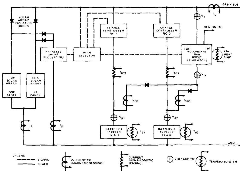
Fig. 4-22 - Functional block diagram of the power subsystem
