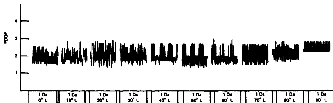
Fig. A-5 - Position geometric dilution of precision for the 3-by-9 constellation using 12-hr periods and circular orbits at a 53-degree inclination
