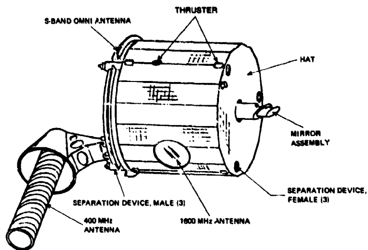
Fig. 3-3 - Spacecraft orbital configuration
