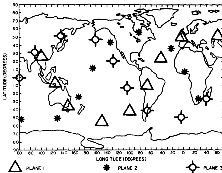
Fig. 3-2 - 27-satellite constellation and ground tracks
