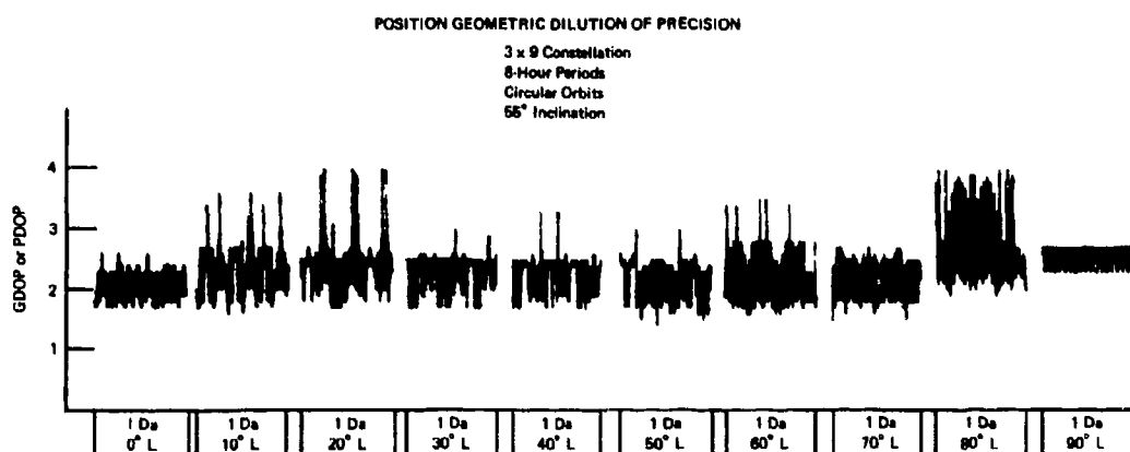
Fig. 3-10 - Position geometric dilution of precision
