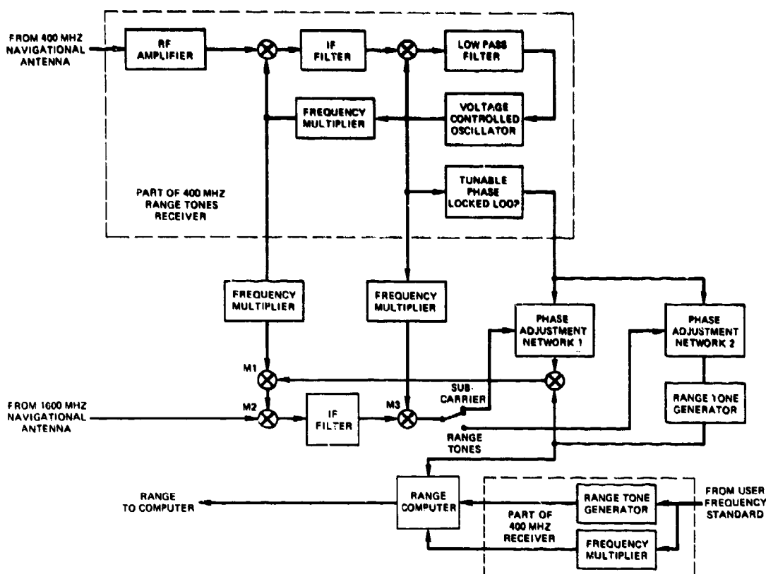
Fig. 4-32 - Block diagram of the 1600-MHz range-tone receiver
