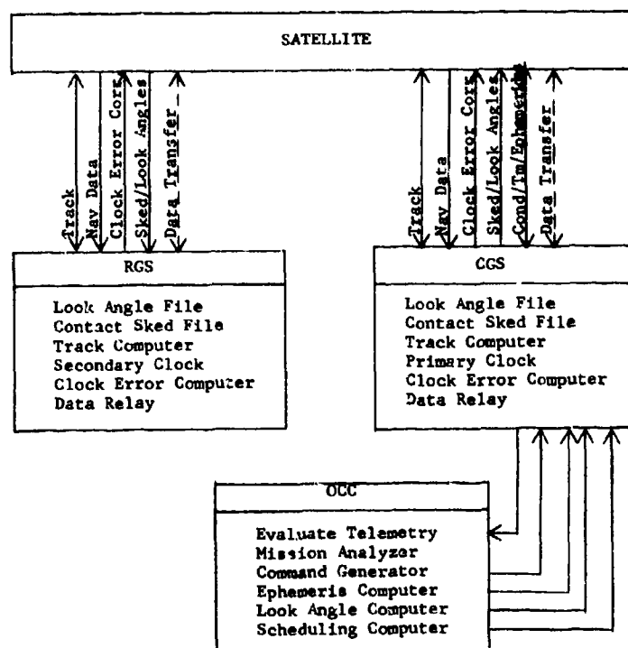
Fig. 3-19 - Ground station complex functional flow diagram
