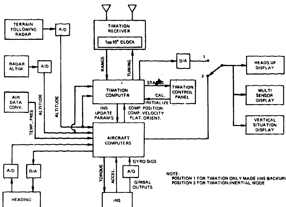
Fig. 4-34 - Signal flow diagram of the category 1 user equipment
