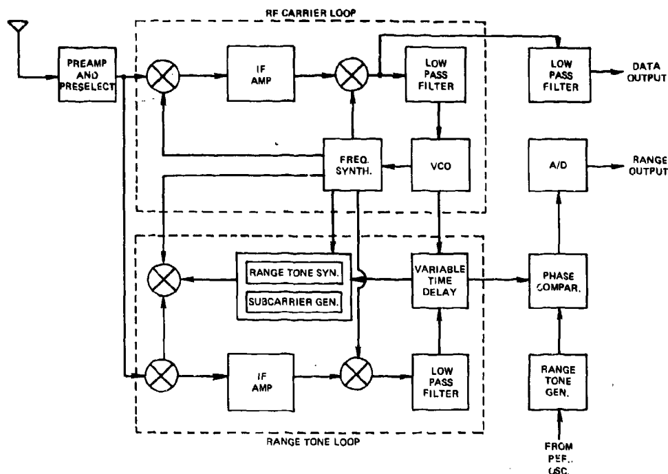
Fig. 3-29 - Range-tone receiver block diagram
