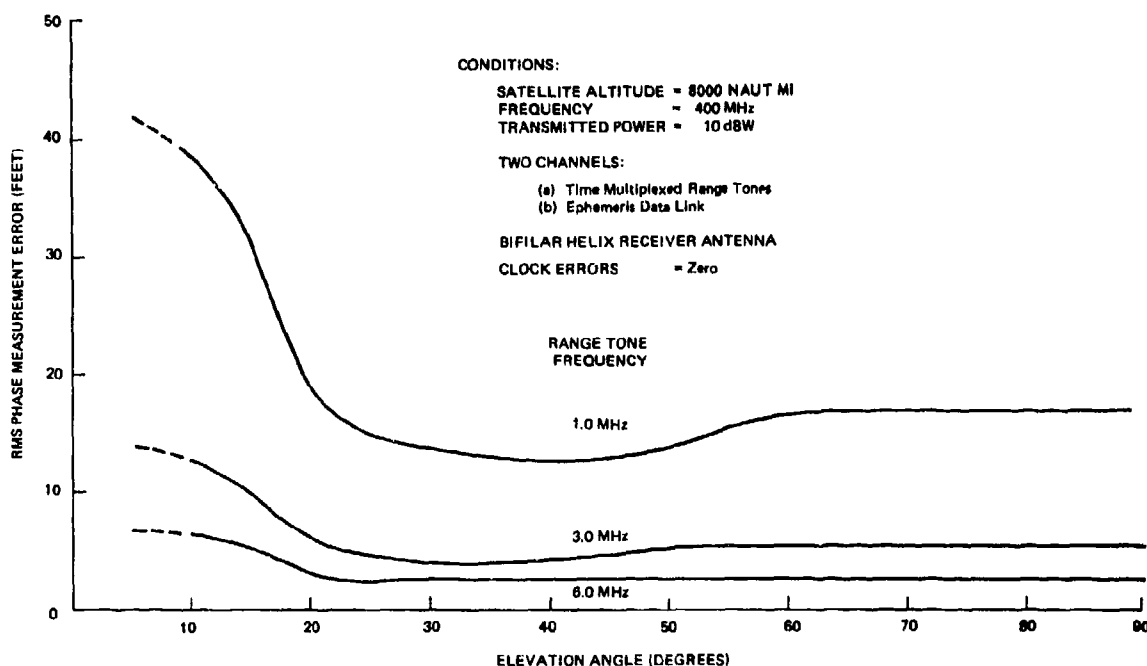
Fig. 4-5 - Range error due to phase measurement error
