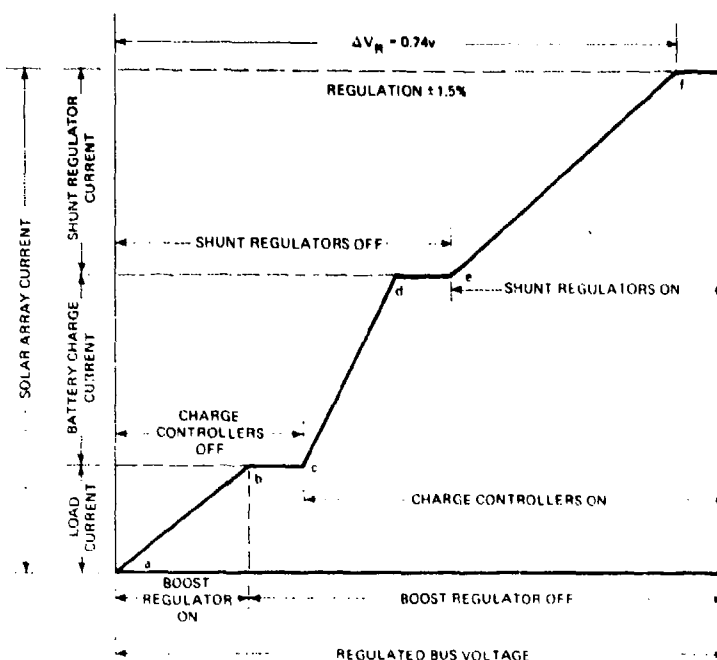
Fig. 4-23 - Mode selector operation (bus voltage profile)
