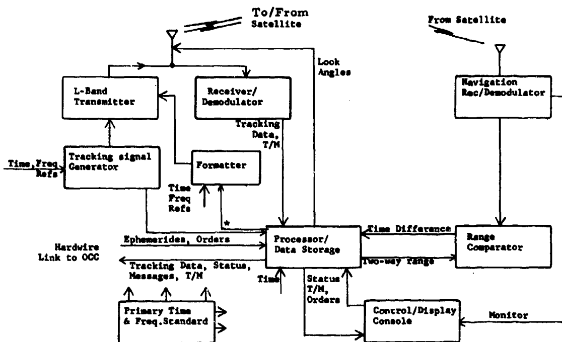
Fig. 3-21 - CGS functional block diagram
