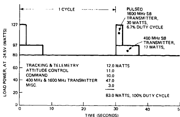
Fig. 4-20 - Load power profile
