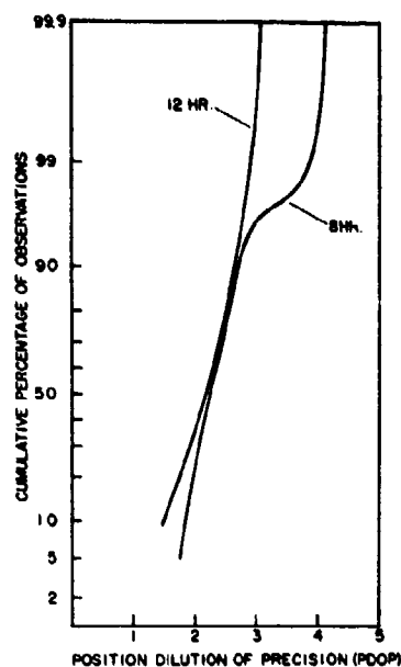
Fig. A-3 - PDOP comparisons of 8-hr and 12-hr orbits using 3-by-9 constellations, 10-degree masks, 53-degree inclination for the 12-hr orbit, and 55-degree inclination for the 8-hr orbit
