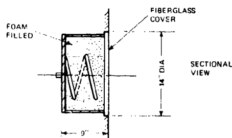
Fig. 4-13 - 1600-MHz navigation links (antenna design)
