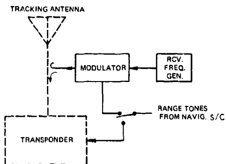
Fig. 4-15 - Satellite transponder
