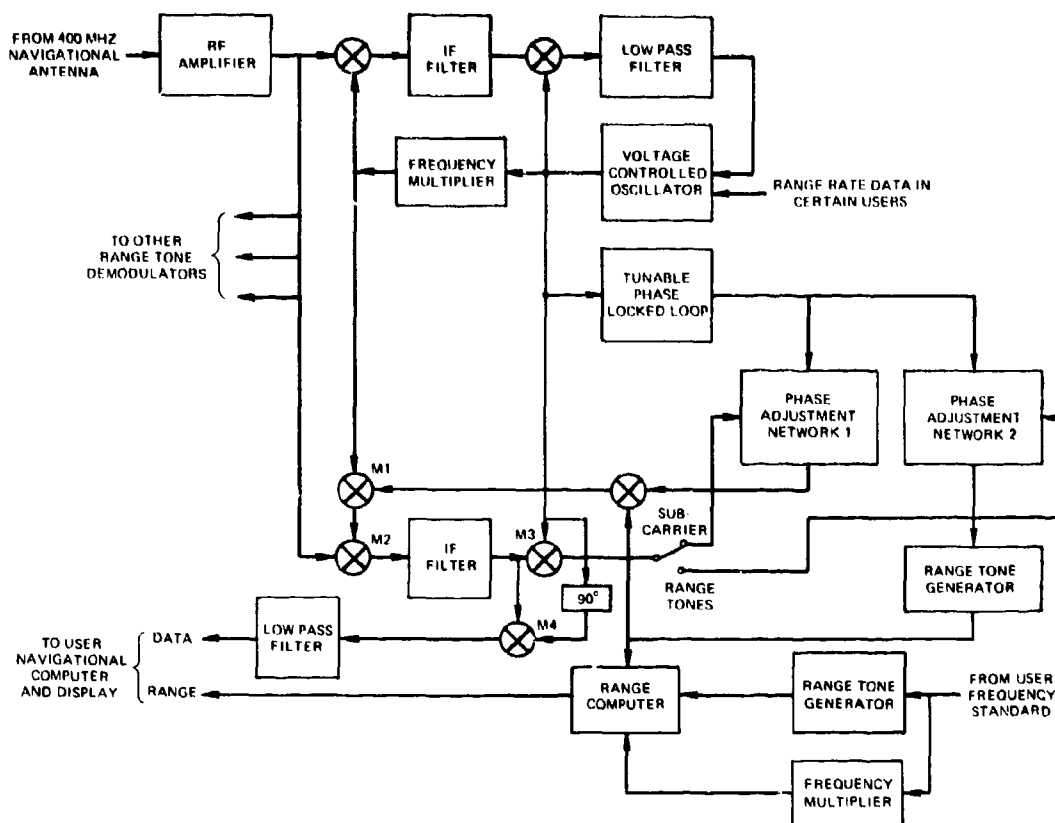
Fig. 4-31 - Block diagram for the 400-MHz range-tone receiver
