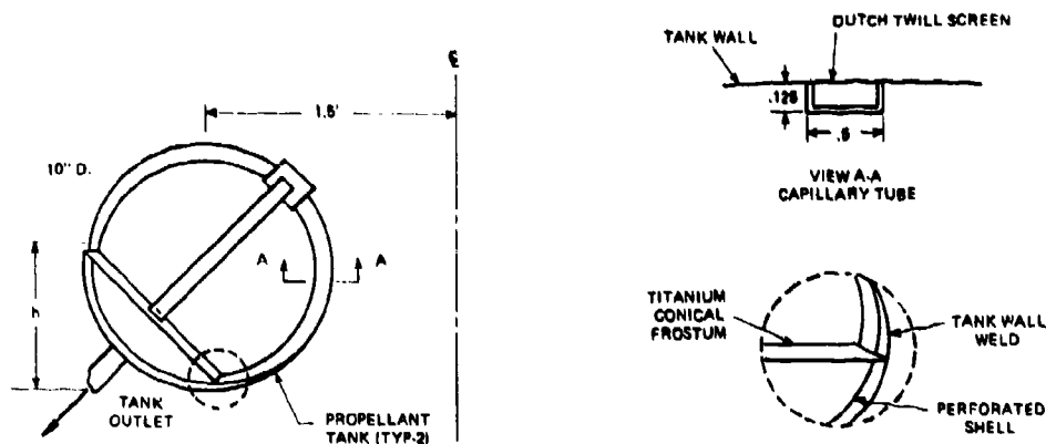
Fig. 4-27 - Capillary propellant-management tank
