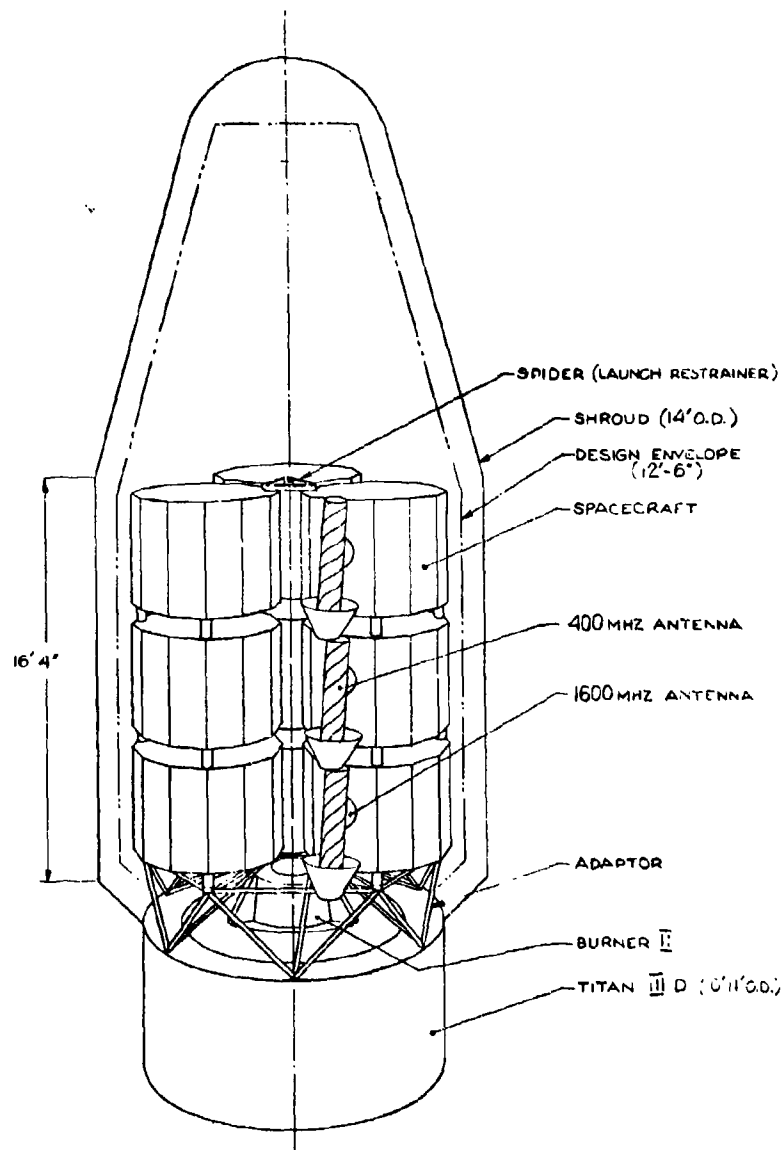
Fig. 3-14 - Nine-satellite launch configuration
