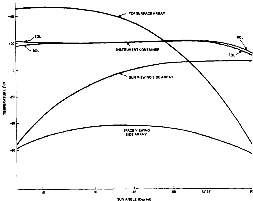
Fig. 4-24 - Steady-state temperature during spacecraft daylight
