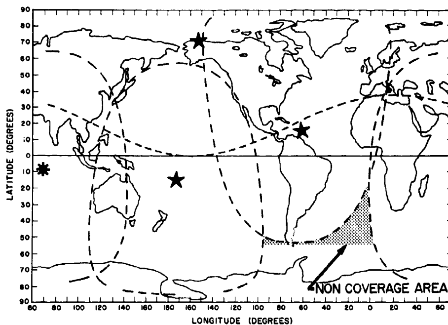
Fig. A-2 - Station coverage and noncoverage for locations shown and for 12-hr, 53-degree inclination orbits
