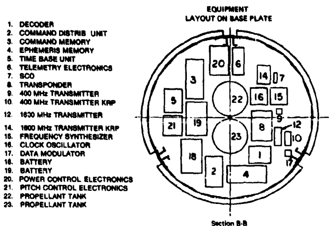
Fig. 3-13 - Spacecraft component layout
