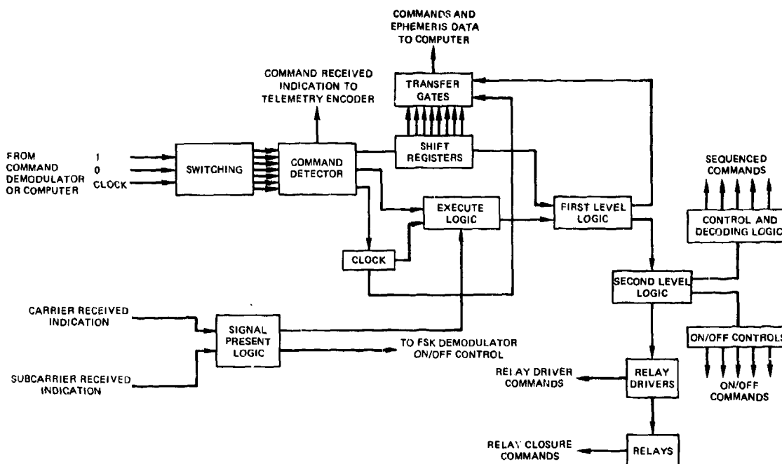
Fig. 4-18 - Timation satellite command receiver
