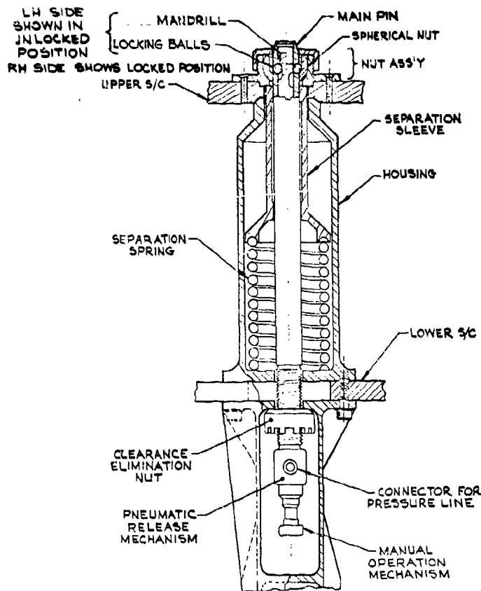
Fig. 4-9 - "Ball-pin" separation device
