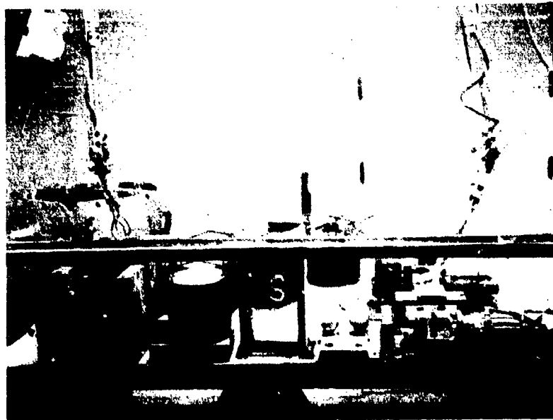
Fig. 3. - Filling Operation. A mechanical hand picks up the muniton from a rack, places it in a hydraulic clamp (the dark object on the table in the foreground on the extreme right), and screws the pellet tube onto a short transparent plastic nipple that fits into the muniton. The muniton is then lifted onto a vibrator, which shakes the pellets from the tube. The filled muniton is then placed again in the hydraulic clamp. The tube and the nipple are removed, and a cap is screwed into the opening of the muniton.
