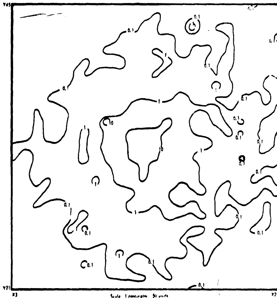
Fig. 8a. - Isointensity contours at the three-foot level showing gamma radiation in milliroentgens per hour for Munition 12.
