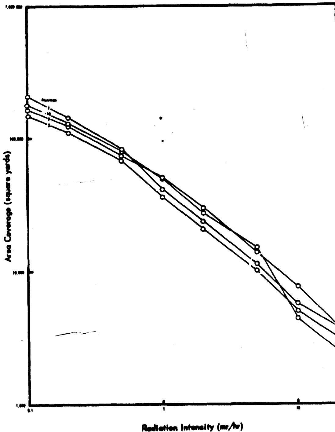
Fig. 6b - Area coverage versus target radiation intensity. Scheduled opening altitude - 2,000 feet.
