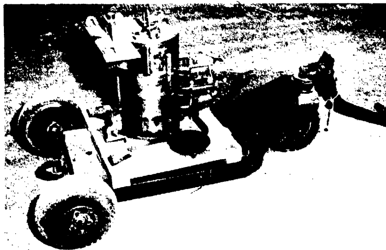
Fig. 3. - Filling Operation. A mechanical hand picks up the muniton from a rack, places it in a hydraulic clamp (the dark object on the table in the foreground on the extreme right), and screws the pellet tube onto a short transparent plastic nipple that fits into the muniton. The muniton is then lifted onto a vibrator, which shakes the pellets from the tube. The filled muniton is then placed again in the hydraulic clamp. The tube and the nipple are removed, and a cap is screwed into the opening of the muniton.
