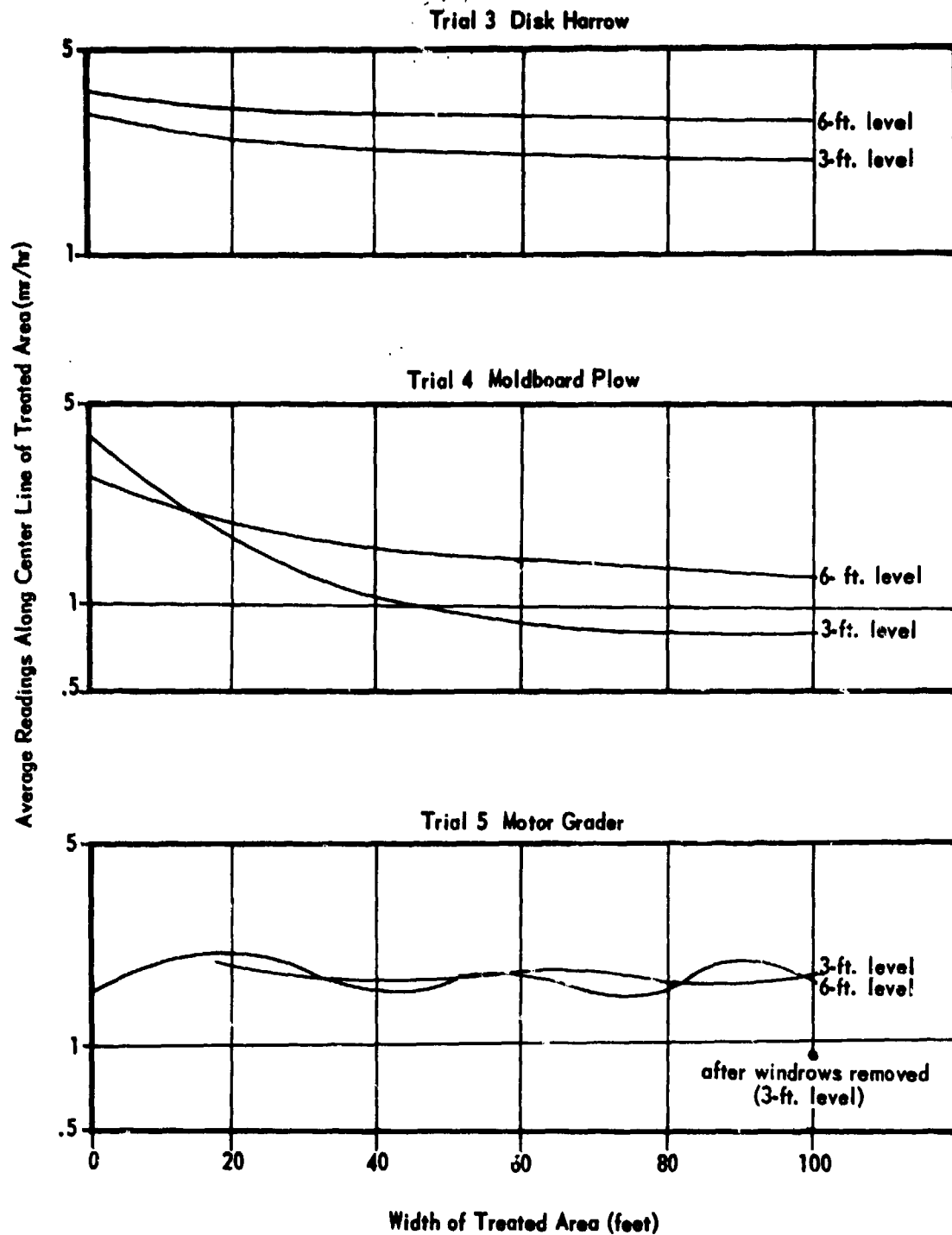
Figs. 11, 12, and 13. - Center-line intensity versus width of decontaminated area.
