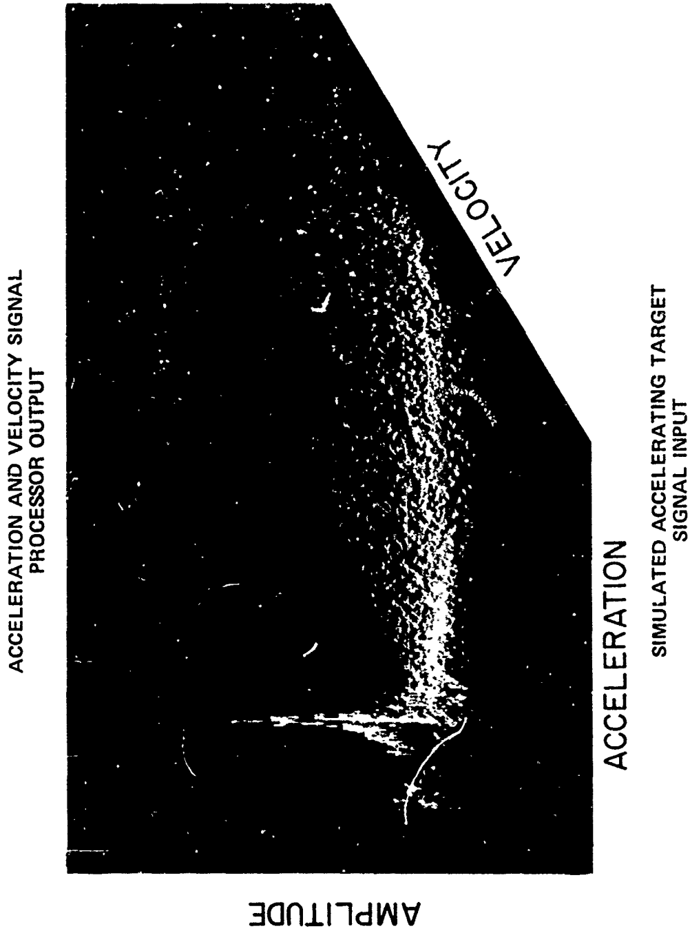
Fig. 16--(S) AVR signal processor output with the target signals of Fig. 14. The lowest 1.0% of the acceleration cells were not processed, thus increasing the mismatch and further suppressing the constant-velocity target.
